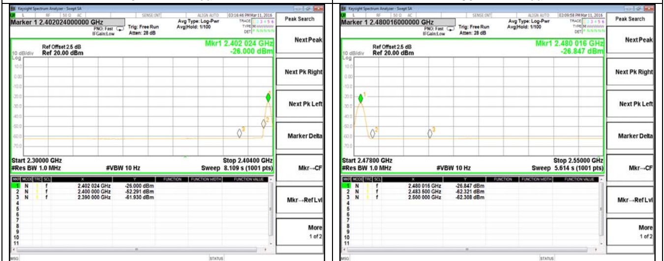
2402 MHz – Average
