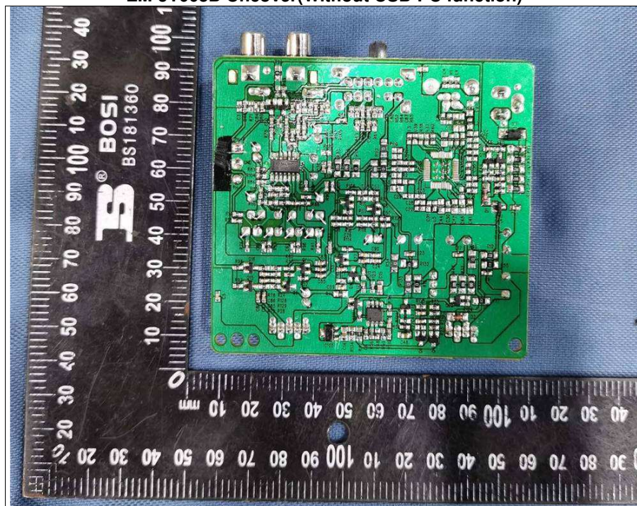
EM-JT003B Uncover(Without USB-PC function)
