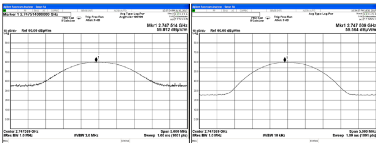
Plot 7.7.24 Radiated emission measurements at the third harmonic of mid carrier frequency
