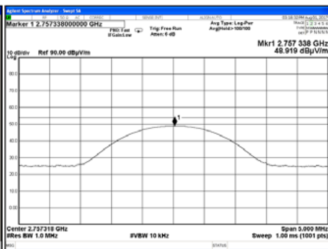
Plot 7.7.26 Radiated emission measurements at the third harmonic of high carrier frequency
