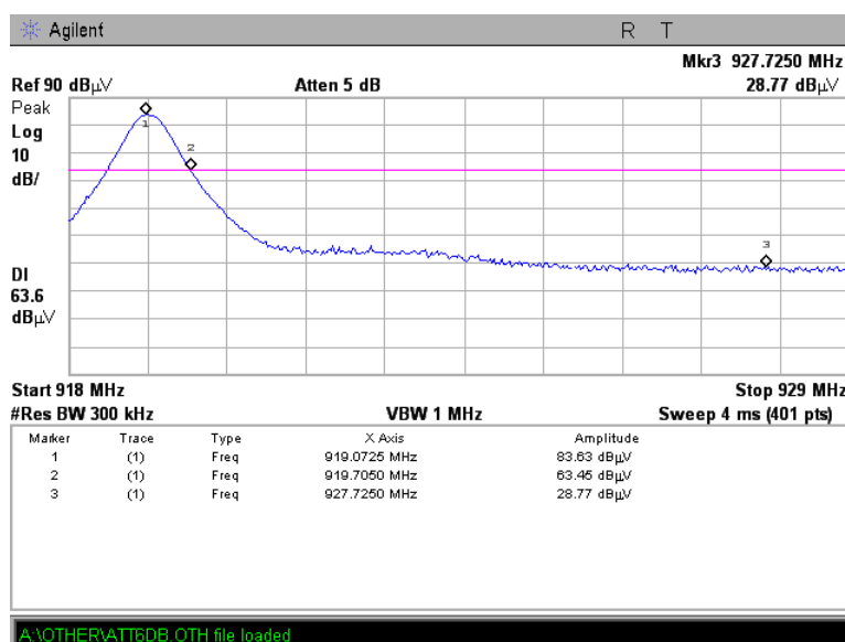
Plot 7.6.2 The highest band edge emission at high carrier frequency with hopping function disabled
