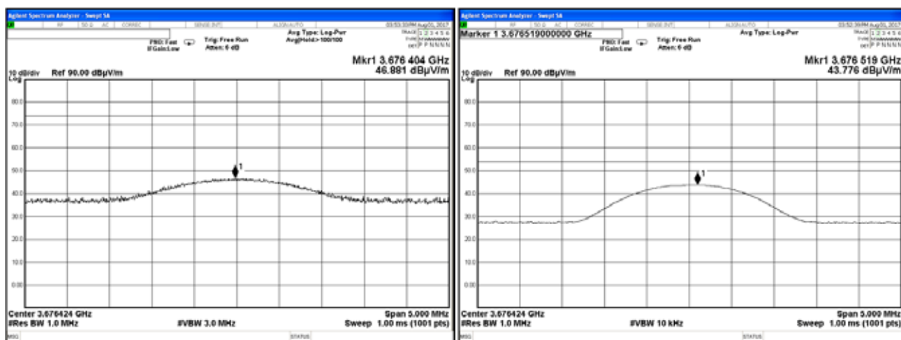
Plot 7.7.32 Radiated emission measurements at the fourth harmonic of high carrier frequency
