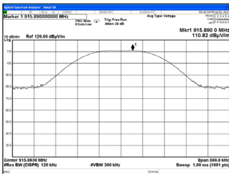
Plot 7.5.8 Field strength of carrier at mid frequency and Unom
