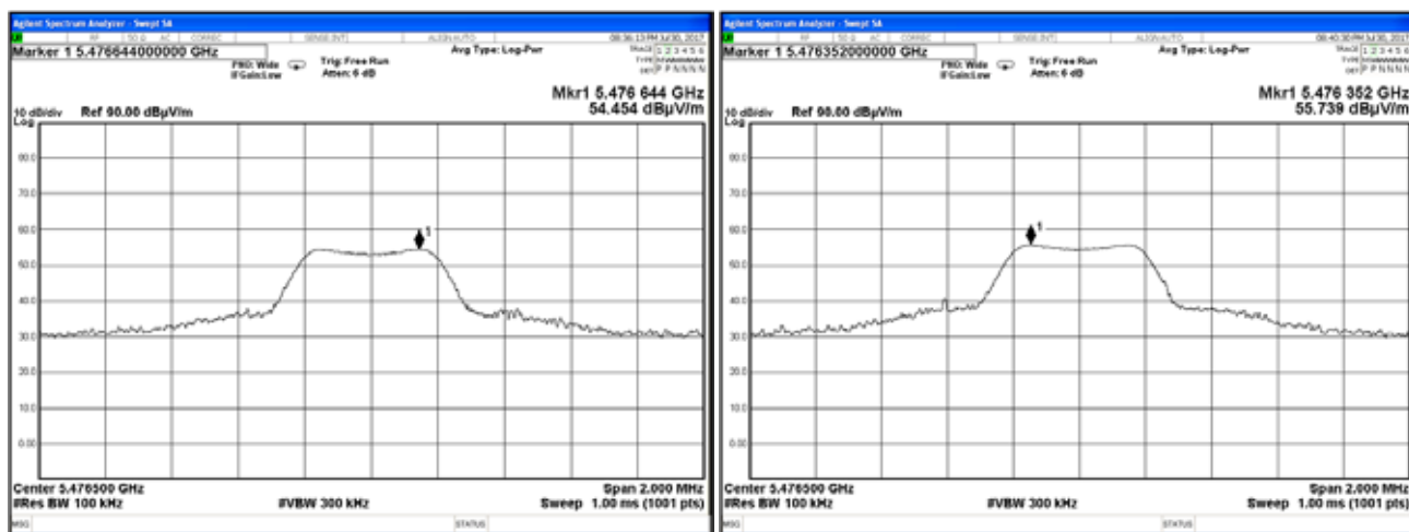
Plot 7.7.40 Radiated emission measurements at the sixth harmonic of mid carrier frequency
