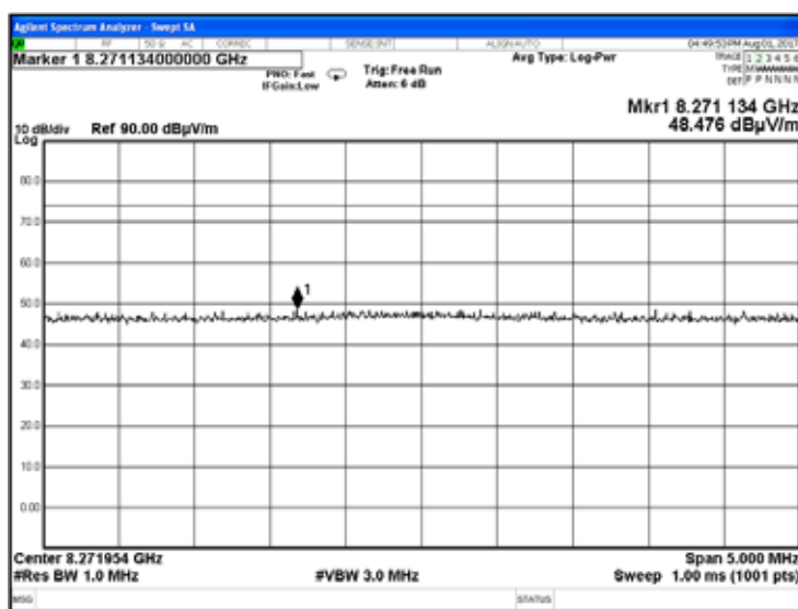
Plot 7.7.56 Radiated emission measurements at the ninth harmonic of high carrier frequency
