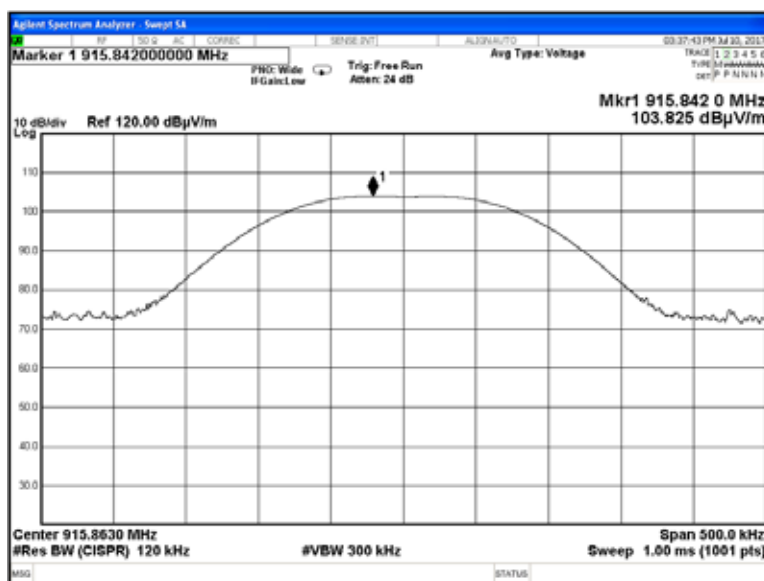
Plot 7.5.12 Field strength of carrier at mid frequency and Unom
