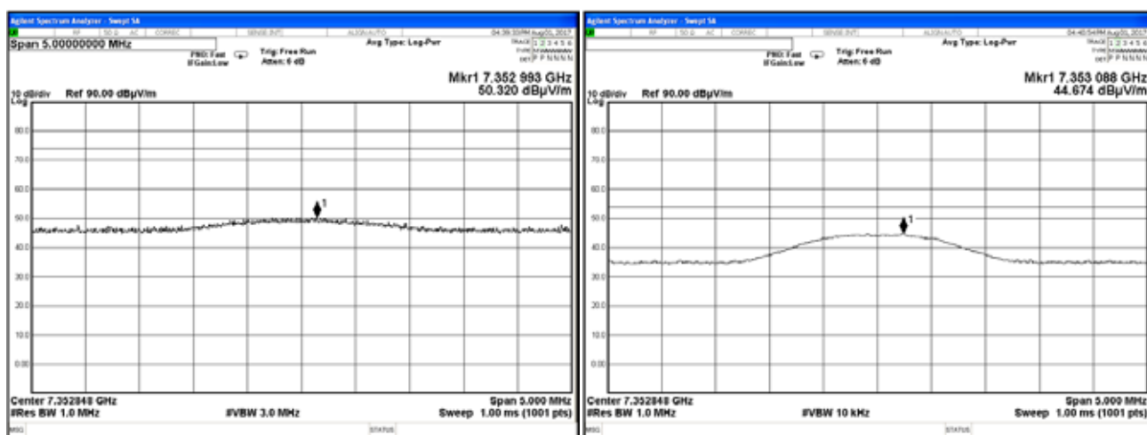
Plot 7.7.50 Radiated emission measurements at the eighth harmonic of high carrier frequency
