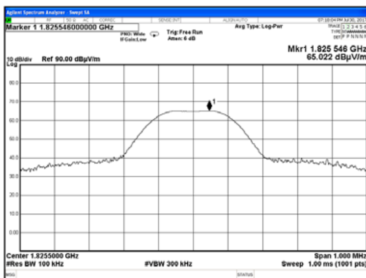
Plot 7.7.16 Radiated emission measurements at the second harmonic of low carrier frequency
