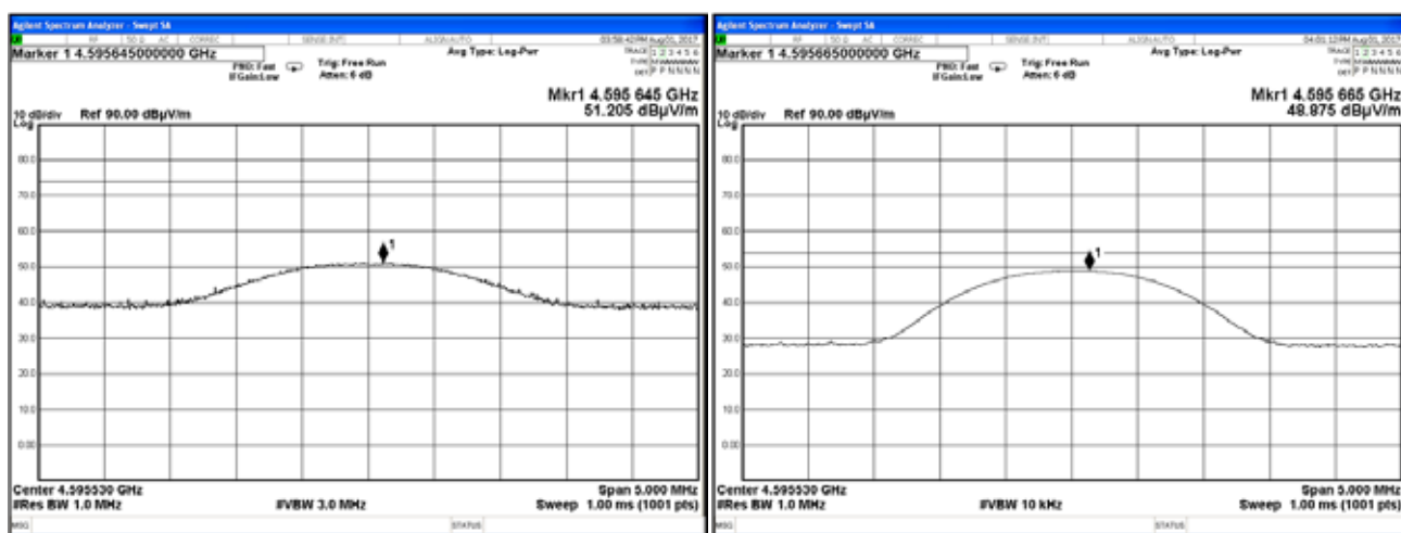
Plot 7.7.38 Radiated emission measurements at the fifth harmonic of high carrier frequency
