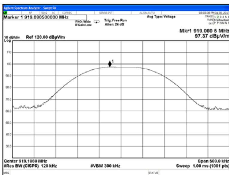
Plot 7.5.16 Field strength of carrier at high frequency and Unom
