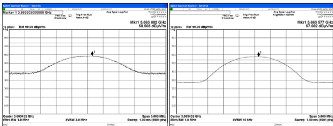
Plot 7.7.30 Radiated emission measurements at the fourth harmonic of low carrier frequency
