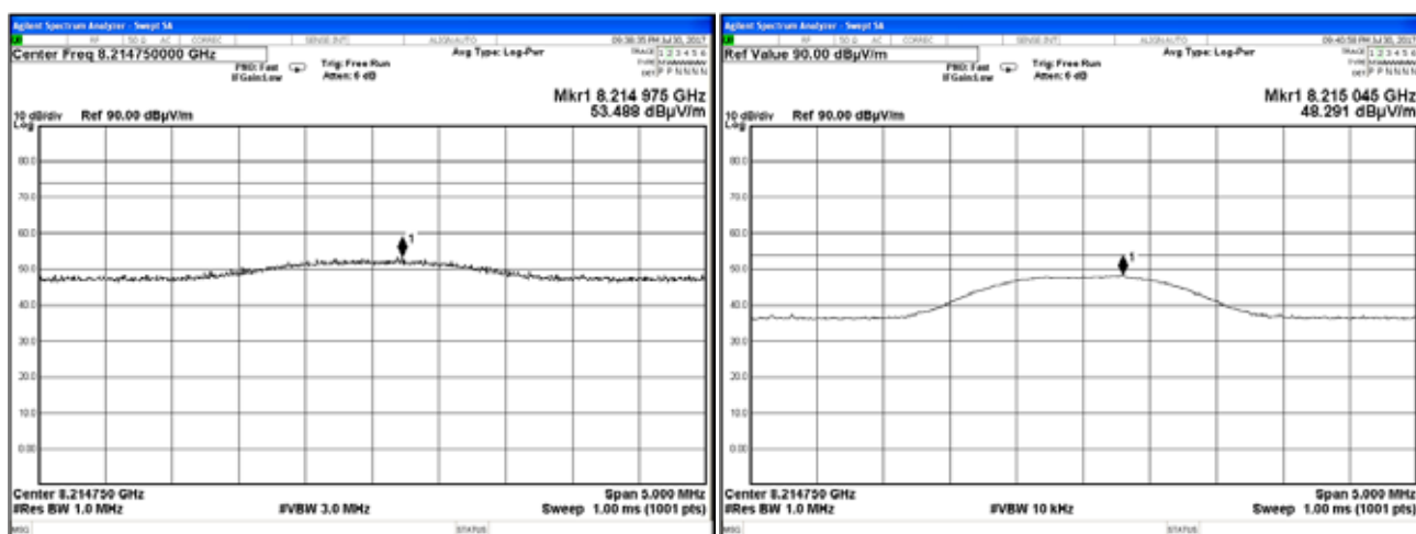
Plot 7.7.52 Radiated emission measurements at the ninth harmonic of low carrier frequency
