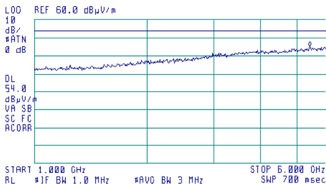
Plot 8.1.4 Radiated emission measurements above 1000 MHz
