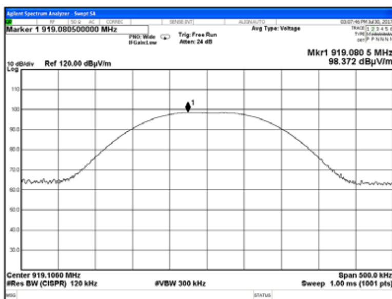
Plot 7.5.18 Field strength of carrier at high frequency and Unom
