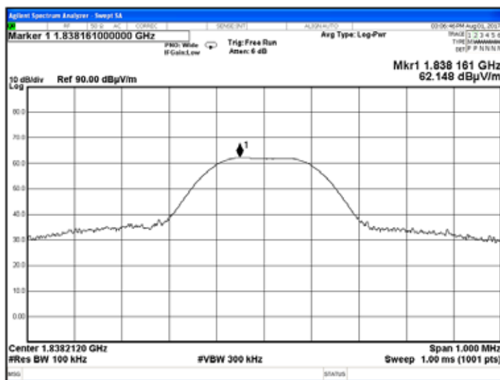
Plot 7.7.20 Radiated emission measurements at the second harmonic of high carrier frequency
