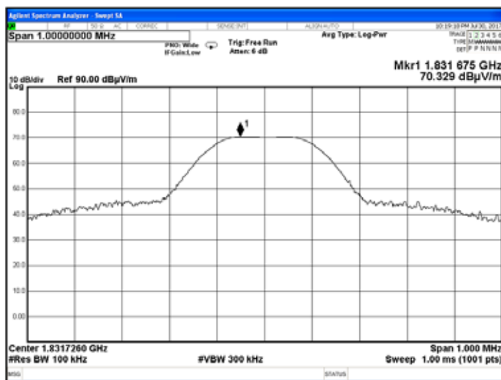
Plot 7.7.18 Radiated emission measurements at the second harmonic of mid carrier frequency
