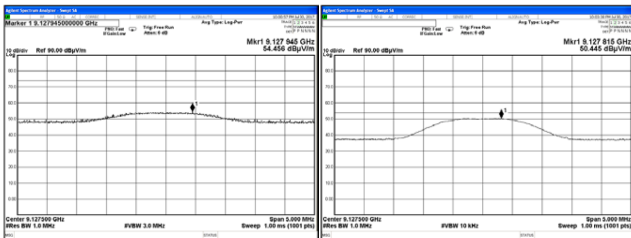
Plot 7.7.58 Radiated emission measurements at the tenth harmonic of low carrier frequency
