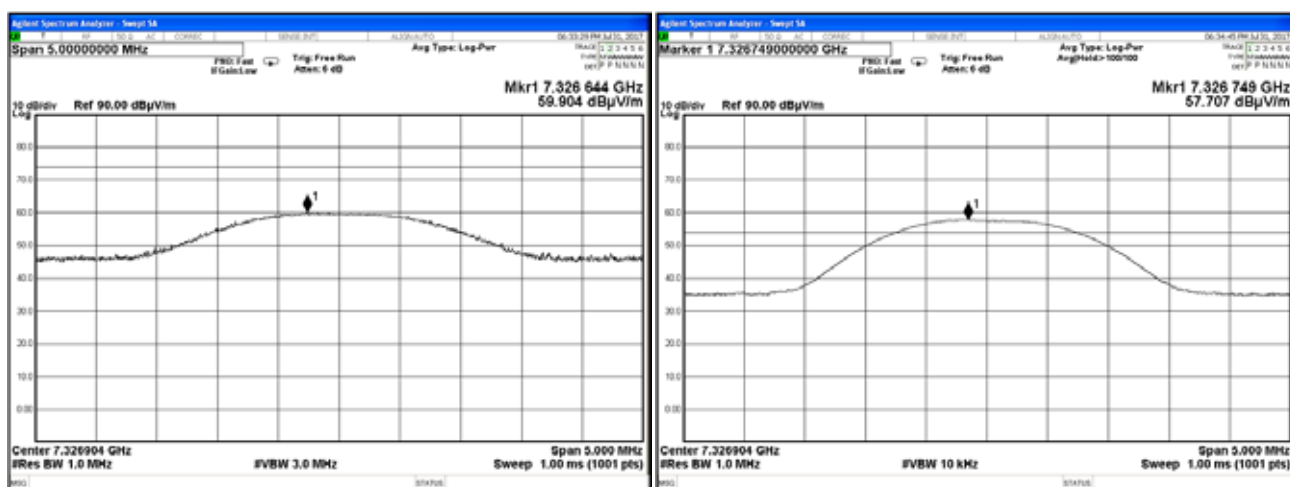
Plot 7.7.48 Radiated emission measurements at the eighth harmonic of mid carrier frequency
