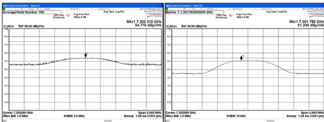
Plot 7.7.46 Radiated emission measurements at the eighth harmonic of low carrier frequency
