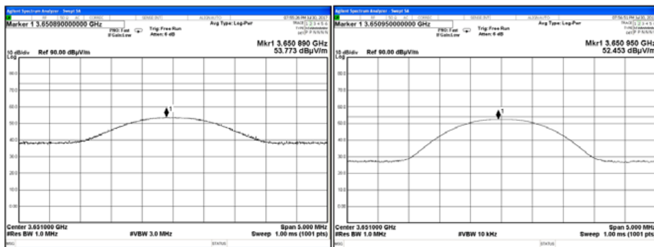
Plot 7.7.28 Radiated emission measurements at the fourth harmonic of low carrier frequency
