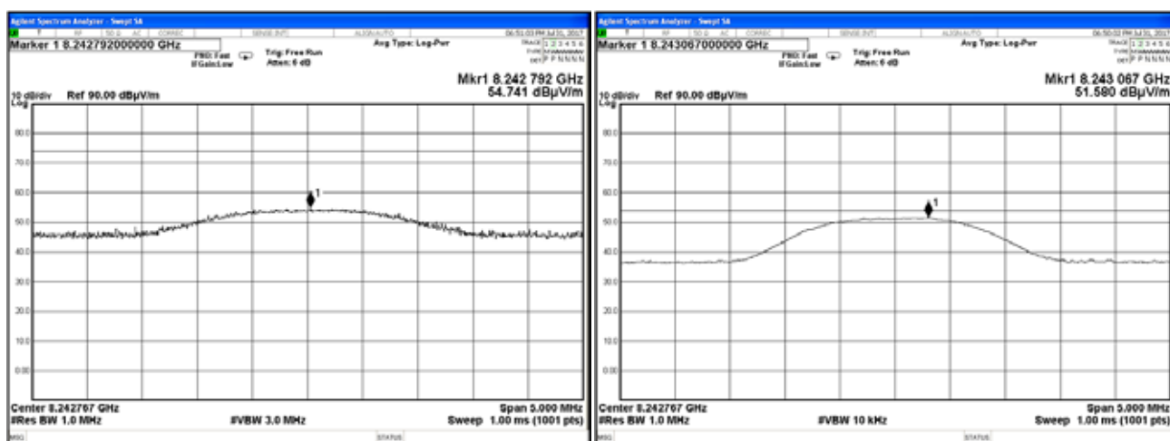
Plot 7.7.54 Radiated emission measurements at the ninth harmonic of mid carrier frequency
