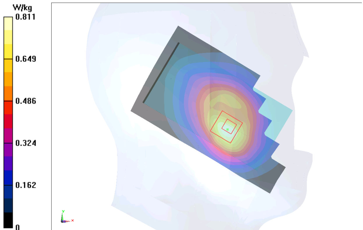
Fig.1 850MHz CH128
