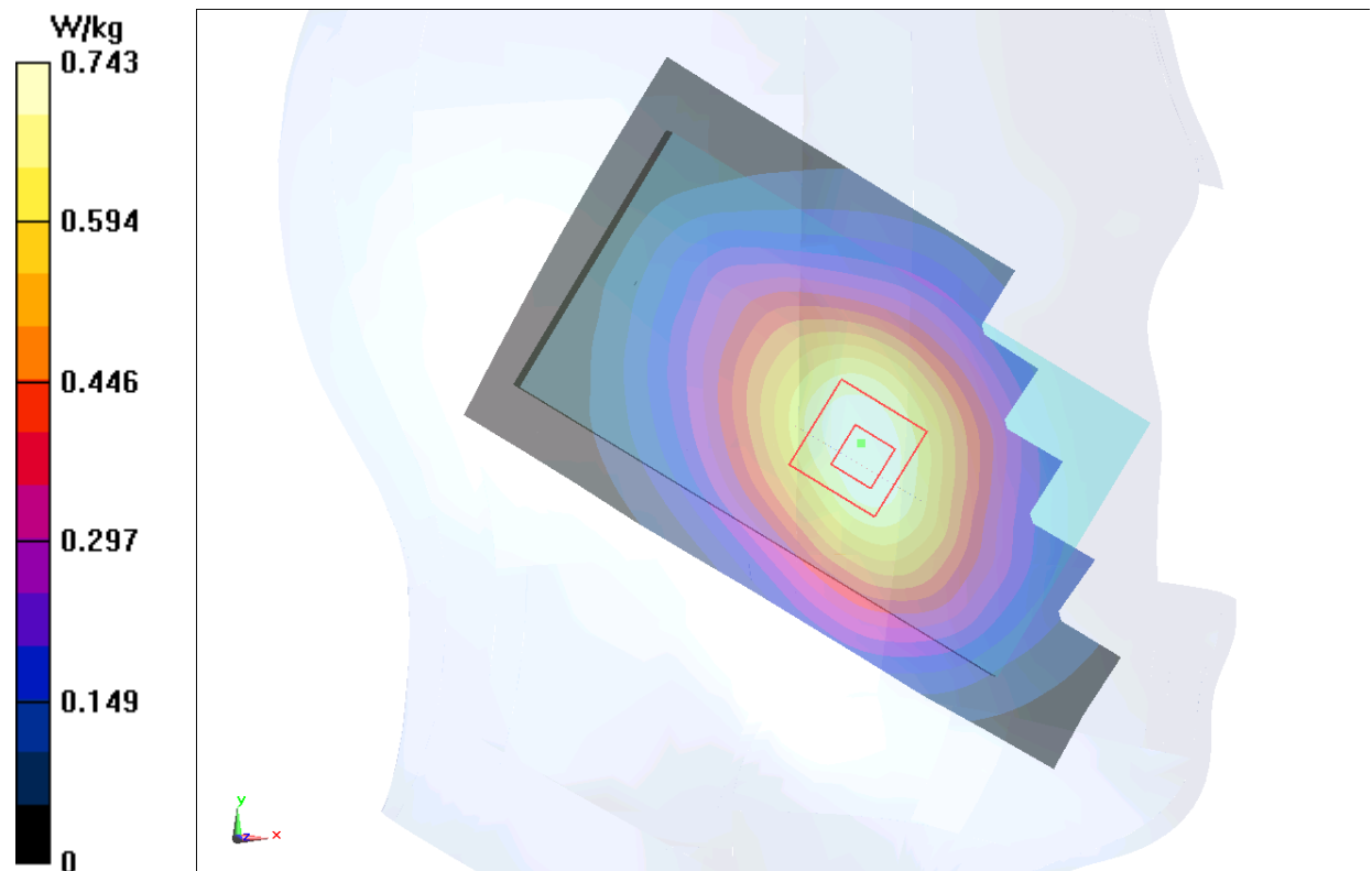
Fig.5 WCDMA 850 CH4132
