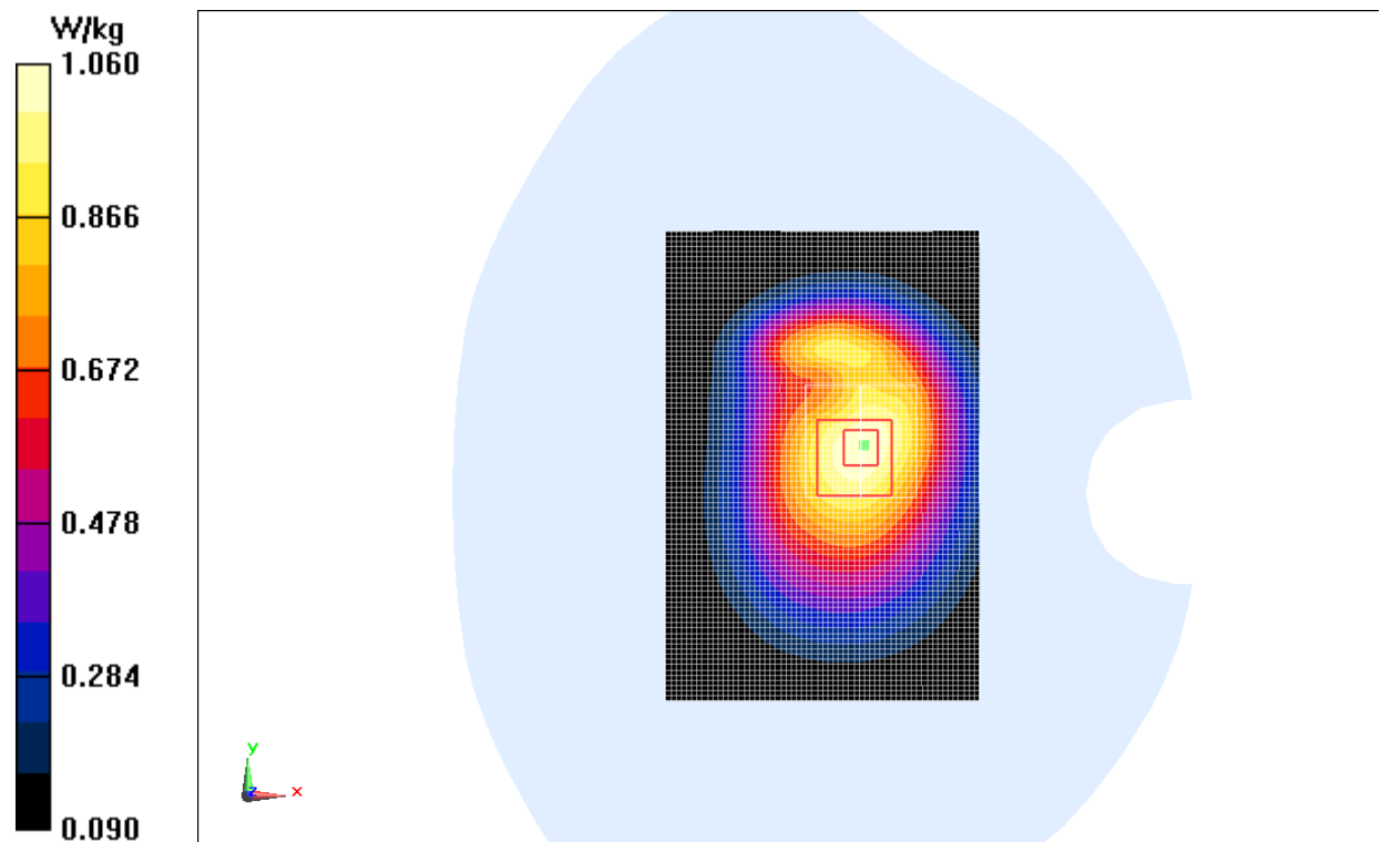
Fig.2 850 MHz CH128
