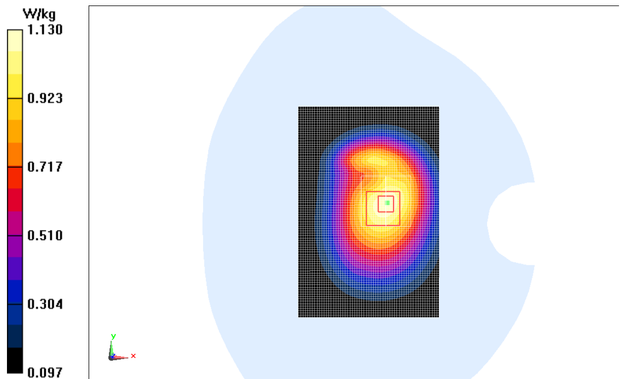
Fig.6 WCDMA 850 CH4132
