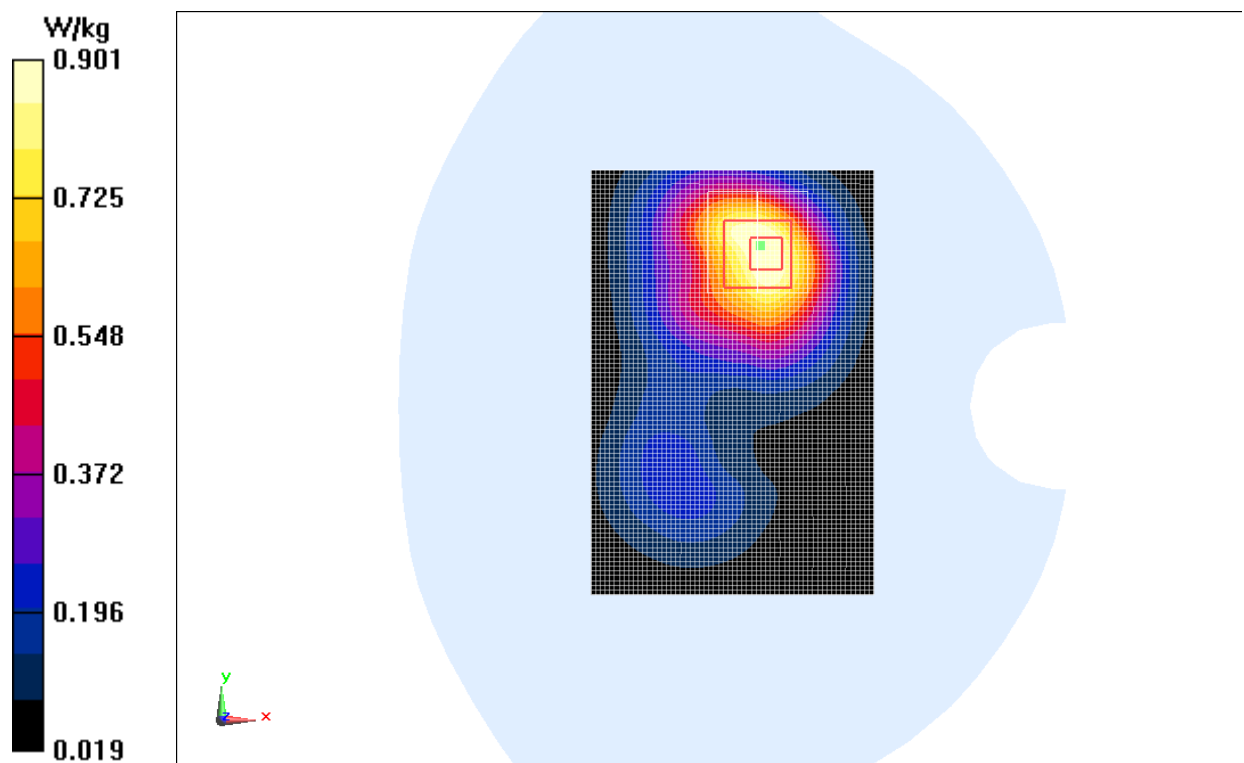
Fig.4 1900 MHz CH810
