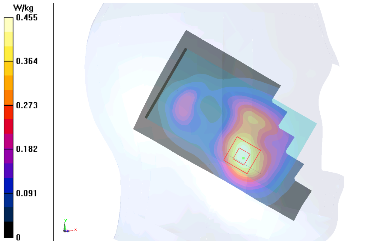
Fig.3 1900 MHz CH810
