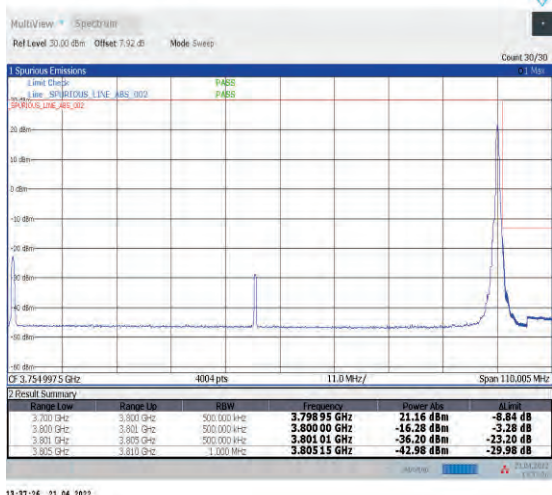
1-N78-3700-3800--30-100-H-2-DFT-PI2BPSK-Edge_1 RB_Right-1@272-Ant1-PASS-see graph
