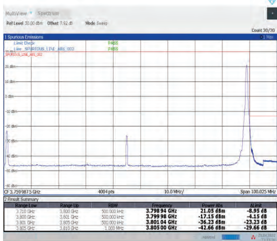
1-N78-3700-3800--30-90-H-5-CP-QPSK-Edge_1RB_Right-1@244-Ant1-PASS-see graph
