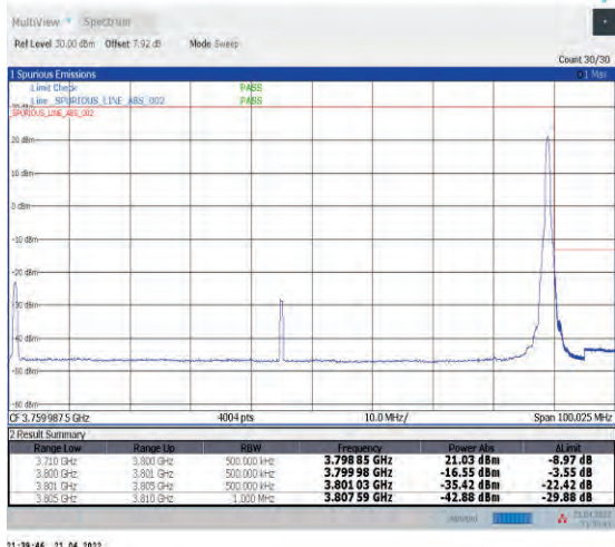
1-N78-3700-3800--30-90-H-2-DFT-PI2BPSK-Edge_1R_B_Right-1@244-Ant1-PASS-see graph
