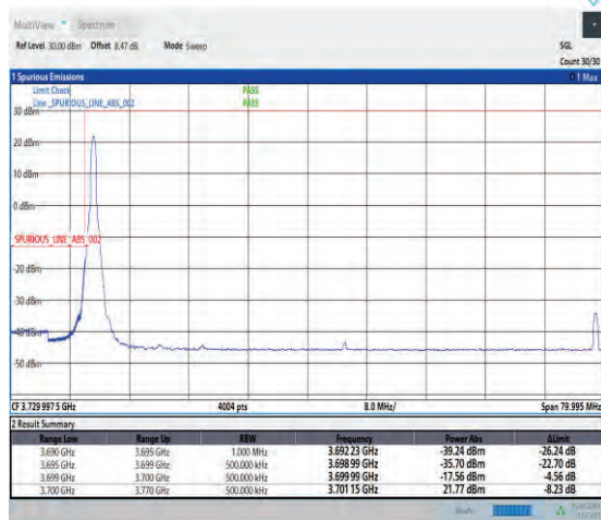
1-N78-3700-3800-PC1-30-70-L-1-DFT-PI2BPSK-Edg_e_1RB_Left-1@0-Ant1-1--PASS-see graph
