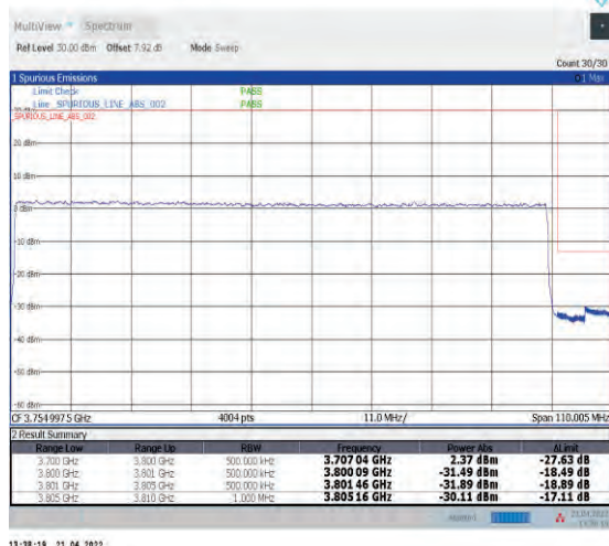
1-N78-3700-3800--30-100-H-3-DFT-PI2BPSK-Out er_Full-270@0-Ant1-PASS-see graph
