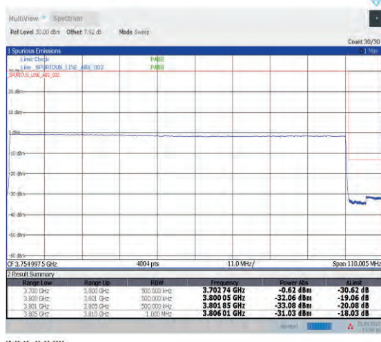
1-N78-3700-3800--30-100-H-6-CP-QPSK-Outer_Full-273@0-Ant1-PASS-see graph
