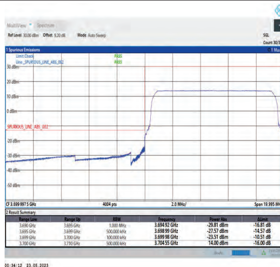
1-N78-3700-3800-PC1-30-10-L-6-CP-QPSK-Outer_Full-24@0-Ant1-1--PASS-see graph
