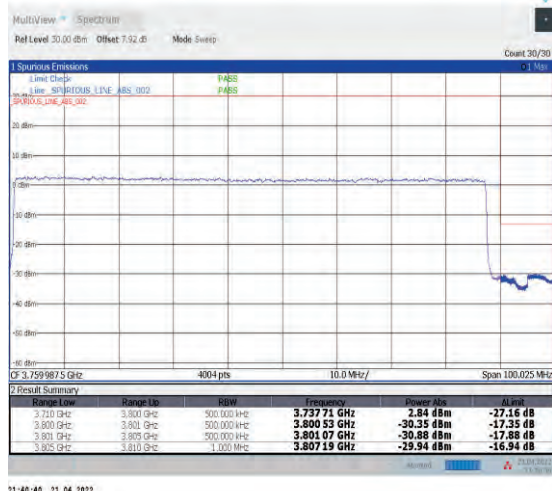
1-N78-3700-3800--30-90-H-3-DFT-PI2BPSK-Outer_Full-240@0-Ant1-PASS-see graph
