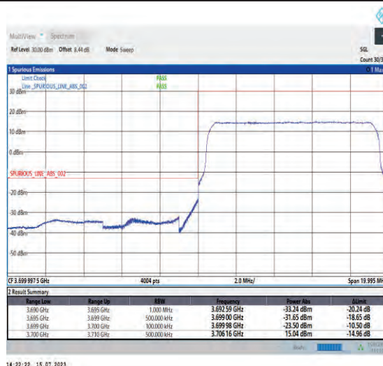
1-N78-3700-3800-PC1-30-10-L-3-DFT-PI2BPSK-Outer_Full-24@0-Ant1-1--PASS-see graph
