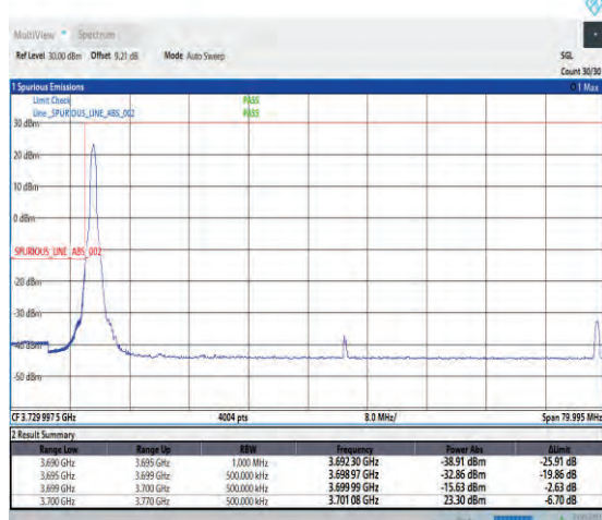
1-N78-3700-3800-PC1-30-70-L-4-CP-QPSK-Edge_1RB_Left-1@0-Ant1-1--PASS-see graph
