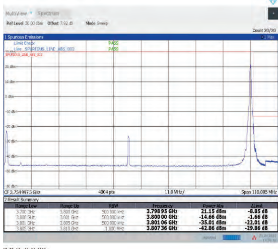
1-N78-3700-3800--30-100-H-5-CP-QPSK-Edge_1RB_Right-1@272-Ant1-PASS-see graph
