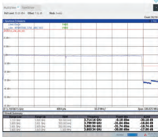
1-N78-3700-3800--30-90-H-6-CP-QPSK-Outer_Full-245@0-Ant1-PASS-see graph
