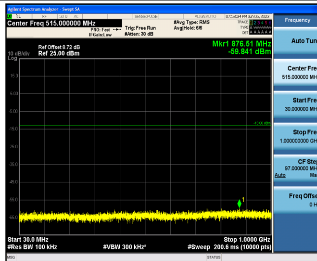
Band2-5MHz-QPSK-18625-1-0-Low-30-1000--59.84-PASS
