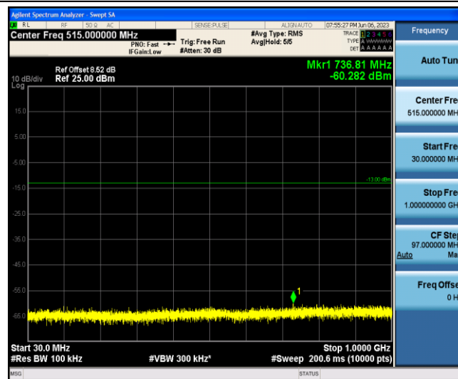
Band2-5MHz-16QAM-19175-1-0-Low-30-1000--60.28-PASS
