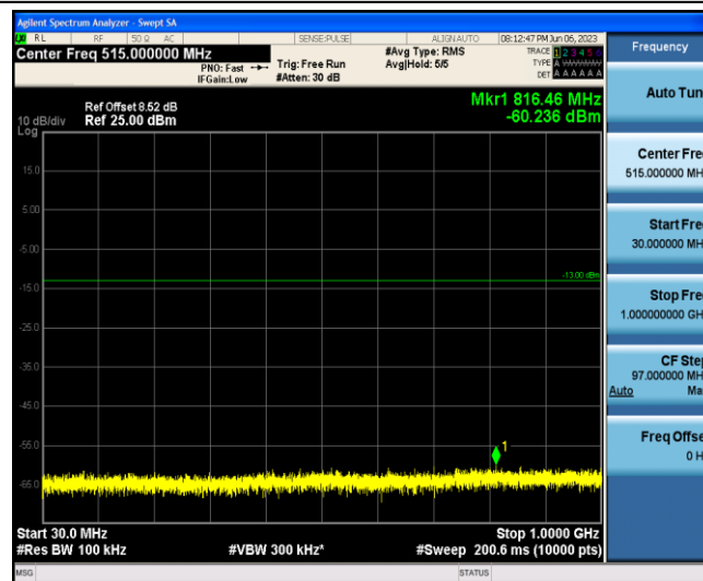
Band2-10MHz-16QAM-19150-1-0-Low-30-1000--60.24-PASS
