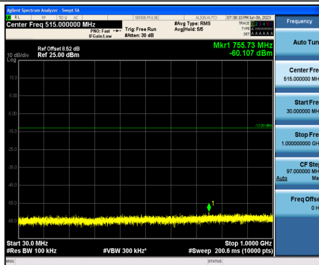
Band2-3MHz-QPSK-19185-1-0-Low-30-1000--60.11-PASS
