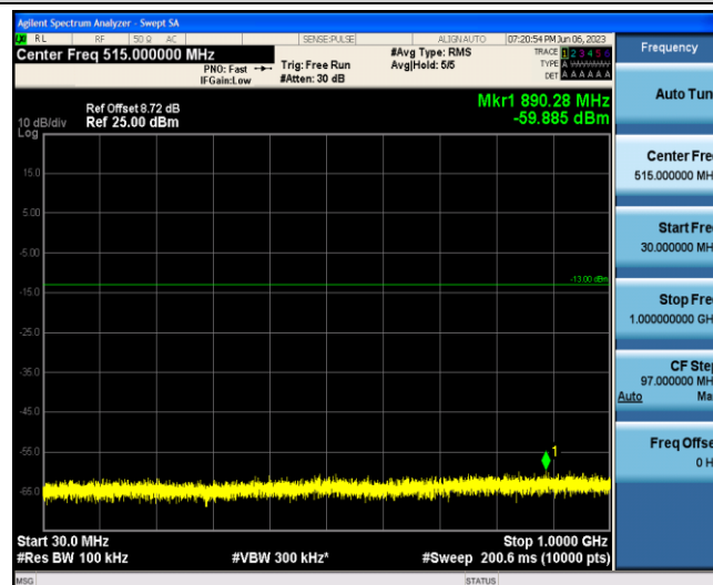
Band2-1.4MHz-16QAM-18900-1-0-Low-30-1000--59.89-PASS
