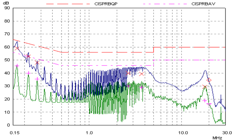
Figure 2 - Line Scan
