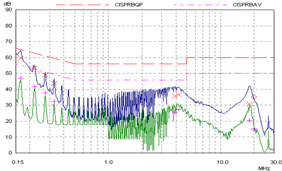
Figure 3 - Neutral Scan
