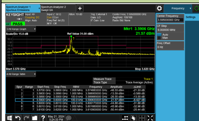
15MHz Channel Bandwidth - 1RB
