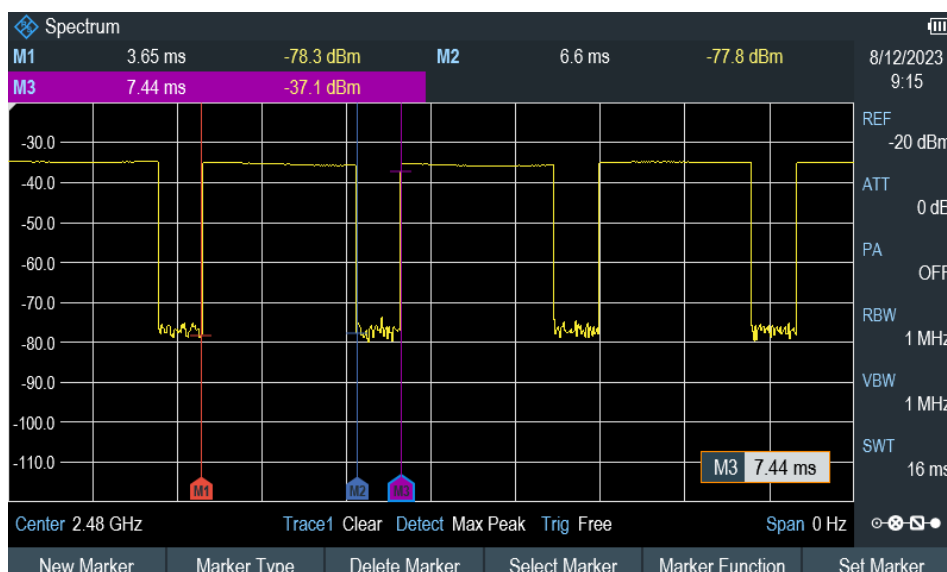
Time-domain plot for Bluetooth transmission signal
