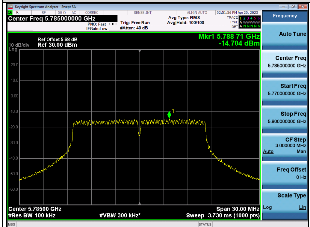
Test_Graph_802.11a_ANT1_5785_6Mbps_PSD
