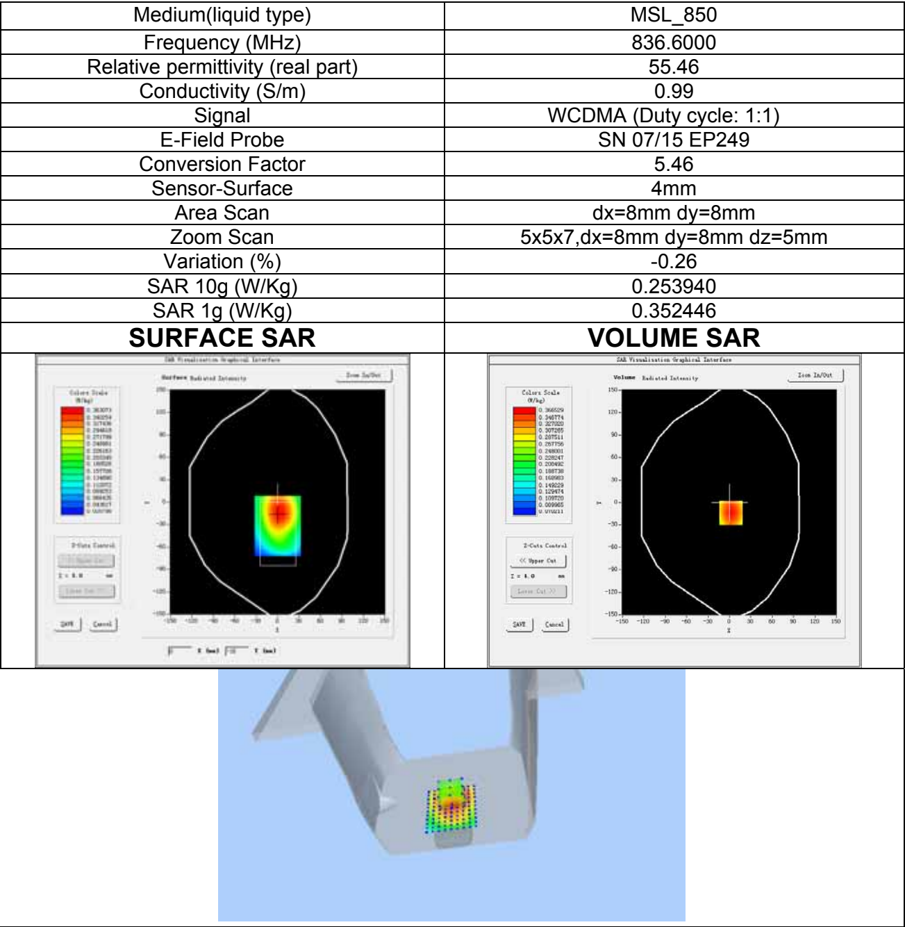
Plot 5: WCDMA BAND , Middle channel (Body-worn/Hotspot, Back Surface) Test Date:Apr. 11,2016
