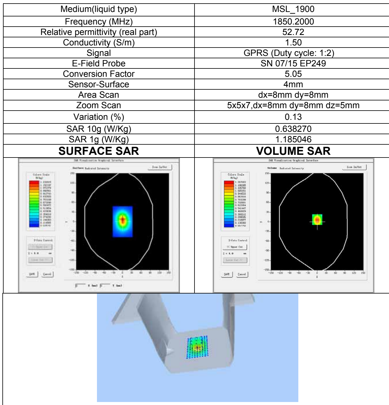
Plot 8: GPRS1900, Low channel (Hotspot, Bottom Edge) repeated measured Test Date: Apr. 13, 2016
