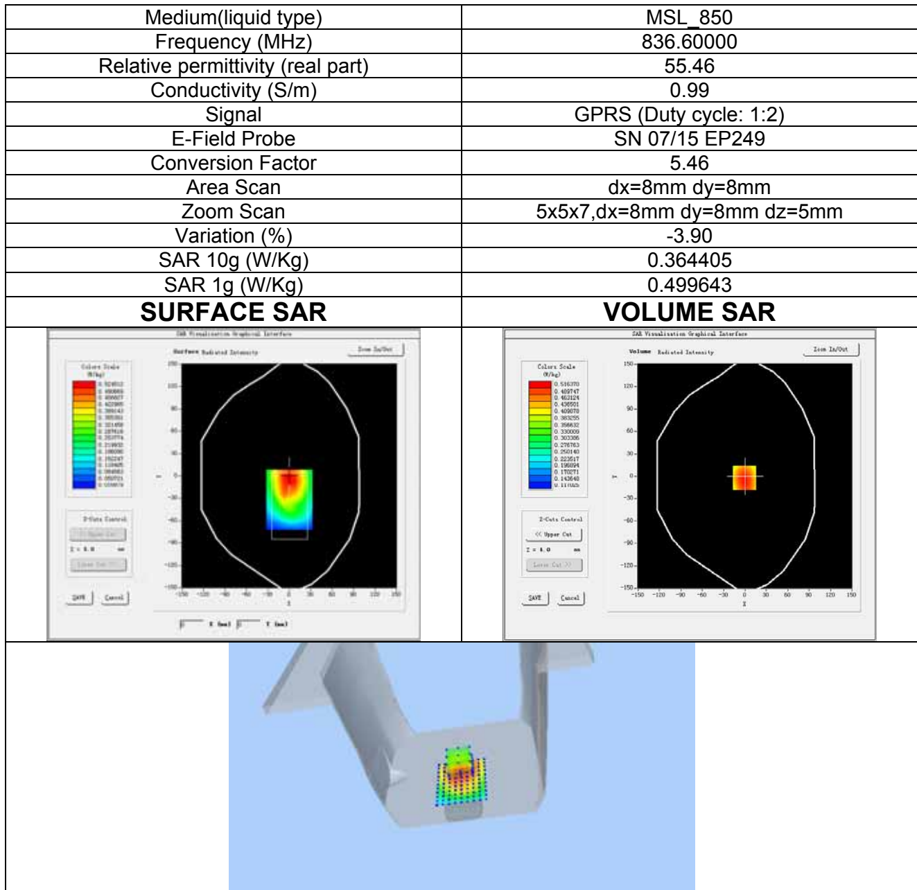
Plot 3: GPRS850MHz, Middle channel (Hotspot, Back Surface) Test Date: Apr. 11, 2016
