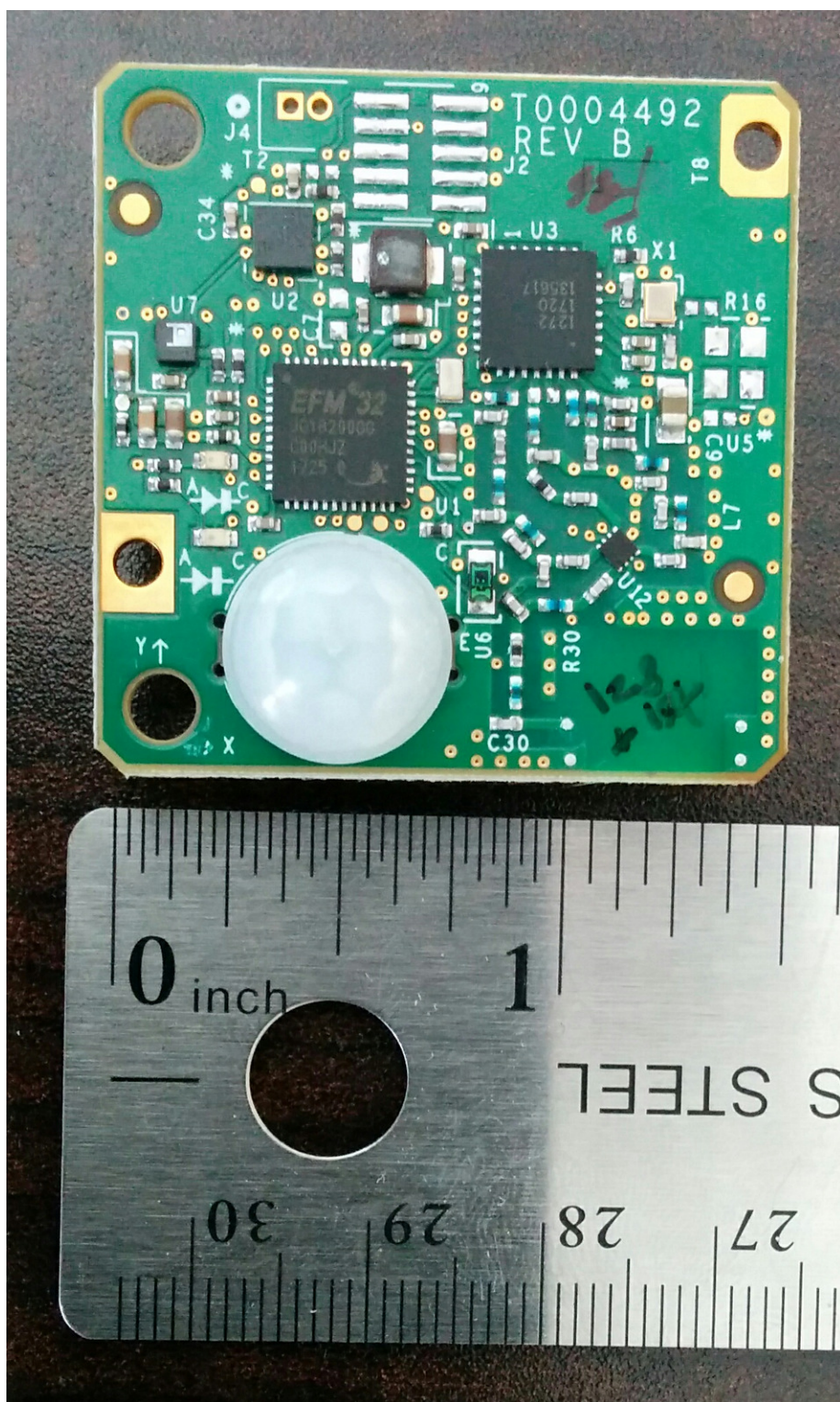
T0004885 PCB Top View (PIR Sensor)
