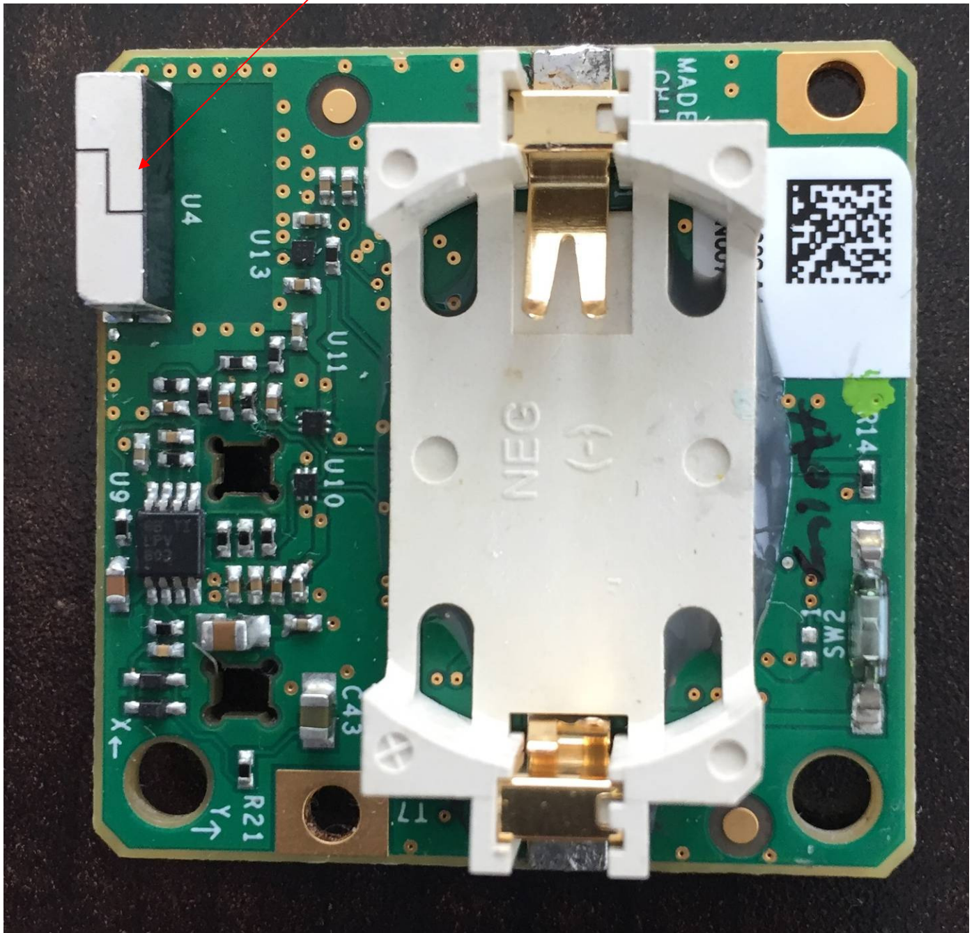
T0004885 PCB Bottom view (PIR Sensor)
