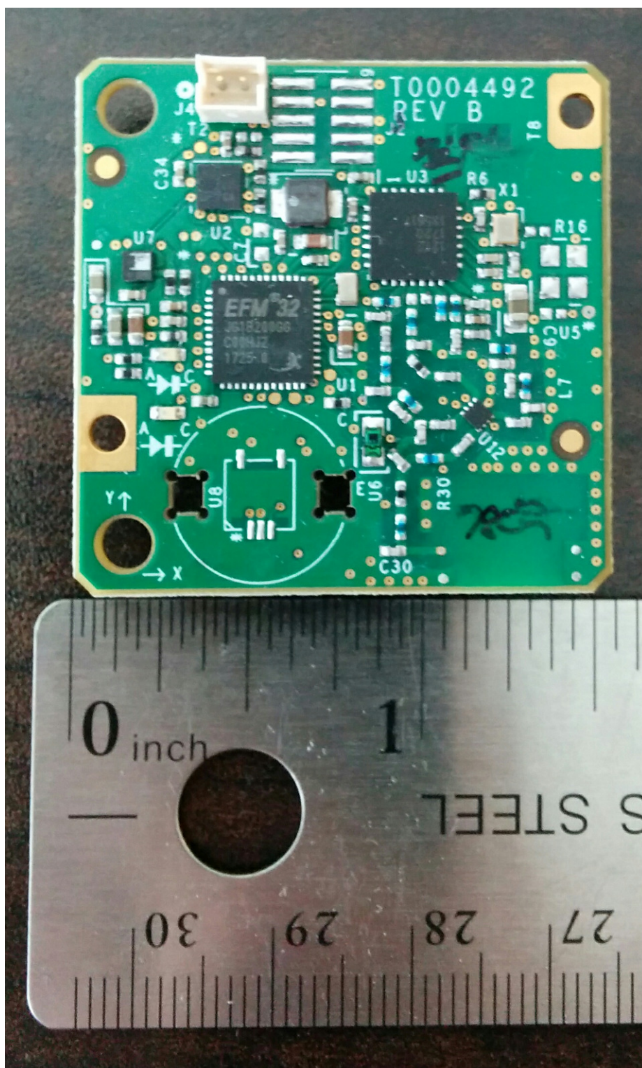
T0004886 PCB Top View (External Connector Sensor)
