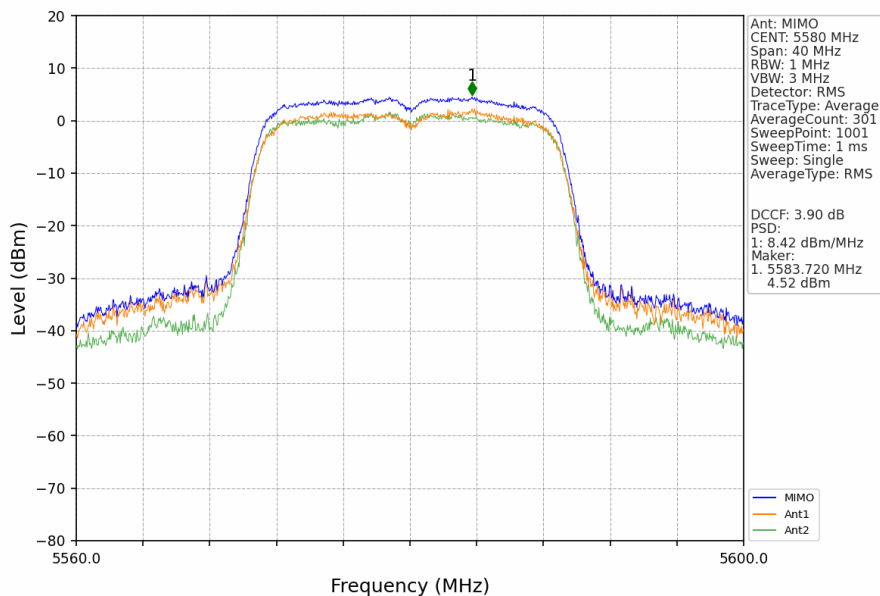
802.11ac(VHT20)_MCH_5580MHz_MIMO_NTNV
