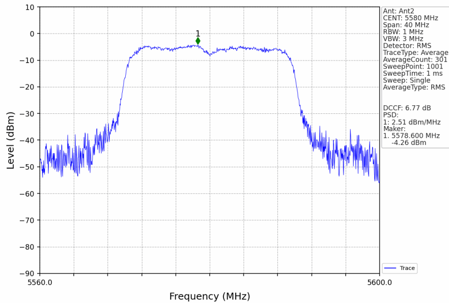
802.11ax(HEW20)_MCH_5580MHz_RU242_Left_MIMO_NTNV
