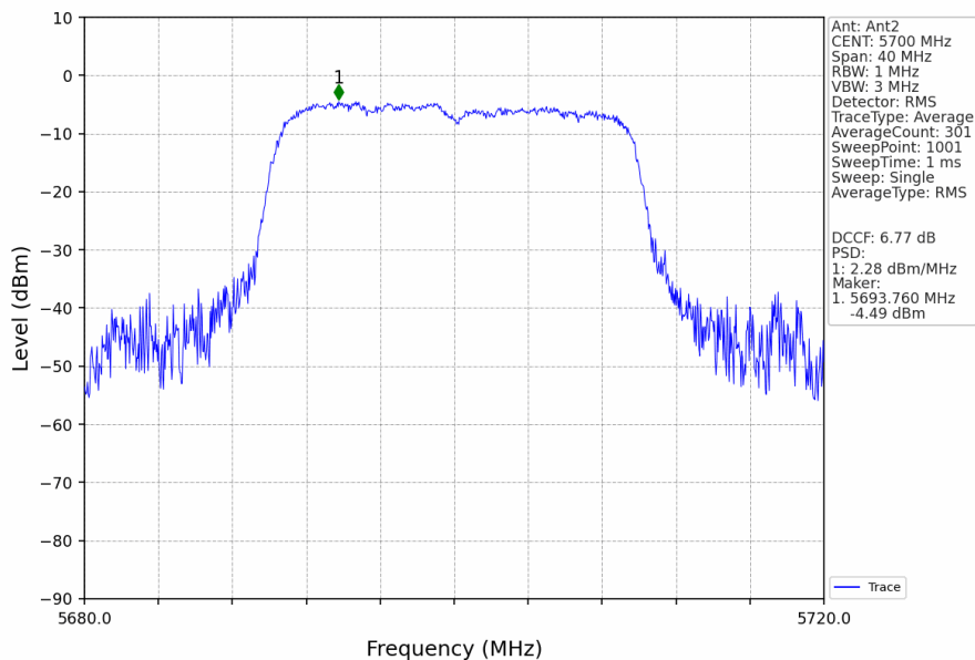
802.11ax(HEW20)_HCH_5700MHz_RU242_Left_Ant2_NTNV
