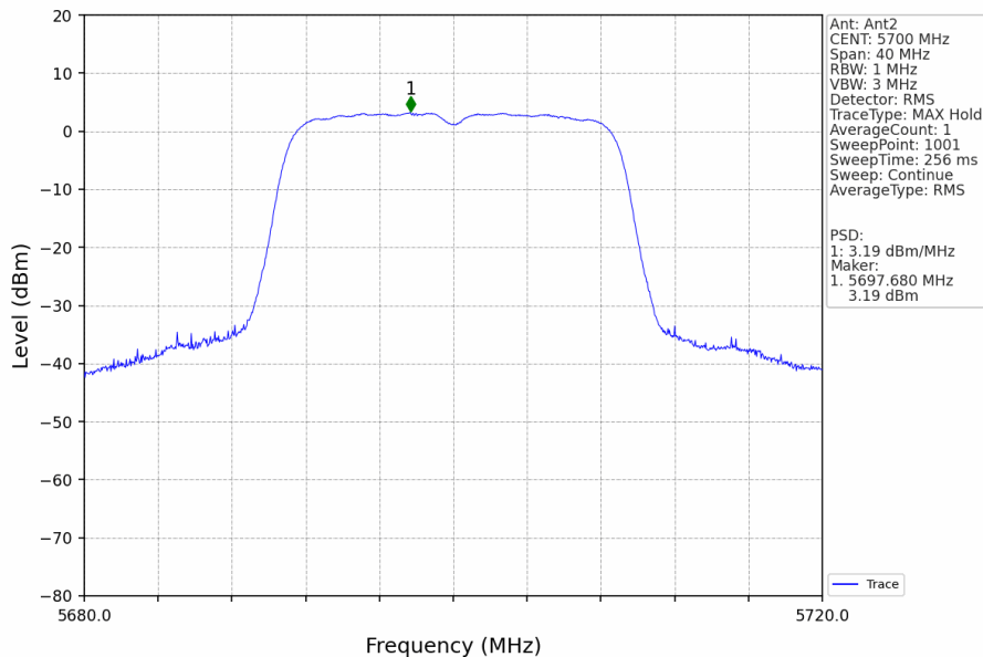
802.11ac(VHT20)_HCH_5700MHz_Ant2_NTNV
