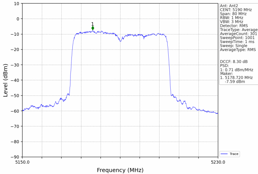
802.11ax(HEW40)_LCH_5190MHz_RU484_Left_MIMO_NTNV
