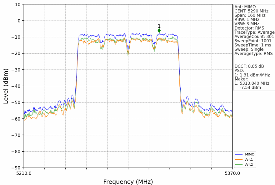
802.11ac(VHT80)_MCH_5290MHz_MIMO_NTNV
