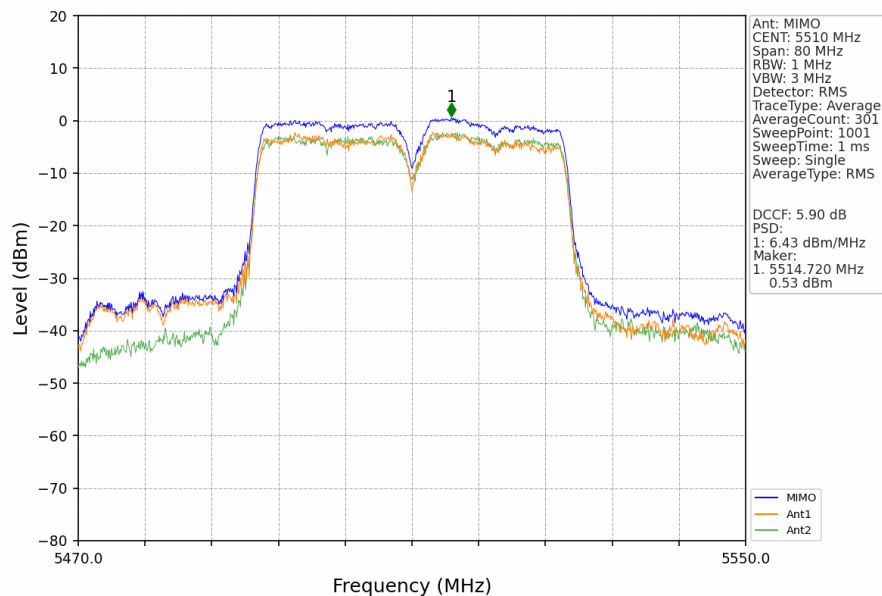
802.11ac(VHT40)_LCH_5510MHz_MIMO_NTNV
