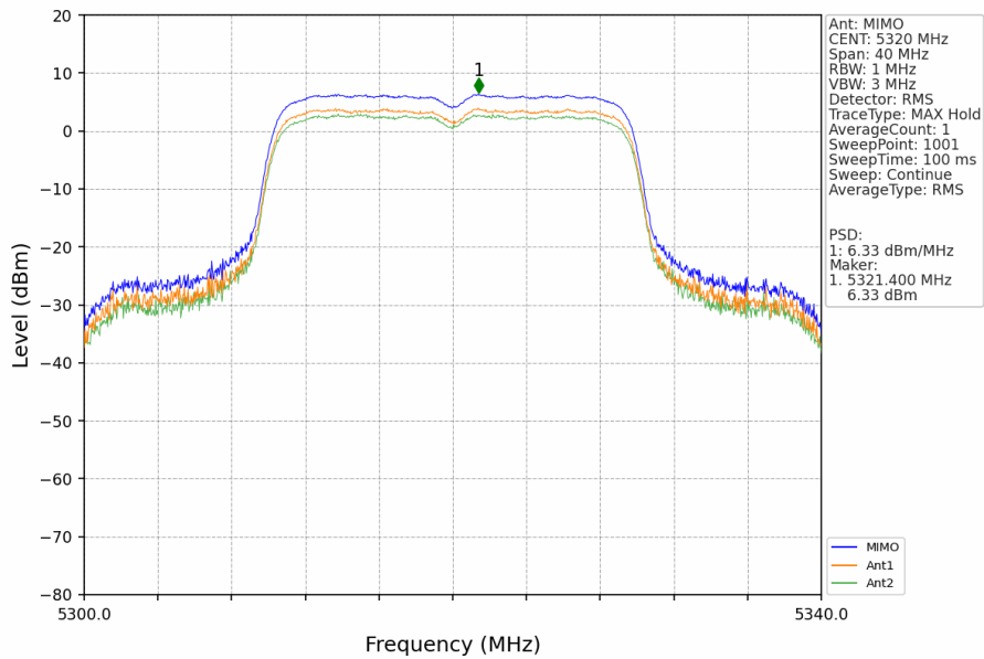
802.11ax(HEW20)_HCH_5320MHz_RU242_Left_MIMO_NTNV
