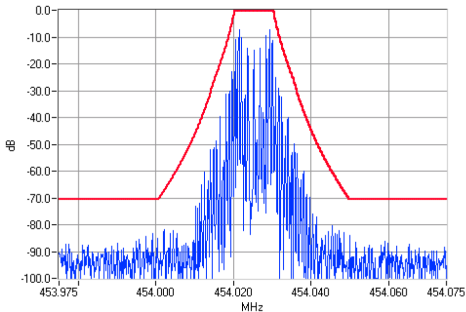
Paging Modulation 454.025MHz Mask G 100W Pass 100W 1600 BAUD MODULATED 454.025 MHz T857-26-1012 Exciter
