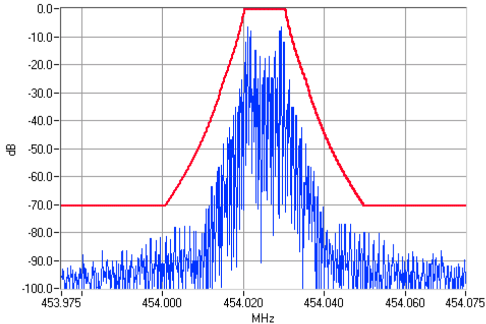
Paging Modulation 454.025MHz Mask G 100W Pass 100W 1200 BAUD MODULATED 454.025 MHz T857-26-1012 Exciter
