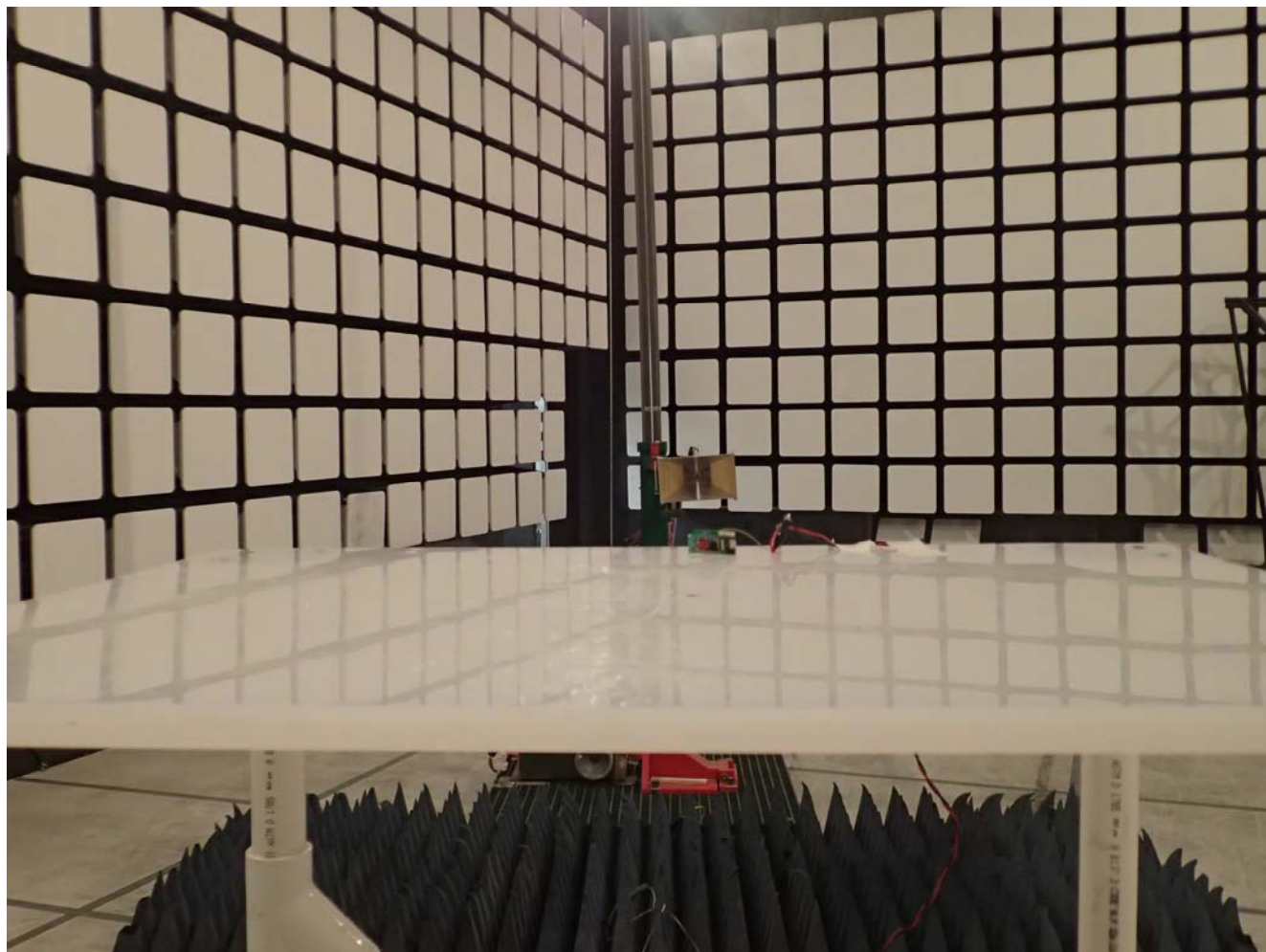
Radiated Emissions @ 3 m, Above 1 GHz, Orthogonal Position 2
