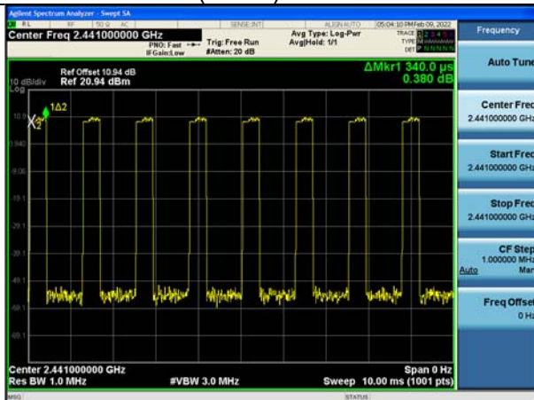
Test Mode: 8DPSK 3DH1 2441MHz
