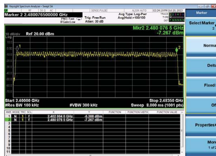
8-DPSK Modulation
