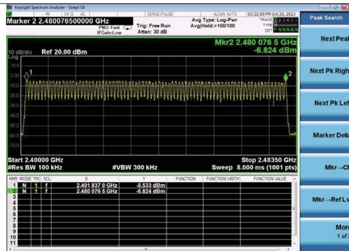
GFSK Modulation
