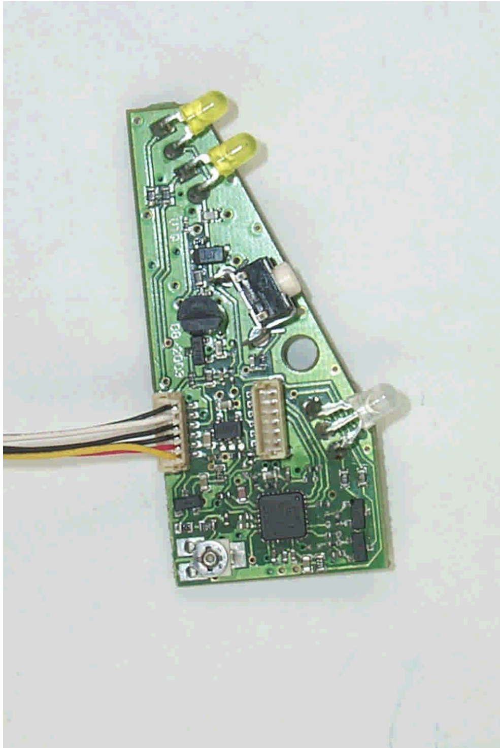
30764TX_pcb5.jpg EUT (transmitter controller-board)
