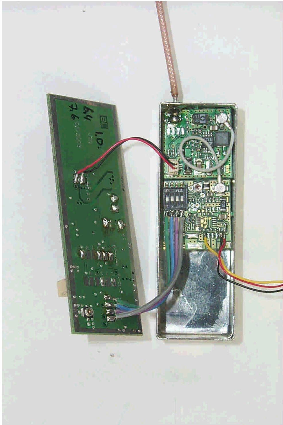
30764TX_pcb1.jpg EUT (rf-module) internal view
