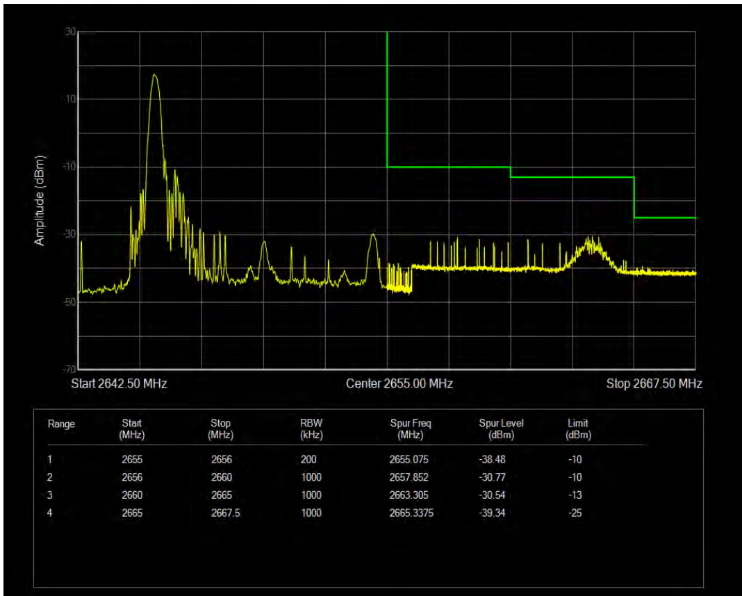
Band41(2555-2655) 16QAM BW=10MHz Channel=41190 RB Size=1 Position=#Max
