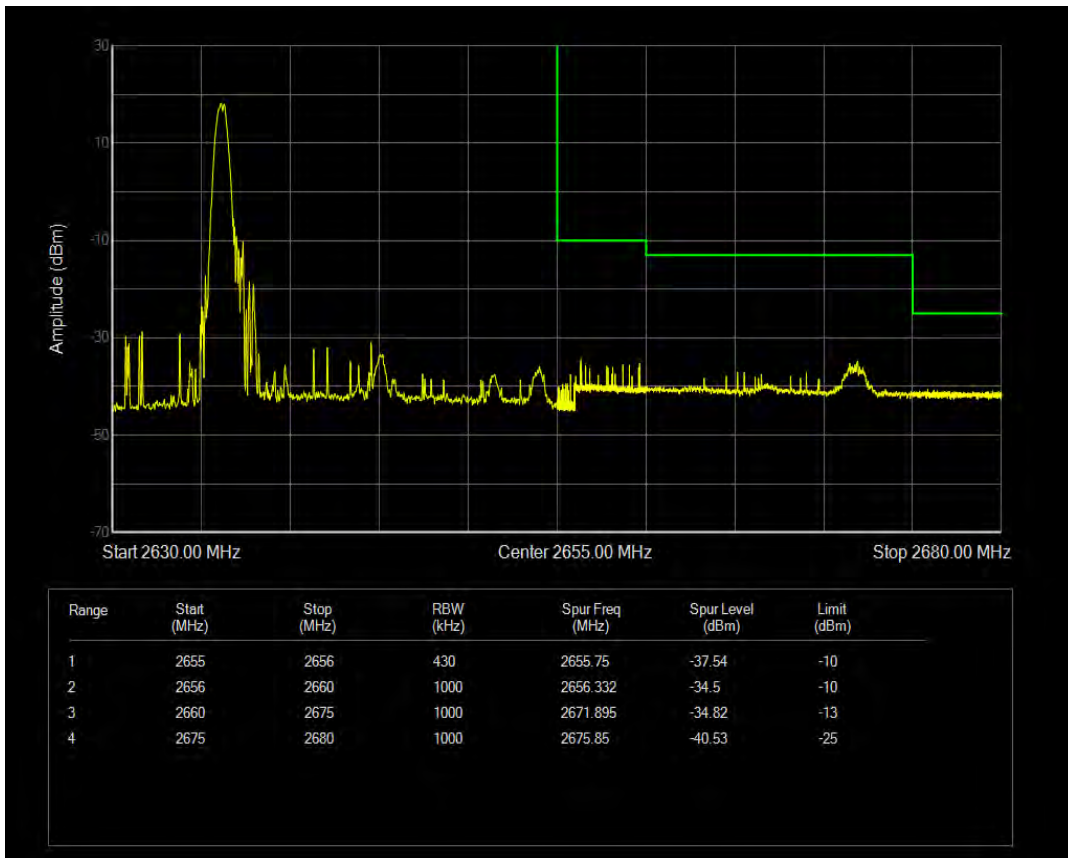
Band41(2555-2655) 16QAM BW=20MHz Channel=41140 RB Size=1 Position=#Max
