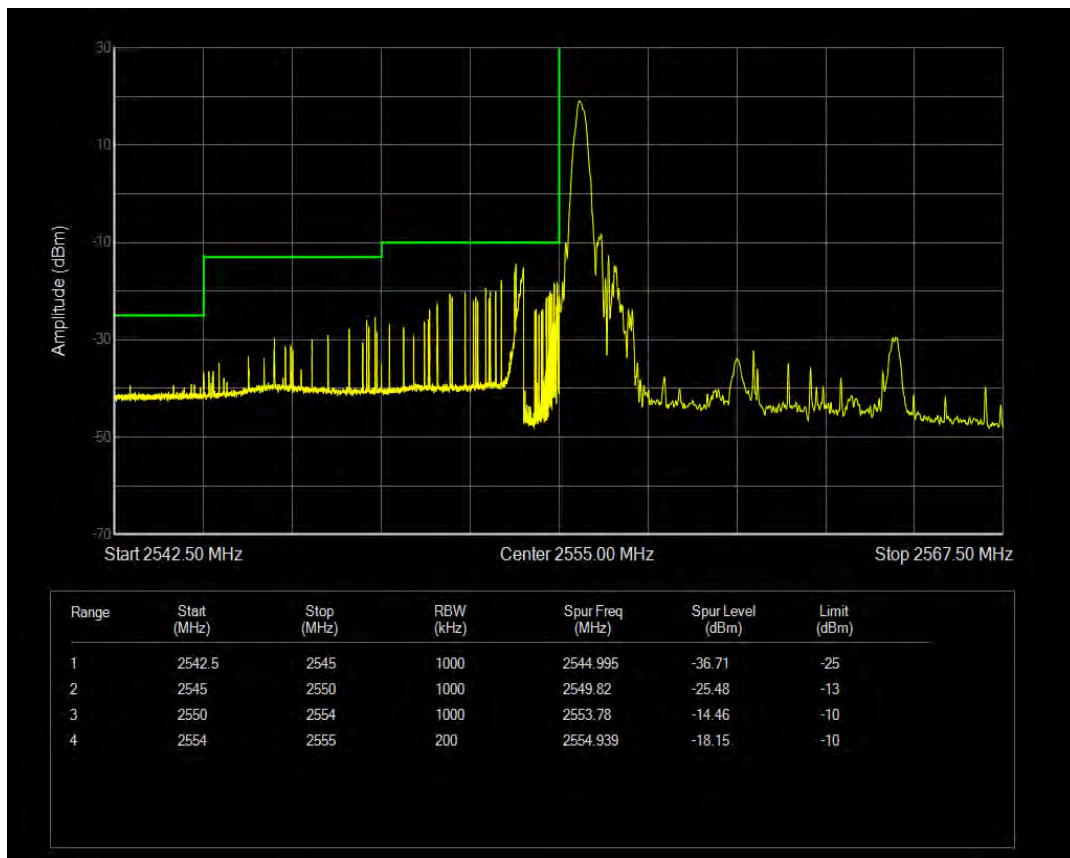
Band41(2555-2655) 16QAM BW=10MHz Channel=40290 RB Size=1 Position=#Max
