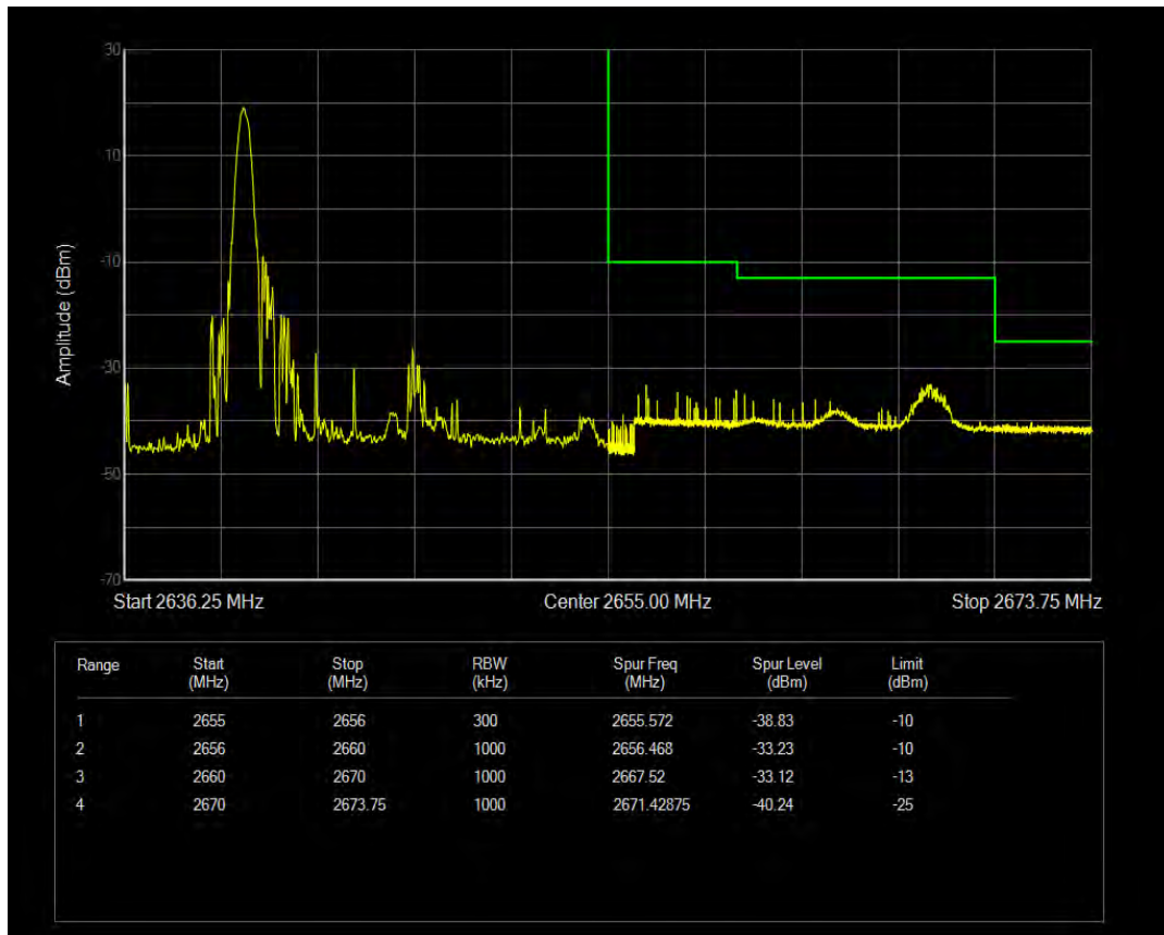
Band41(2555-2655) QPSK BW=15MHz Channel=41165 RB Size=1 Position=#Max
