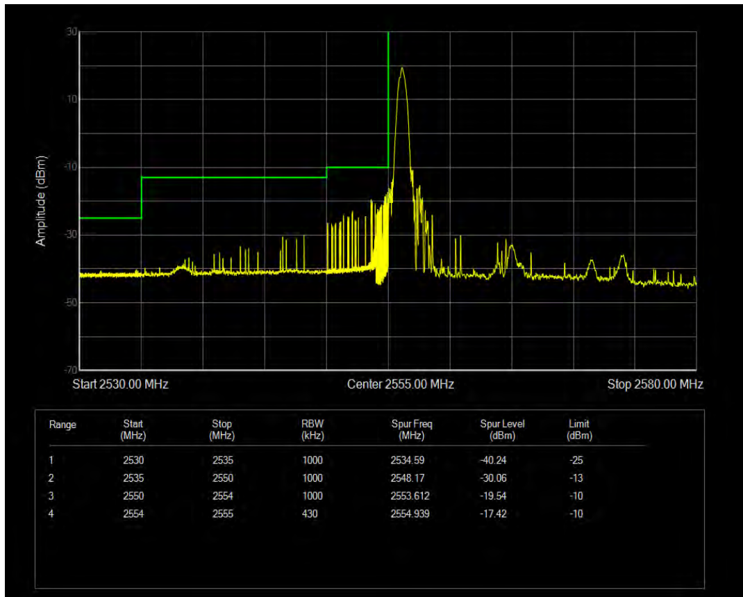
Band41(2555-2655) QPSK BW=20MHz Channel=40340 RB Size=1 Position=#Max
