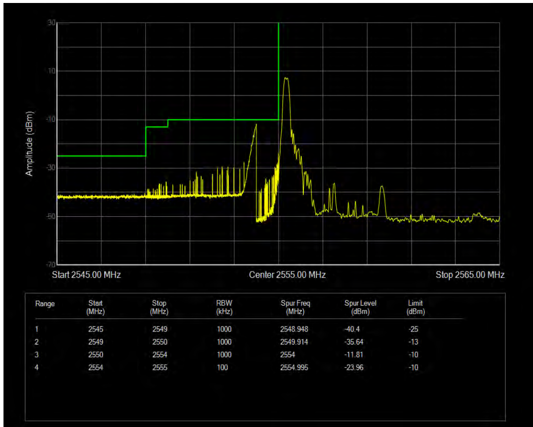
Band41(2555-2655) QPSK BW=5MHz Channel=40265 RB Size=1 Position=#Max
