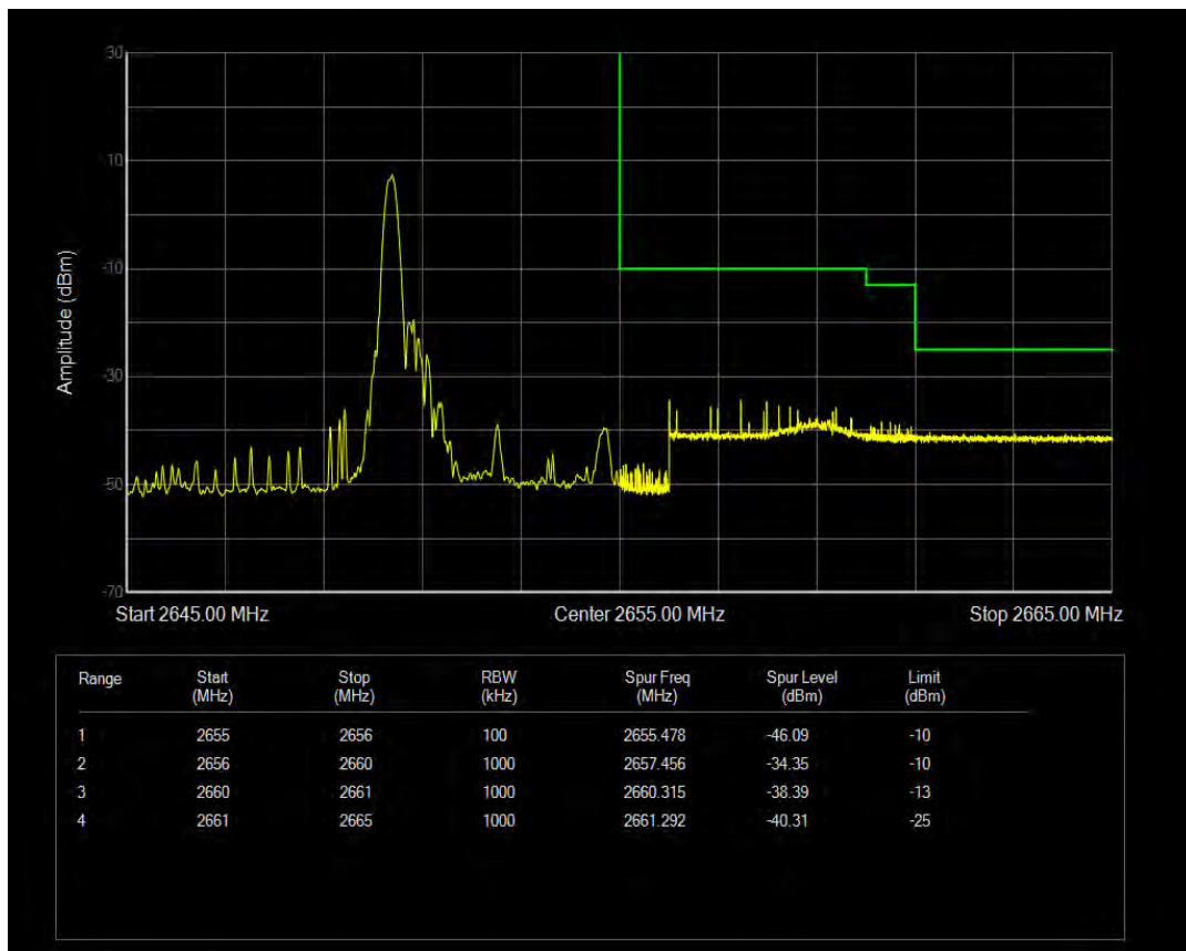
Band41(2555-2655) 16QAM BW=5MHz Channel=41215 RB Size=1 Position=#Max
