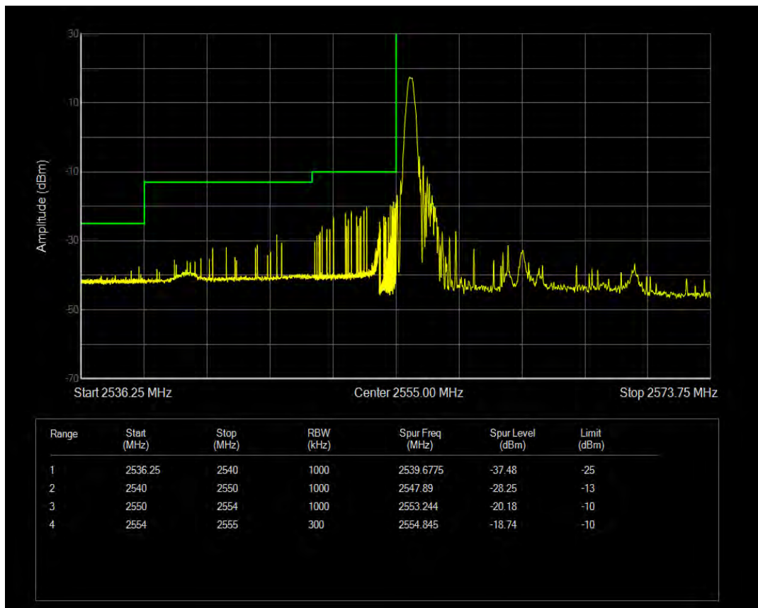
Band41(2555-2655) 16QAM BW=15MHz Channel=40315 RB Size=1 Position=#Max
