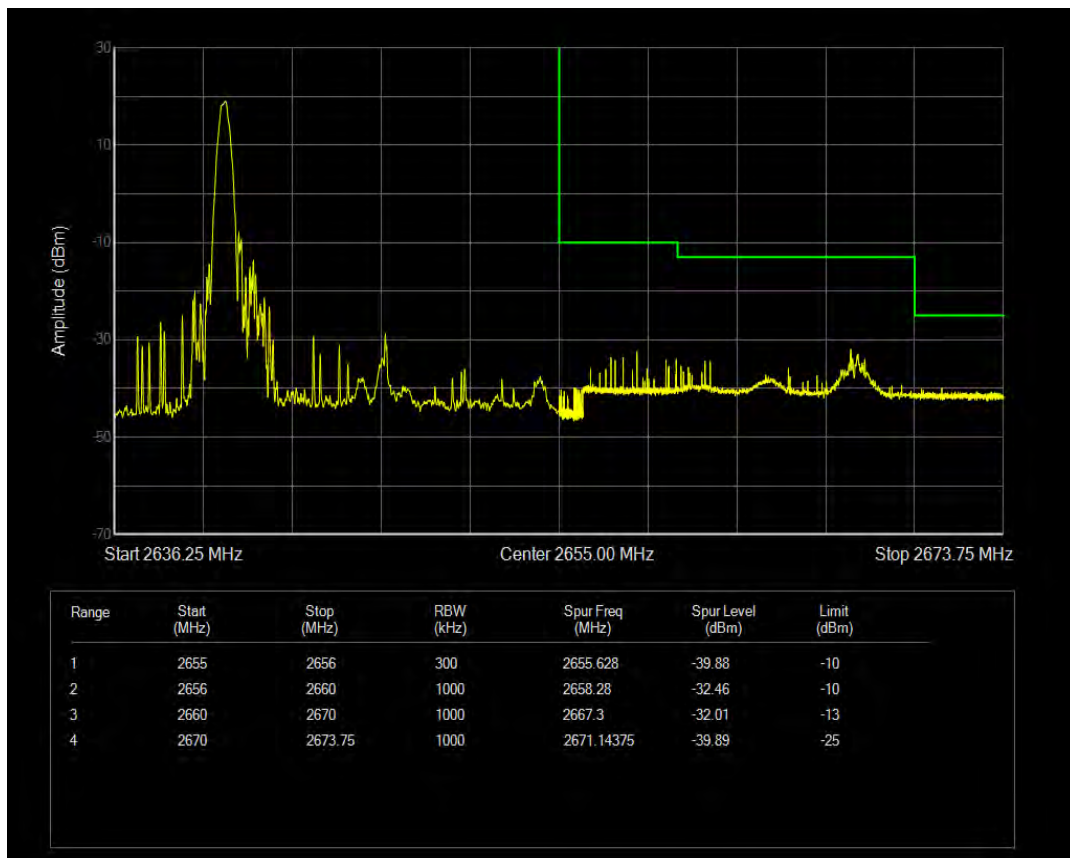
Band41(2555-2655) 16QAM BW=15MHz Channel=41165 RB Size=1 Position=#Max
