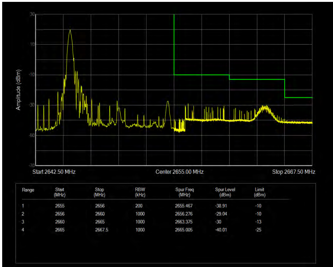
Band41(2555-2655) QPSK BW=10MHz Channel=41190 RB Size=1 Position=#Max
