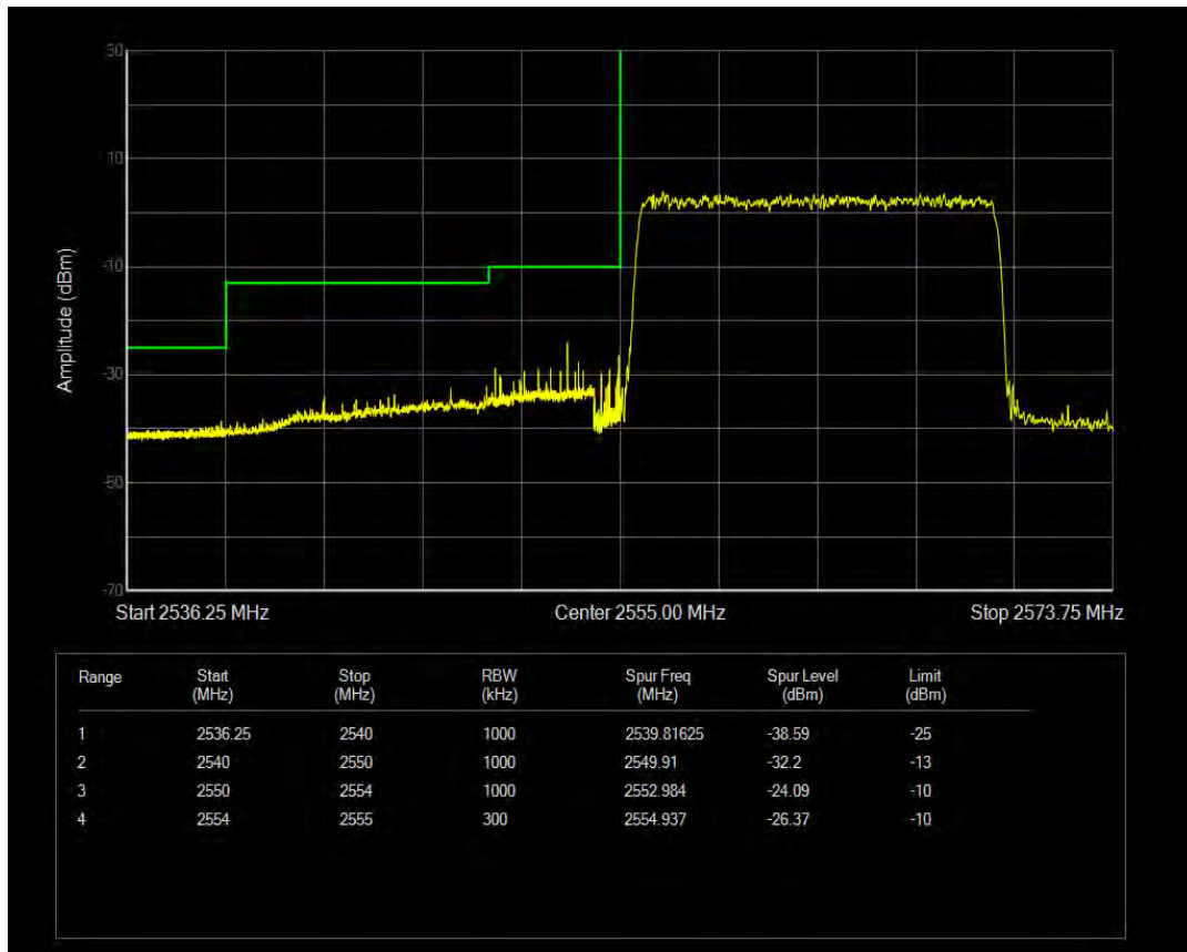
Band41(2555-2655) 16QAM BW=15MHz Channel=40315 RB Size=1 Position=#0
