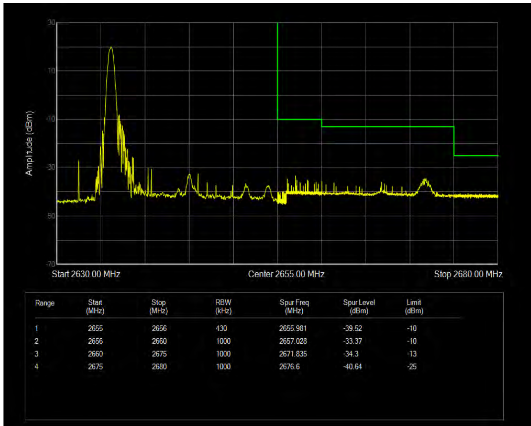
Band41(2555-2655) QPSK BW=20MHz Channel=41140 RB Size=1 Position=#Max
