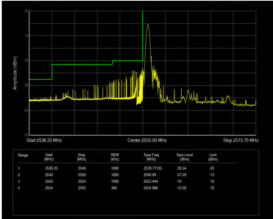
Band41(2555-2655) QPSK BW=15MHz Channel=40315 RB Size=1 Position=#Max
