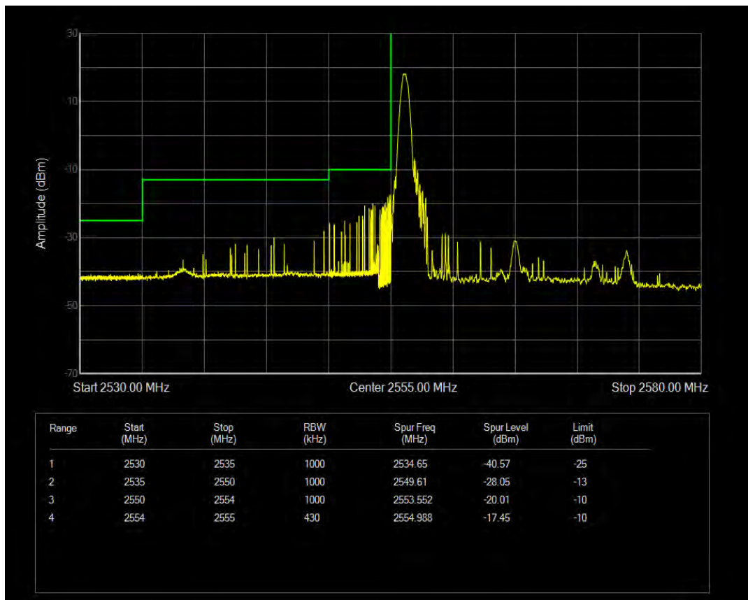
Band41(2555-2655) 16QAM BW=20MHz Channel=40340 RB Size=1 Position=#Max
