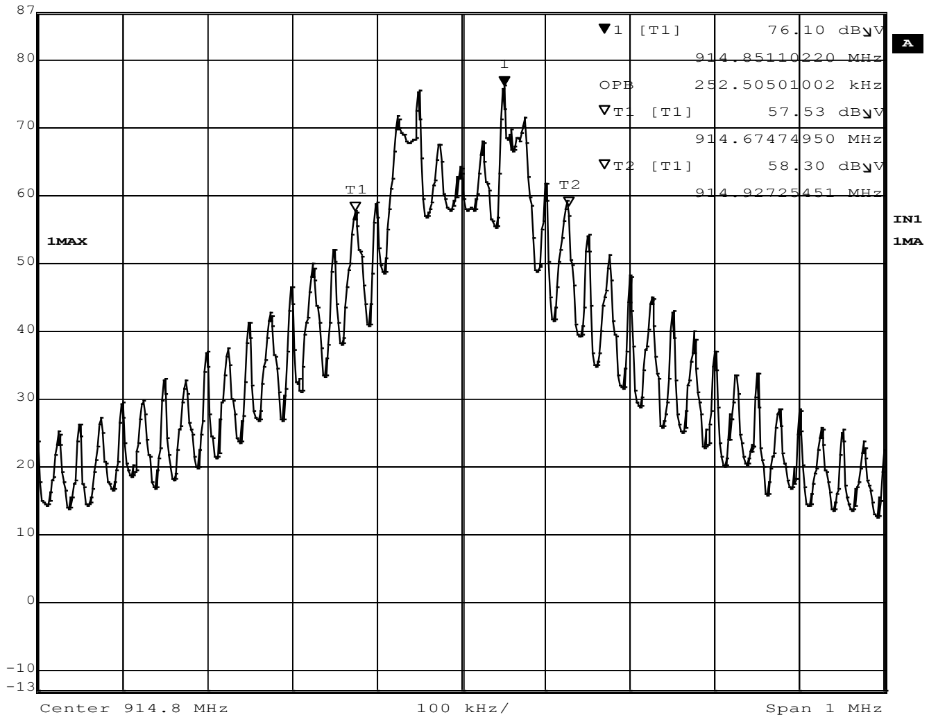
Figure 13 – Occupied Bandwidth, Mid Channel, 252.51 kHz
