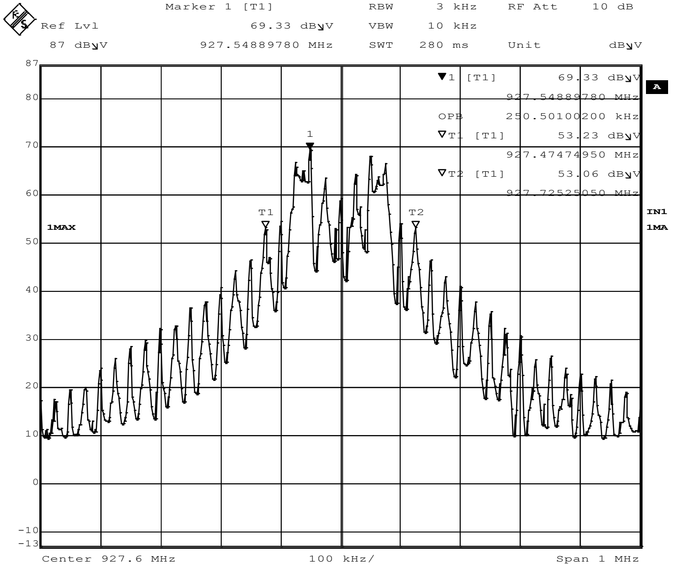
Figure 14 - Occupied Bandwidth, High Channel, 250.50 kHz
