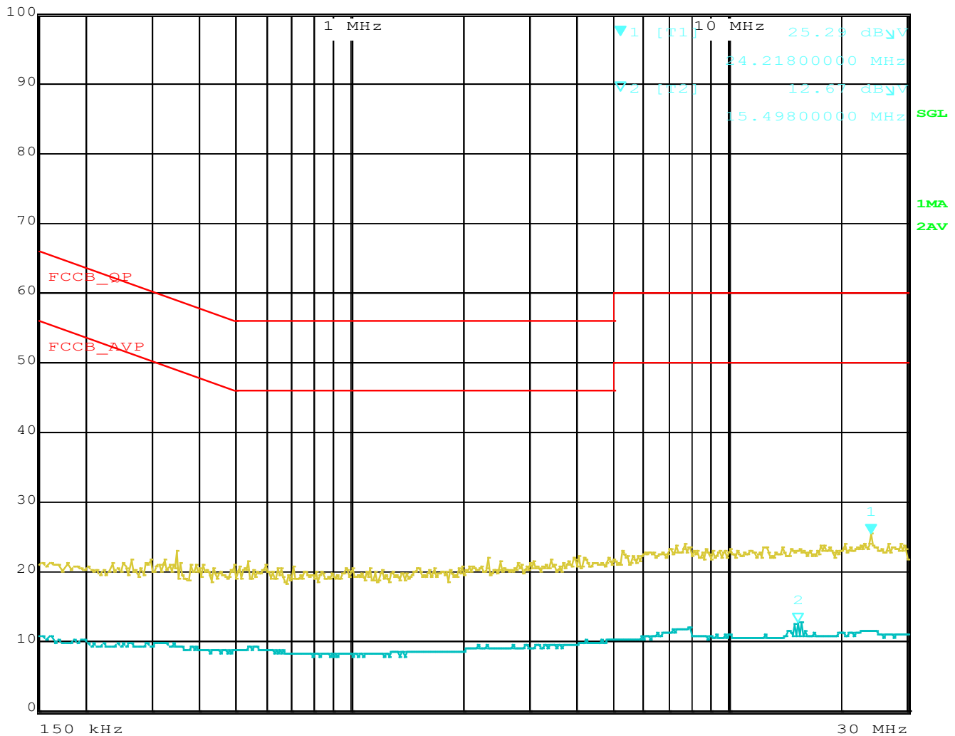
Figure 28 - Conducted Emissions Plot, - Ve Lead
