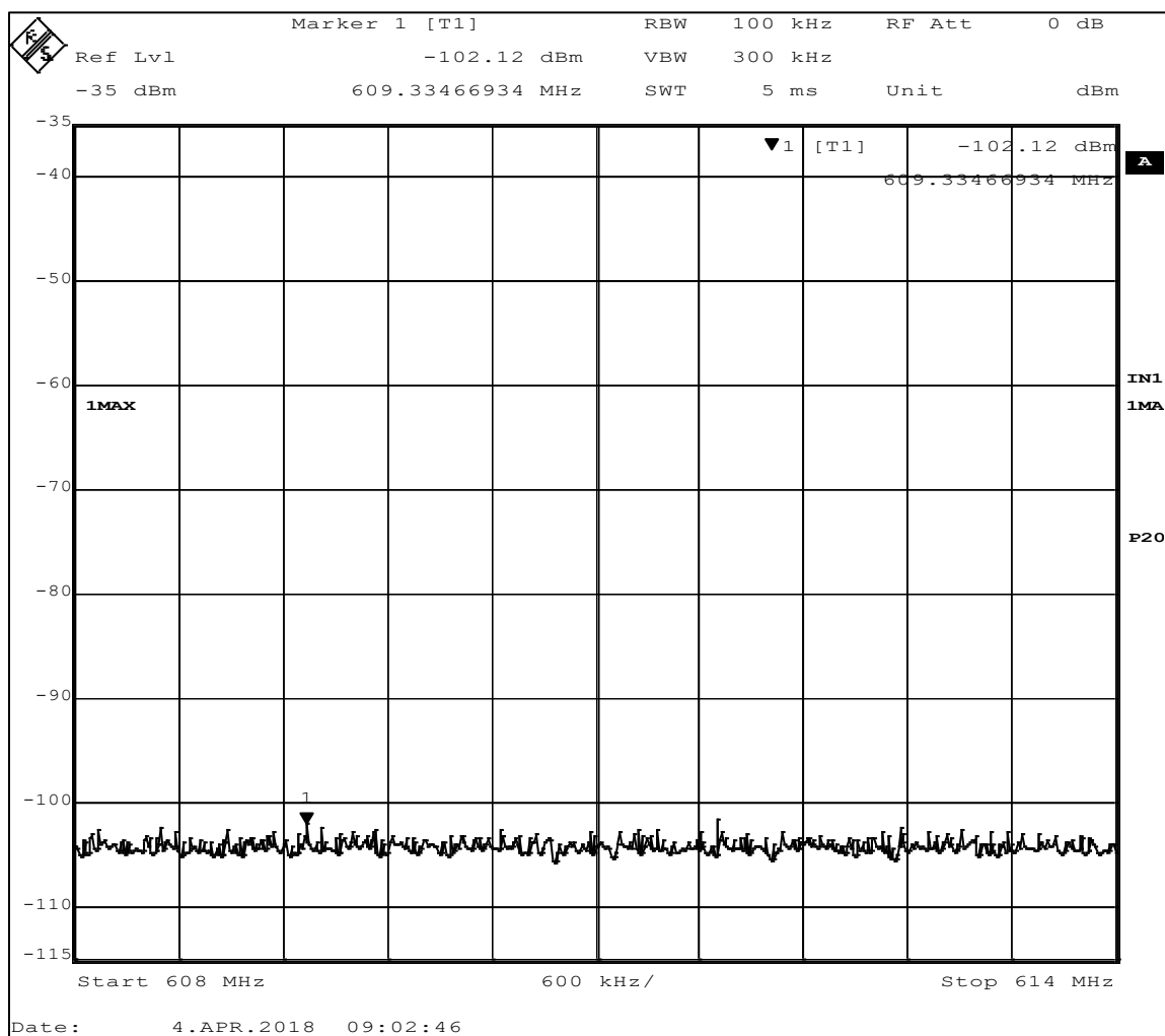
Figure 15 - Band-edge Measurement, Low Channel, Restricted Frequency, Continuous Transmit
