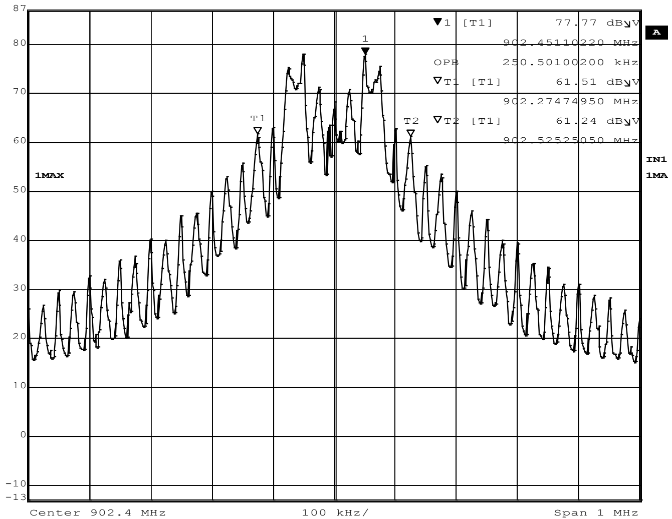
Figure 12 – Occupied Bandwidth, Low Channel. 250.50 kHz
