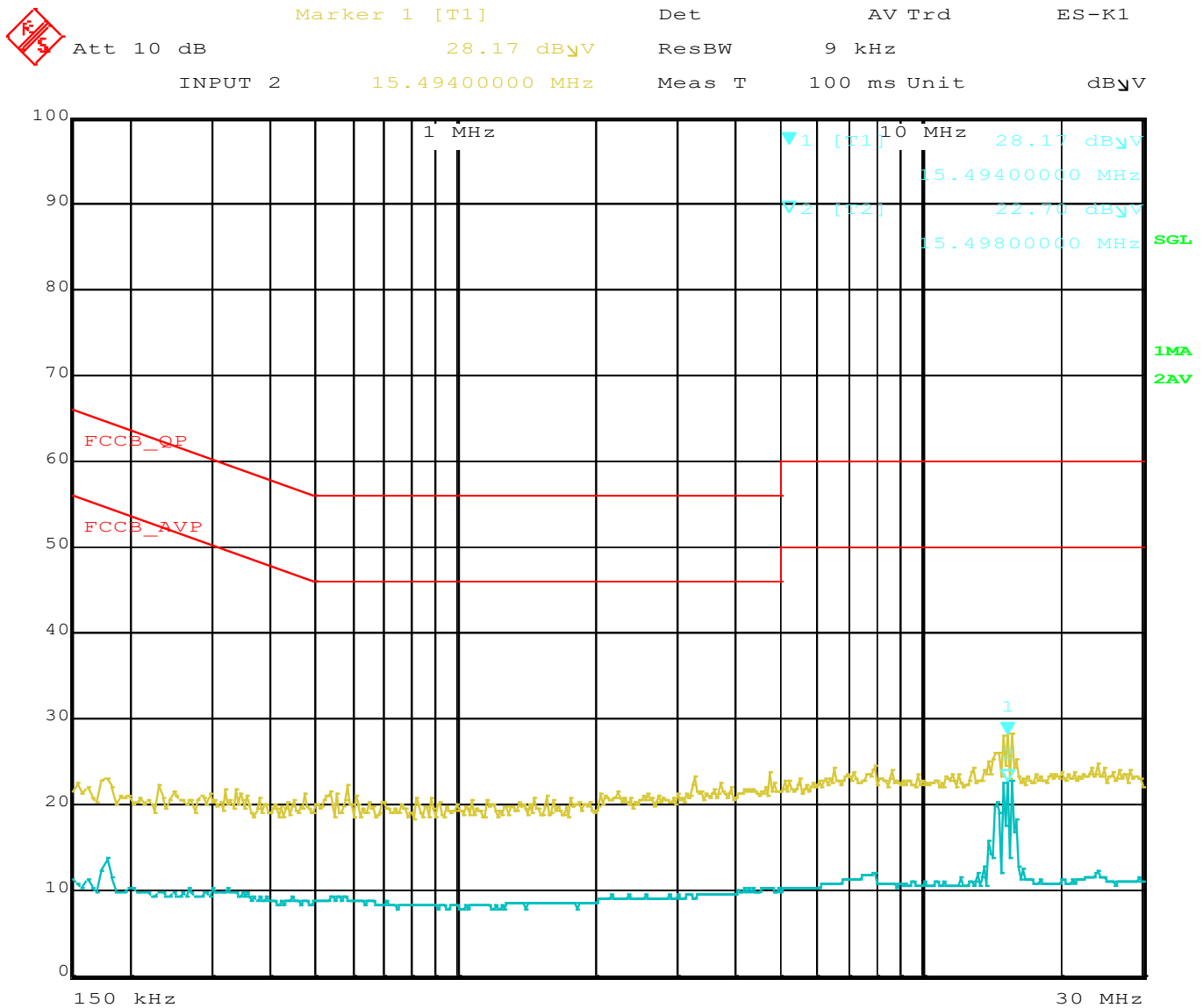
Figure 27 - Conducted Emissions Plot, +Ve Lead
