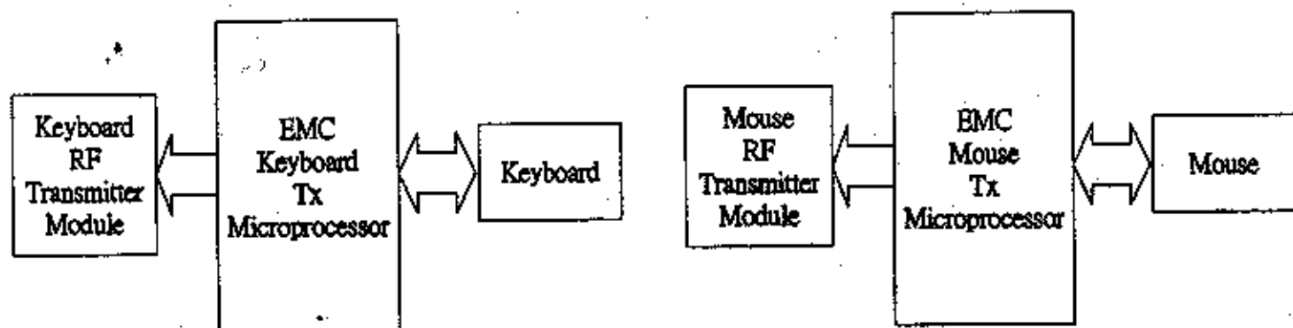
Fig.2 Mouse Block
