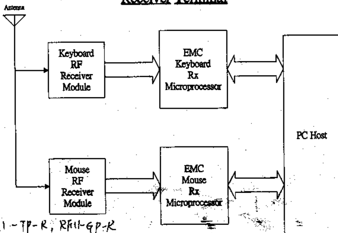
Fig.3 Receiver Block
