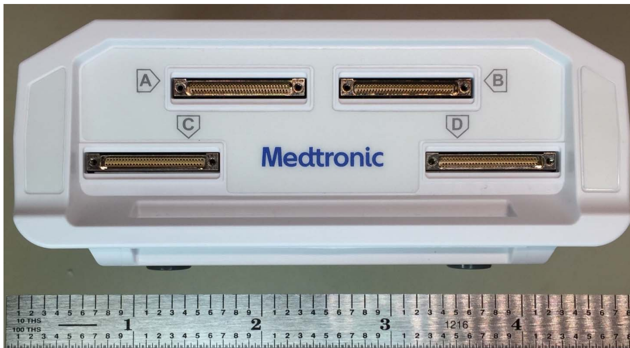
Figure 4 : External Neurostimulator, Model: 4NR003, Front View
