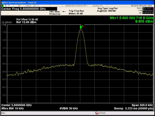
NT/NV_Antenna 0 IEEE 802.11a_Channel 120_20MHz
