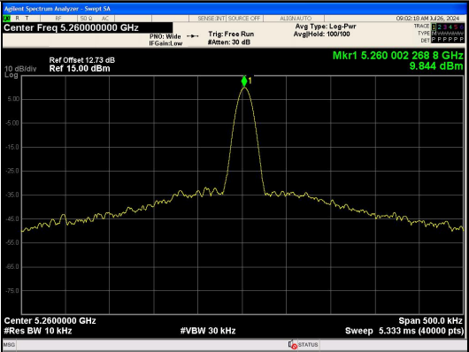
NT/NV_Antenna 0 IEEE 802.11a_Channel 52_20MHz
