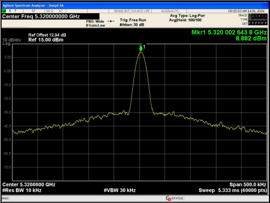
NT/NV_Antenna 0 IEEE 802.11a_Channel 64_20MHz
