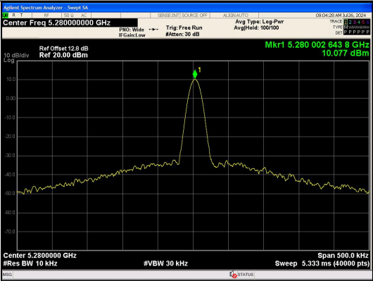
NT/NV_Antenna 0 IEEE 802.11a_Channel 56_20MHz
