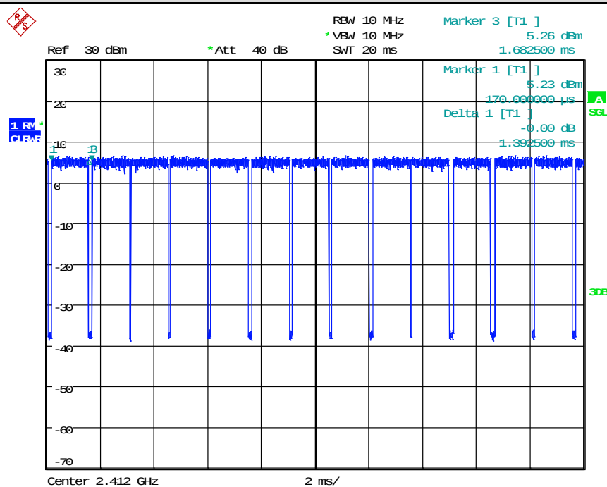
Test Graph_IEEE802.11g Duty Cycle:
