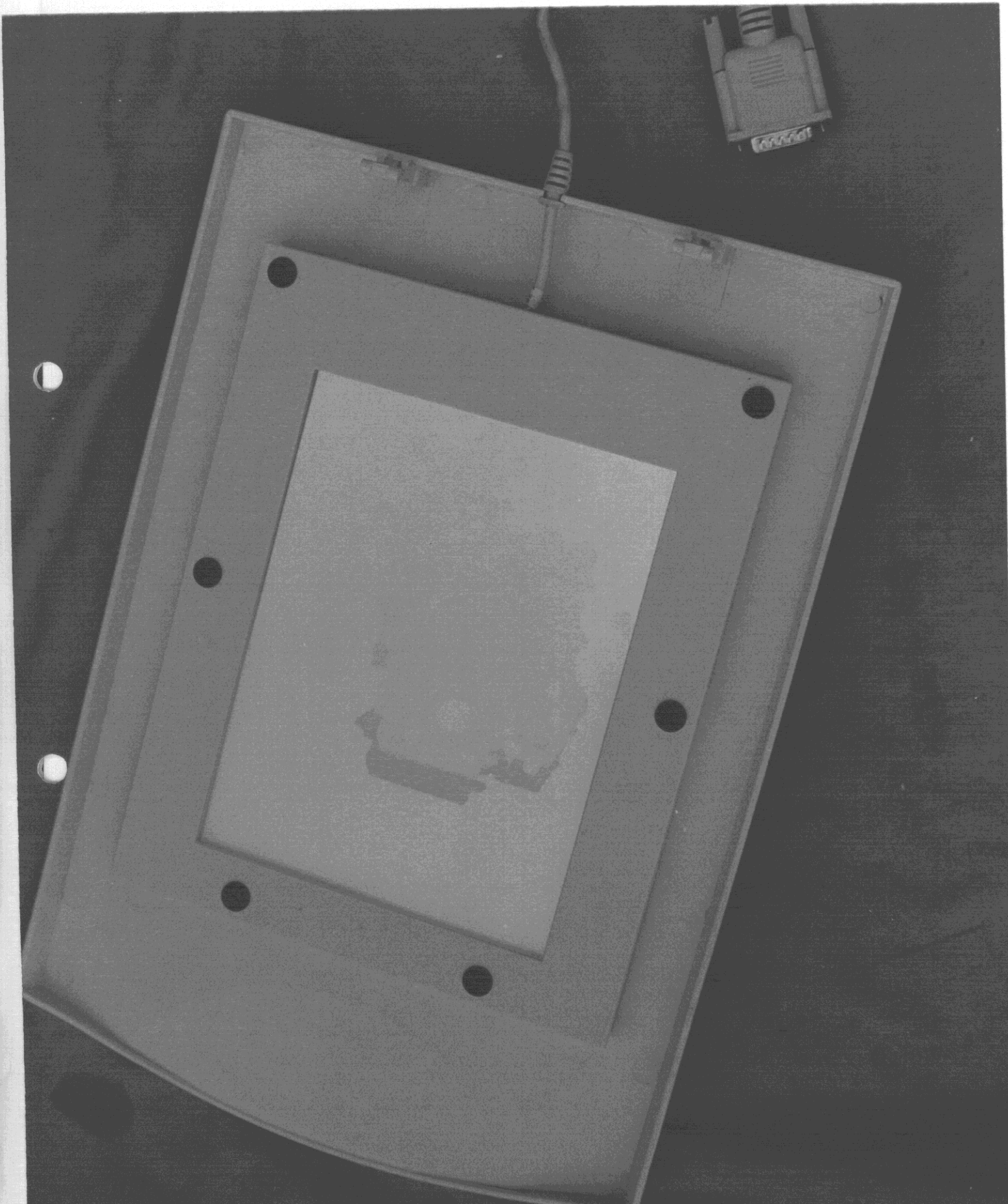
Figure 19 Back View of Light Plate
