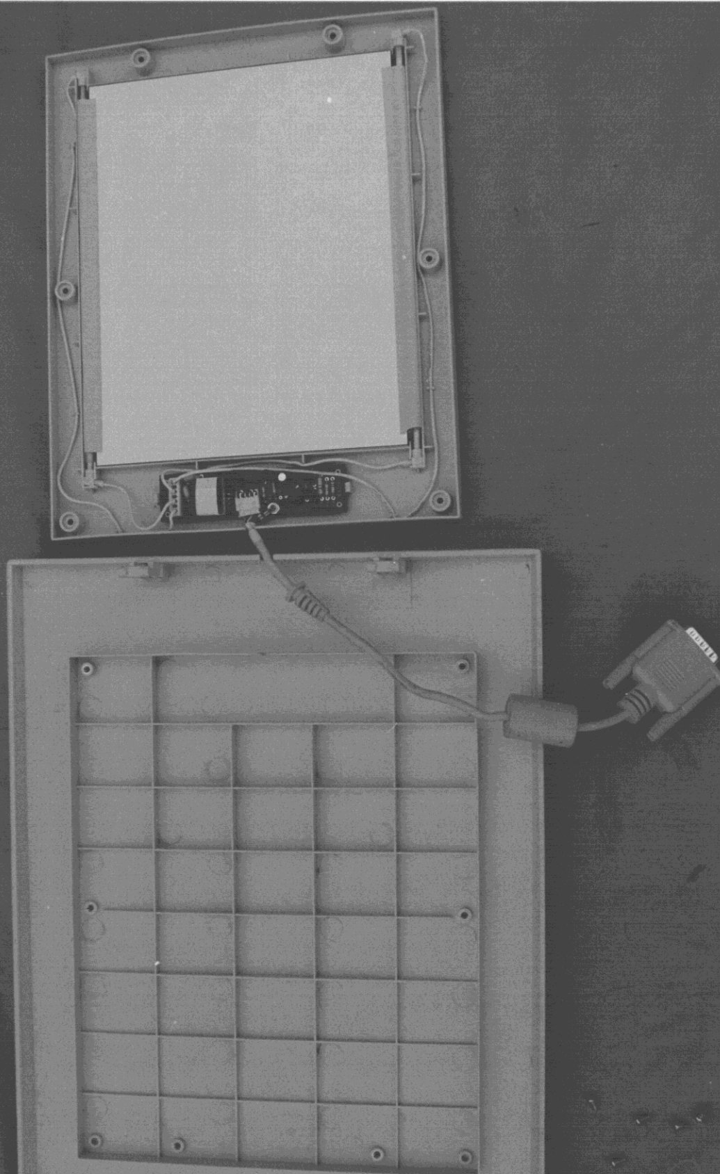
Figure 21 Top Cover, Internal View of Light Plate
