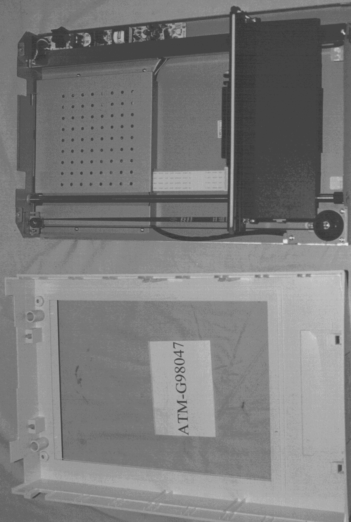
Figure 6 Top Cover Removed, Frame of Internal
