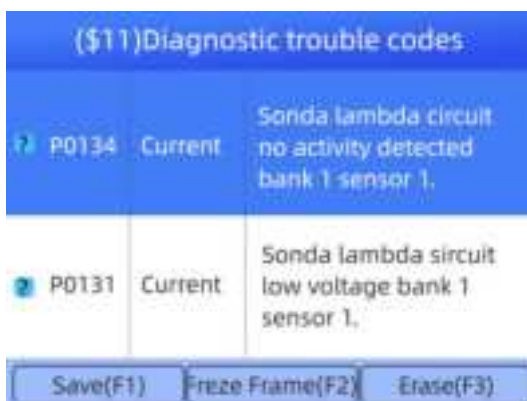
Figure 5-15 Sample Diagnostic Menu Screen
