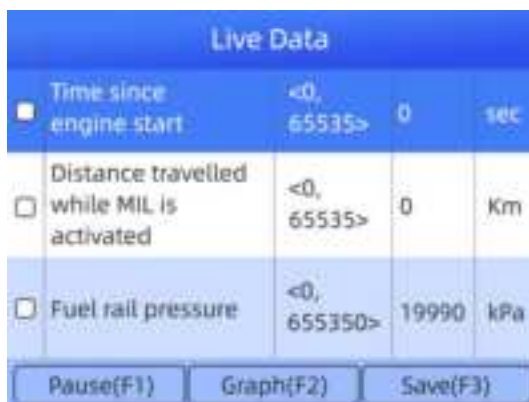
Figure 5-14 Sample Data stream Screen
