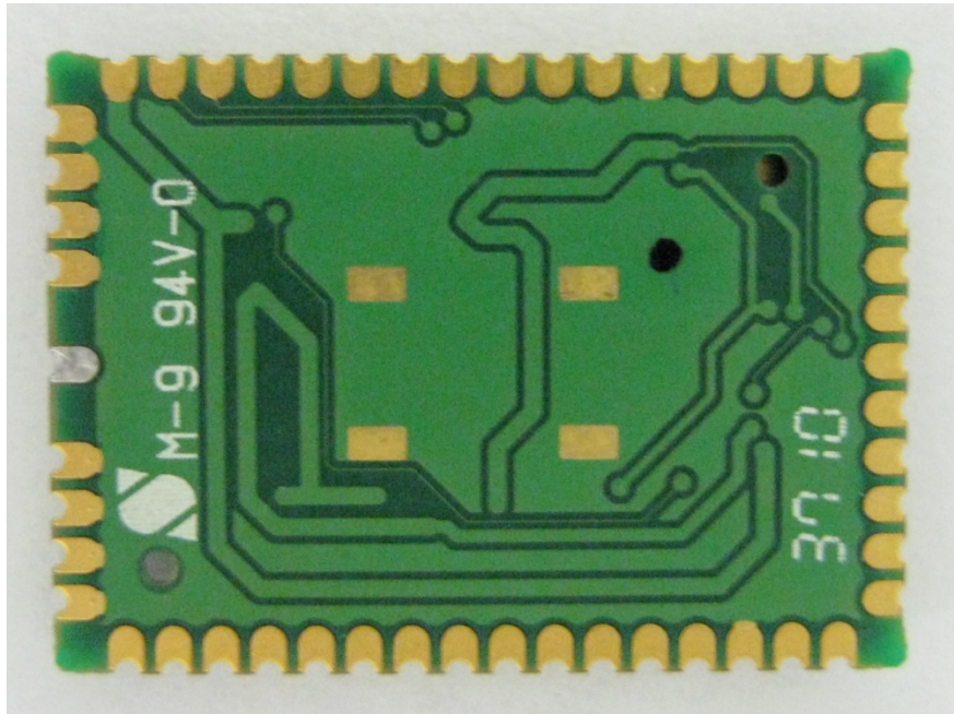
Back side of TiWi-R2 Module
