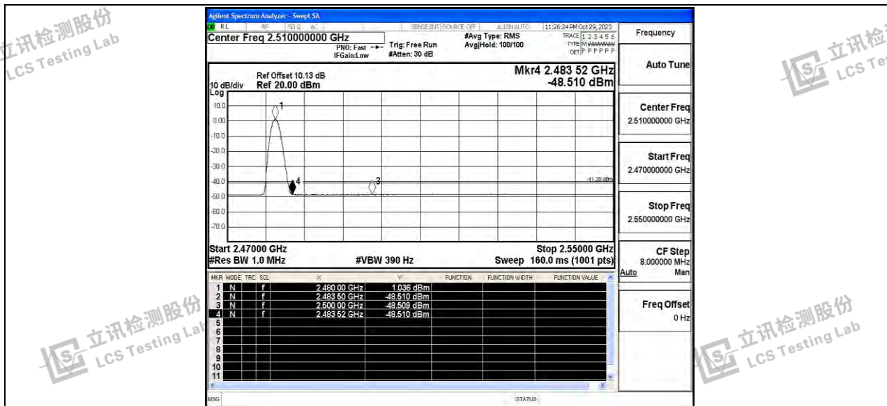
DH5_Ant_High_2480_Peak
