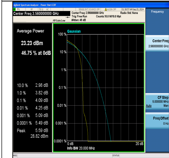
Band7-20MHz-16QAM-21350-1RB#0-PASS
