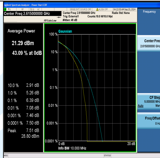
Band38-10MHz-16QAM-38200-50RB#0-PASS
