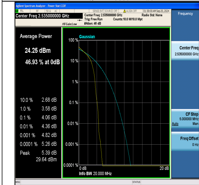
Band7-20MHz-QPSK-21100-1RB#0-PASS
