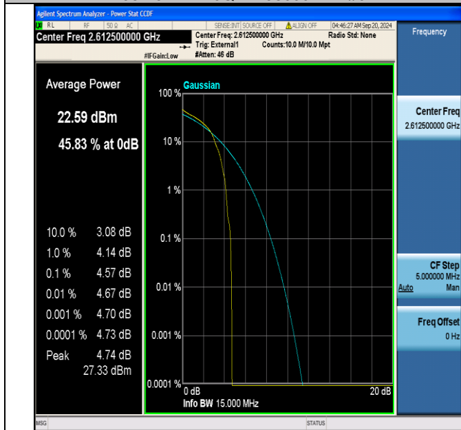
Band38-15MHz-16QAM-38175-1RB#0-PASS
