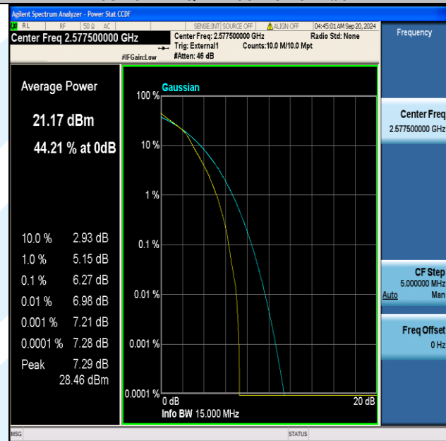
Band38-15MHz-16QAM-37825-75RB#0-PASS
