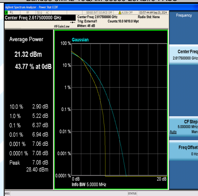
Band38-5MHz-16QAM-38225-25RB#0-PASS
