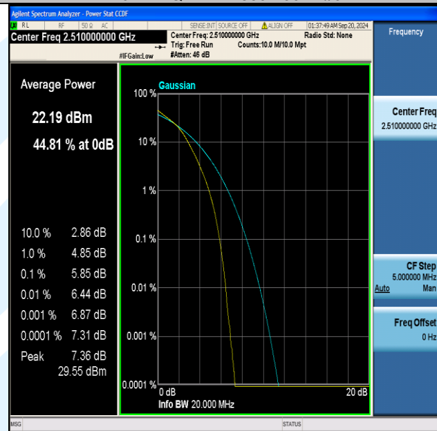
Band7-20MHz-16QAM-20850-100RB#0-PASS
