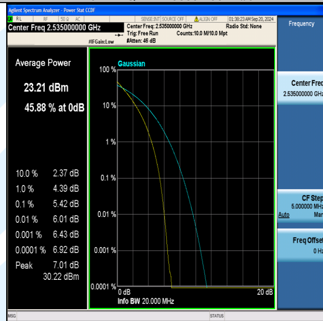
Band7-20MHz-QPSK-21100-100RB#0-PASS
