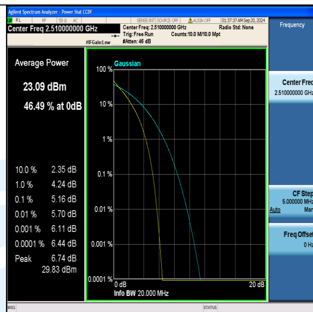
Band7-20MHz-QPSK-20850-100RB#0-PASS
