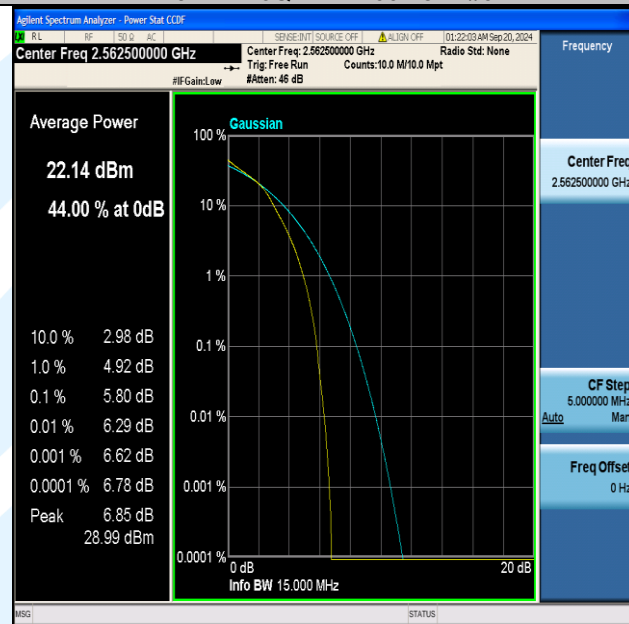
Band7-15MHz-16QAM-21375-75RB#0-PASS
