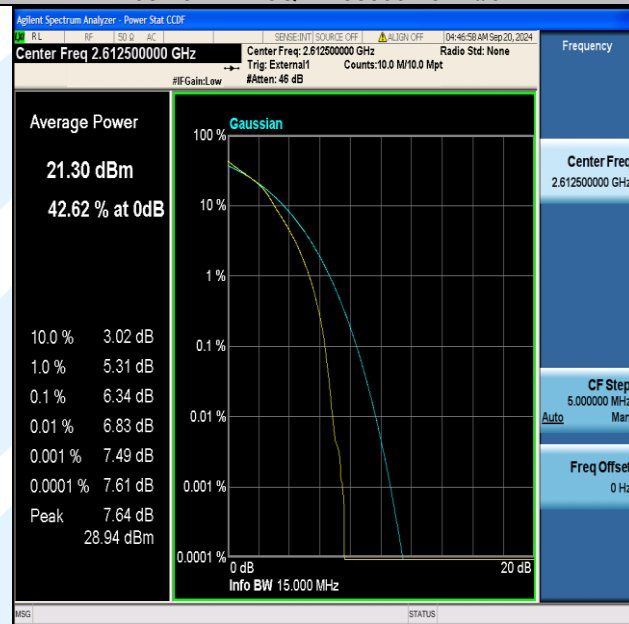
Band38-15MHz-16QAM-38175-75RB#0-PASS
