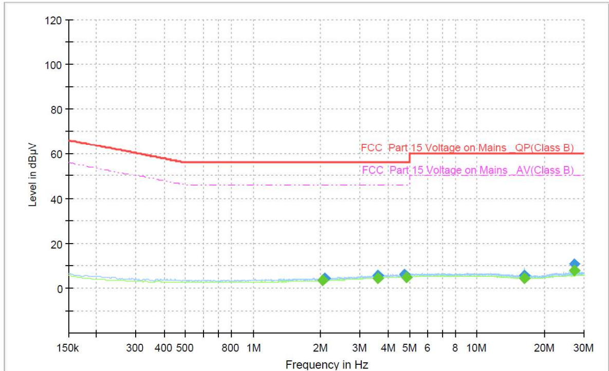
Figure 2: Spectral Diagrams, Conducted Emission, 150kHz - 30MHz, N
