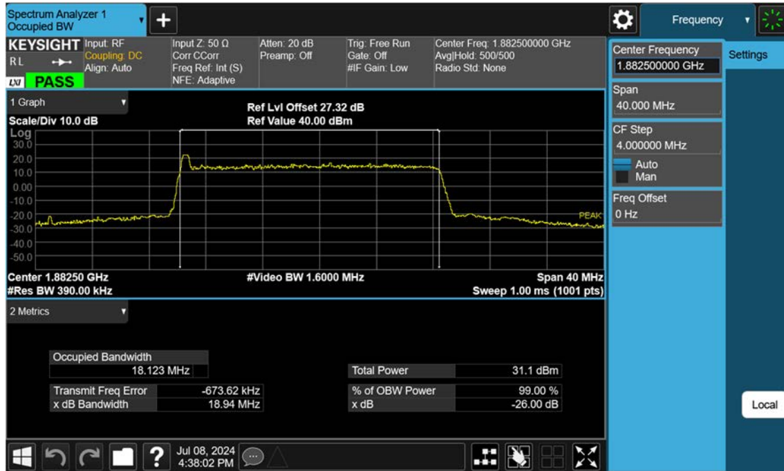
Sub6 n25(2)_20 M_OBW_Mid_QPSK_FullRB
