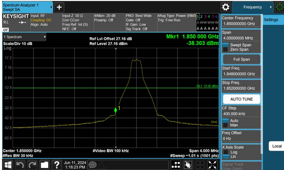
Sub6 n25(2)_10 M_Band Edge_Low_BPSK_1RB
