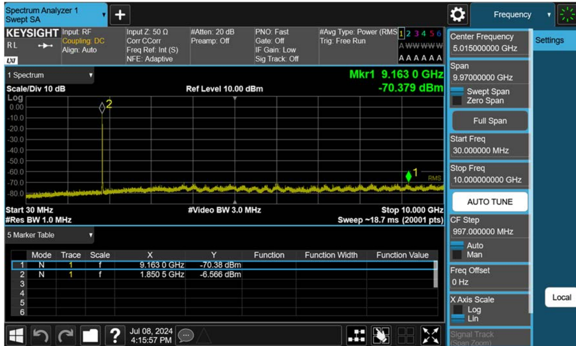
Sub6 n25(2)_5 M_Conducted Spurious(30 M-10 G)_Low_BPSK_1RB
