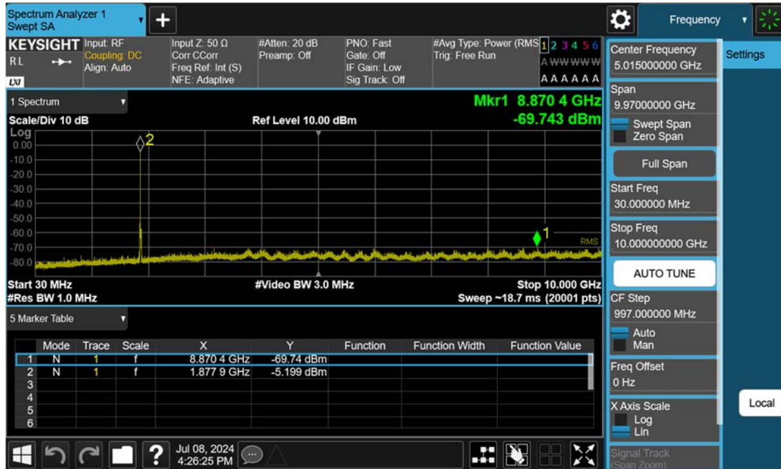
Sub6 n25(2)_10 M_Conducted Spurious(30 M-10 G)_Mid_BPSK_FullRB
