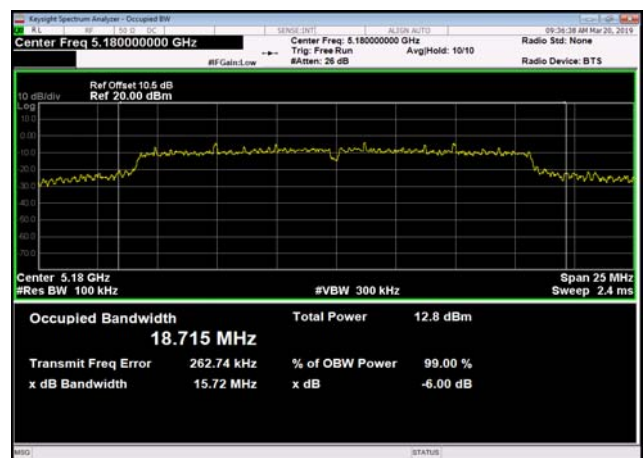
U-NII-1 6dB Bandwidth-802.11a(20MHz) ,5180MHz,Ant1
