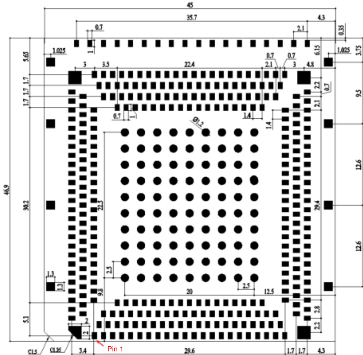
Figure 41: Recommended Footprint (Top View, Unit: mm)
