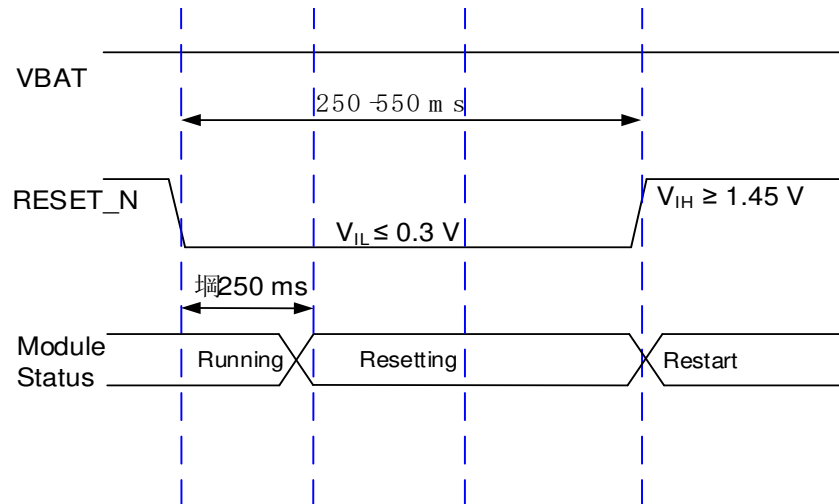
Figure 14: Reset Timing
