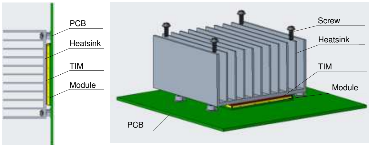
Figure 38: Placement and Fixing of the Heatsink
