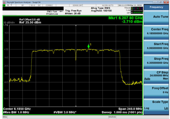
Plot 7-432. LPI Power Spectral Density Plot Antenna WF7a (160MHz 802.11ax RU996x2 (UNII Band 5) – Ch. 47)
