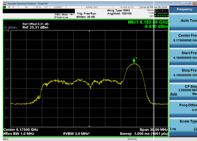
Plot 7-419. LPI Power Spectral Density Plot Antenna WF7a (20MHz 802.11ax RU26 (UNII Band 5) – Ch. 45)
