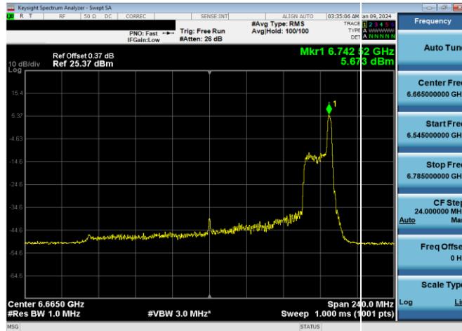
Plot 7-413. SP Power Spectral Density Plot CDD Diversity Antenna WF2a (160MHz 802.11ax RU26 (UNII Band 7) – Ch. 143)
