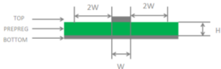
Figure 7: Microstrip Design on a 2-layer PCB
