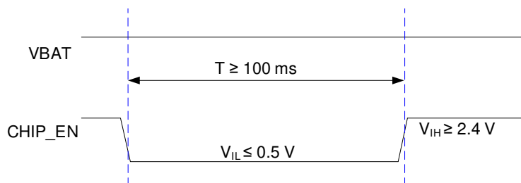
Figure 5: Reset Timing
