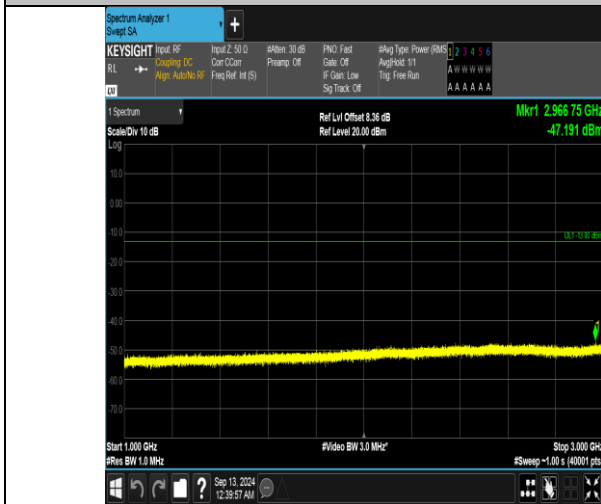
Band5_10MHz_16QAM_20600_50RB#0_1000~3000_1000~3000
