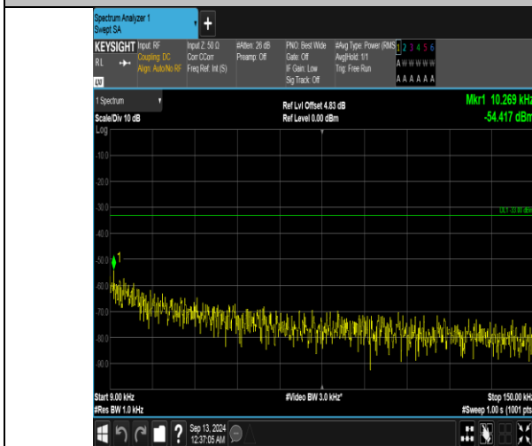
Band5_10MHz_QPSK_20600_1RB#49_0.009~0.15_0.009~0.15
