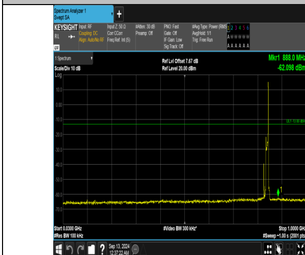
Band5_10MHz_QPSK_20600_1RB#49_30~1000_30~1000
