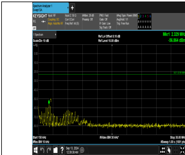
Band5_10MHz_16QAM_20600_50RB#0_0.15~30_0.15~30
