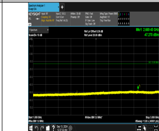
Band5_10MHz_QPSK_20600_1RB#49_1000~3000_1000~3000
