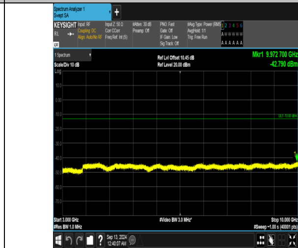
Band5_10MHz_16QAM_20600_50RB#0_3000~10000_3000~10000
