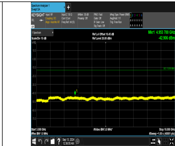
Band5_10MHz_16QAM_20600_1RB#0_3000~10000_3000~10000
