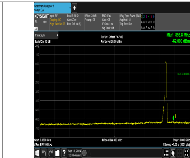
Band5_10MHz_16QAM_20600_50RB#0_30~1000_30~1000
