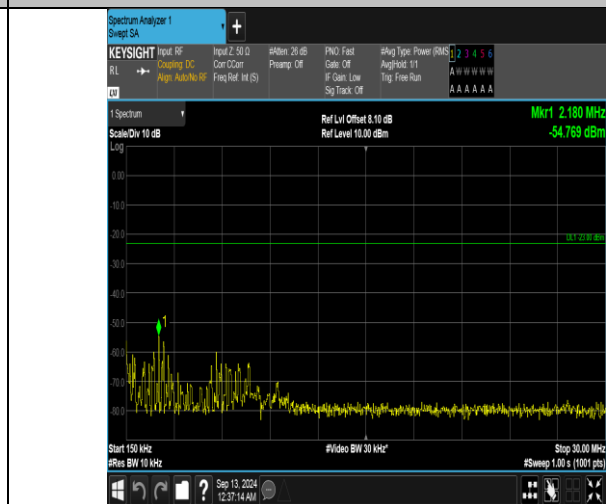
Band5_10MHz_QPSK_20600_1RB#49_0.15~30_0.15~30
