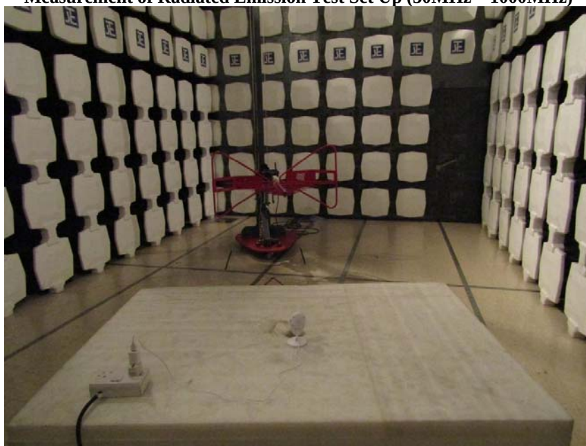
Measurement of Radiated Emission Test Set Up (30MHz – 1000MHz)
