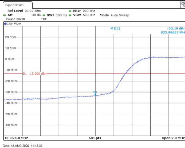
Band5-10MHz-QPSK-20600-1RB#0
