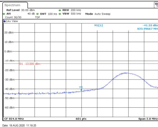
Band5-10MHz-16QAM-20450-50RB#0
