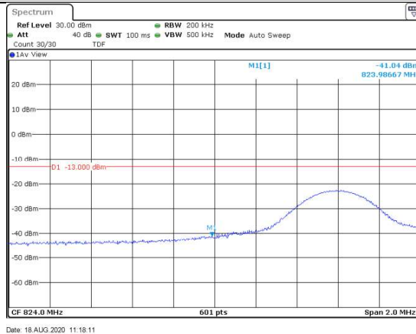
Band5-10MHz-QPSK-20450-50RB#0
