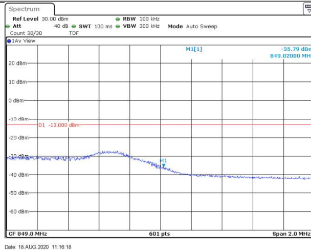
Band5-5MHz-QPSK-20625-25RB#0
