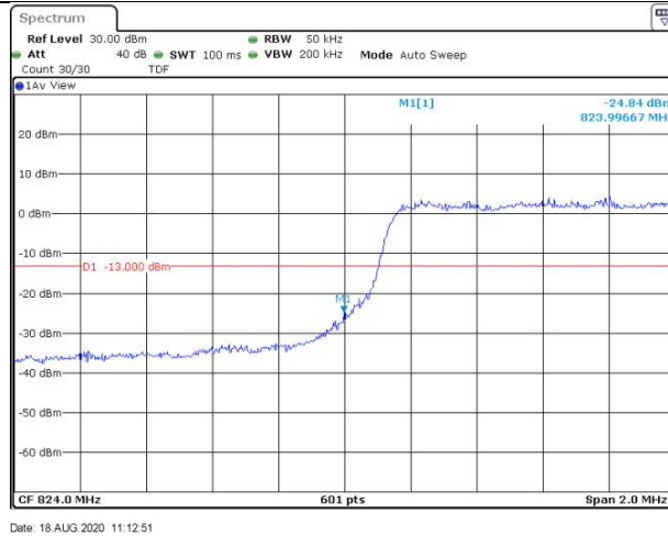
Band5-3MHz-16QAM-20635-1RB#0
