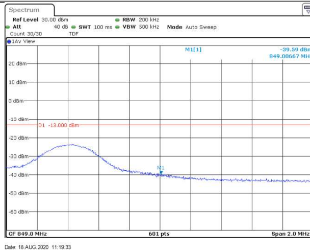
Band5-10MHz-16QAM-20600-1RB#49
