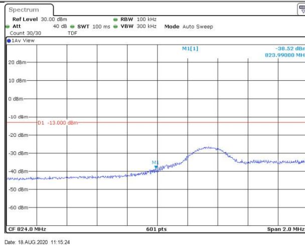
Band5-5MHz-16QAM-20425-1RB#0
