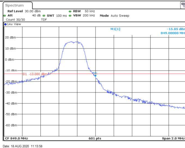
Band5-3MHz-16QAM-20635-15RB#0
