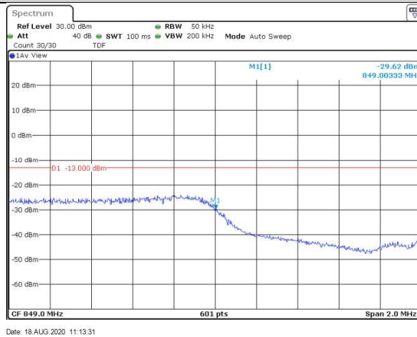
Band5-3MHz-16QAM-20635-1RB#14
