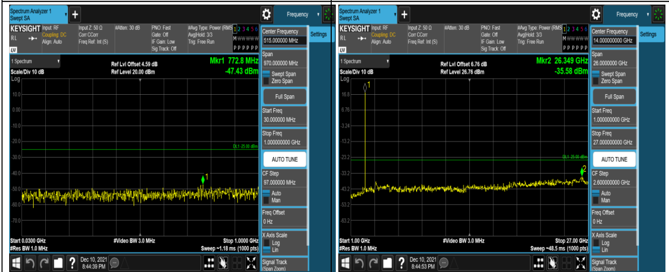
Band7-5MHz-QPSK-21425-1RB#0-Range1:30~100 OMHz
