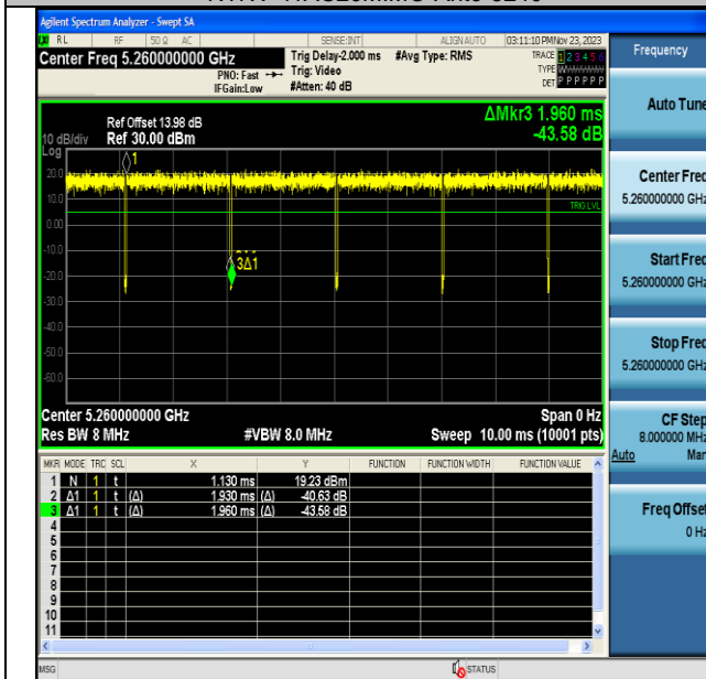
NTNV-11AC20MIMO-Ant6-5260
