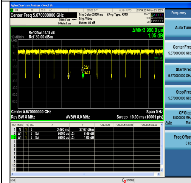
NTNV-11AC40MIMO-Ant6-5670
