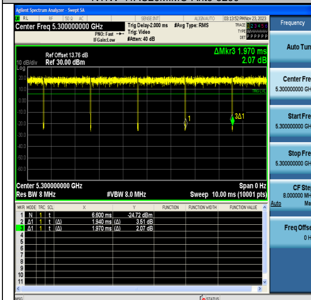
NTNV-11AC20MIMO-Ant6-5300
