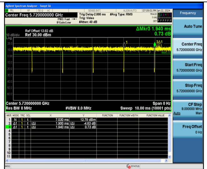
NTNV-11AC20MIMO-Ant7-5720
