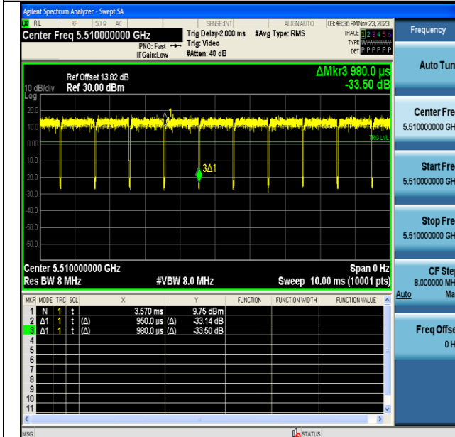
NTNV-11AC40MIMO-Ant6-5510
