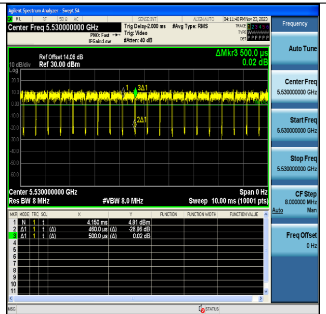
NTNV-11AC80MIMO-Ant7-5530
