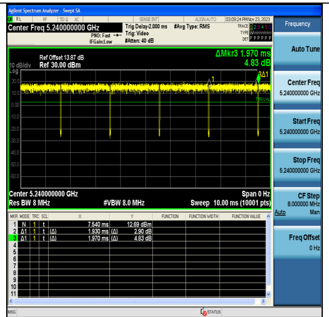
NTNV-11AC20MIMO-Ant7-5240
