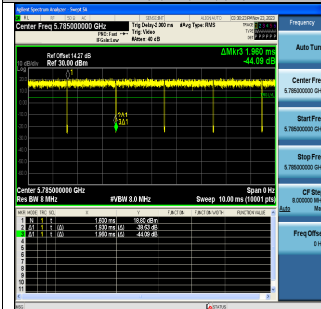
NTNV-11AC20MIMO-Ant6-5785
