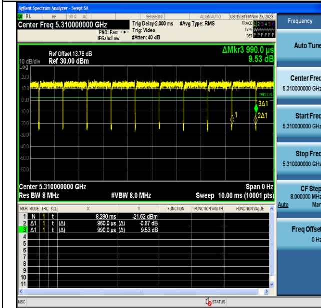
NTNV-11AC40MIMO-Ant6-5310
