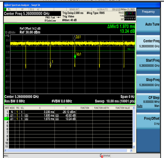
NTNV-11AC20MIMO-Ant7-5260
