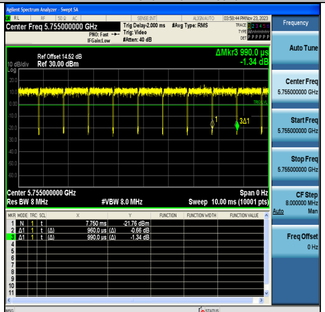
NTNV-11AC40MIMO-Ant7-5755
