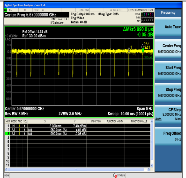
NTNV-11AC40MIMO-Ant7-5670
