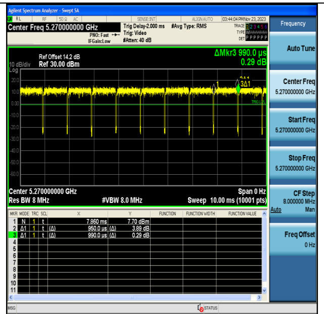
NTNV-11AC40MIMO-Ant7-5270
