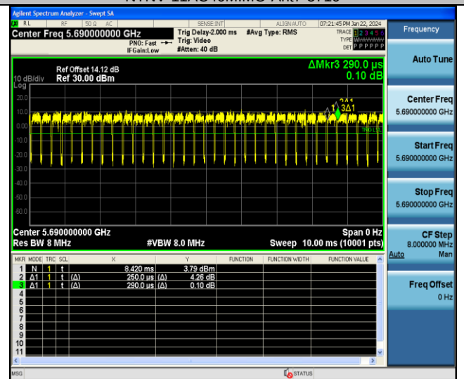
NTNV-11AC80MIMO-Ant7-5690
