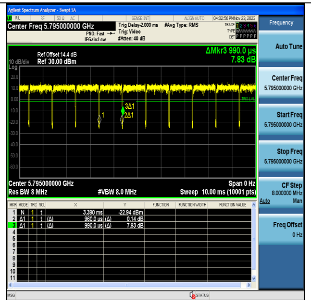
NTNV-11AC40MIMO-Ant7-5795
