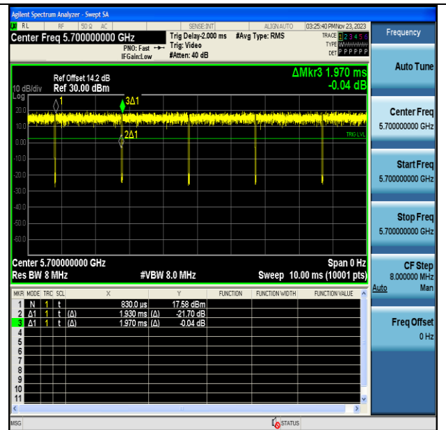
NTNV-11AC20MIMO-Ant7-5700
