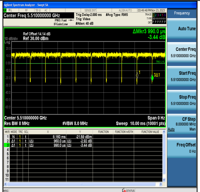
NTNV-11AC40MIMO-Ant7-5510
