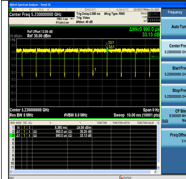
NTNV-11AC40MIMO-Ant6-5230
