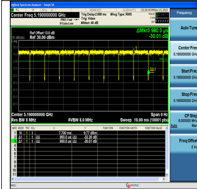
NTNV-11AC40MIMO-Ant6-5190
