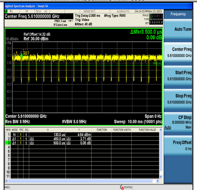
NTNV-11AC80MIMO-Ant7-5610
