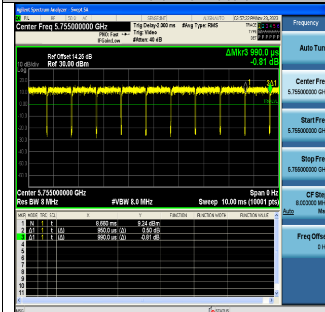
NTNV-11AC40MIMO-Ant6-5755
