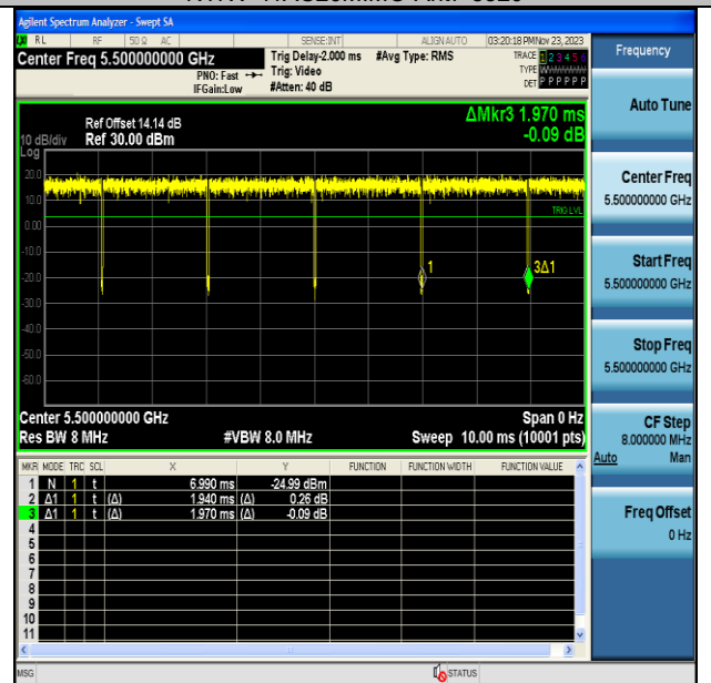
NTNV-11AC20MIMO-Ant7-5500
