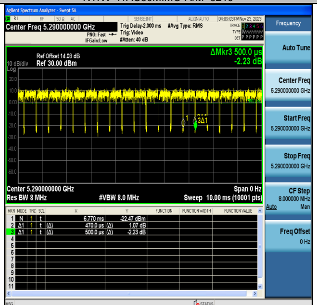
NTNV-11AC80MIMO-Ant7-5290
