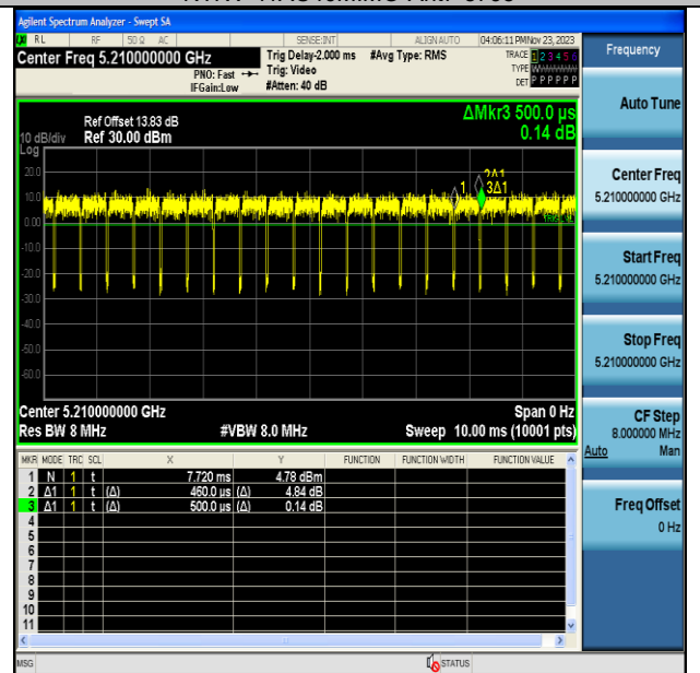
NTNV-11AC80MIMO-Ant7-5210
