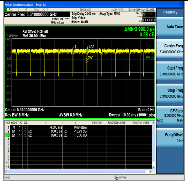
NTNV-11AC40MIMO-Ant7-5310
