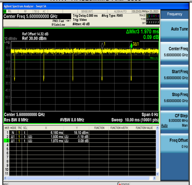
NTNV-11AC20MIMO-Ant7-5600
