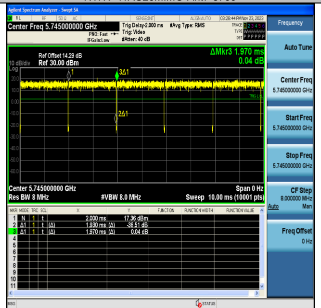
NTNV-11AC20MIMO-Ant7-5745
