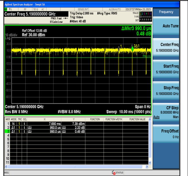
NTNV-11AC40MIMO-Ant7-5190
