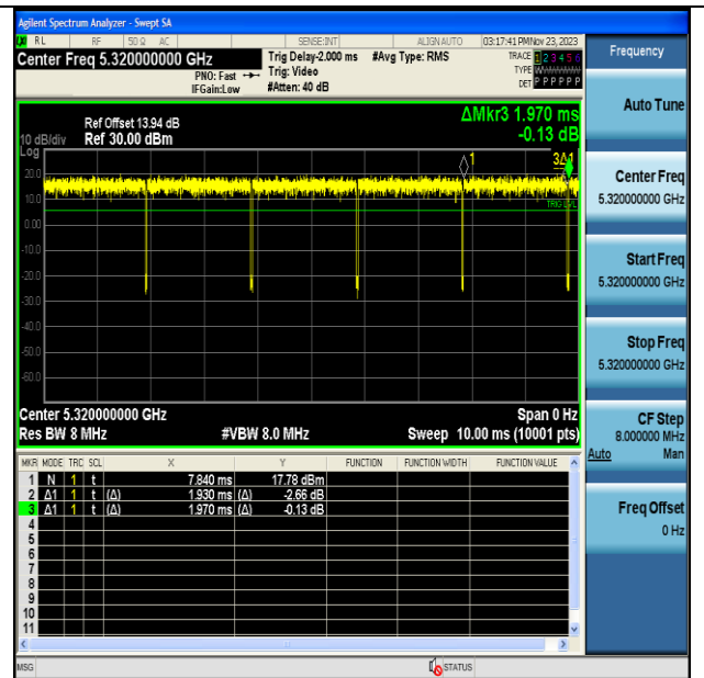
NTNV-11AC20MIMO-Ant7-5320
