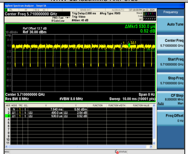
NTNV-11AC40MIMO-Ant7-5710
