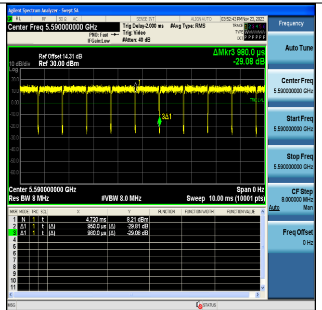
NTNV-11AC40MIMO-Ant7-5590
