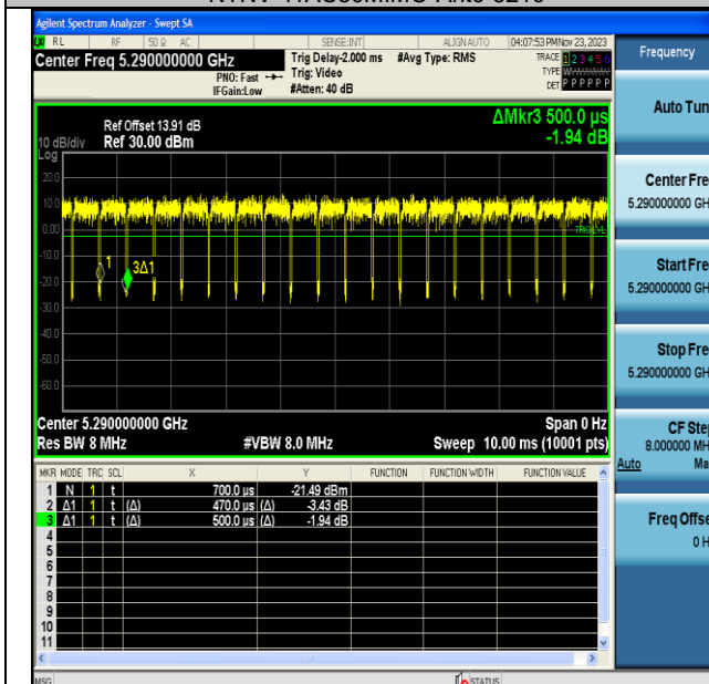
NTNV-11AC80MIMO-Ant6-5290
