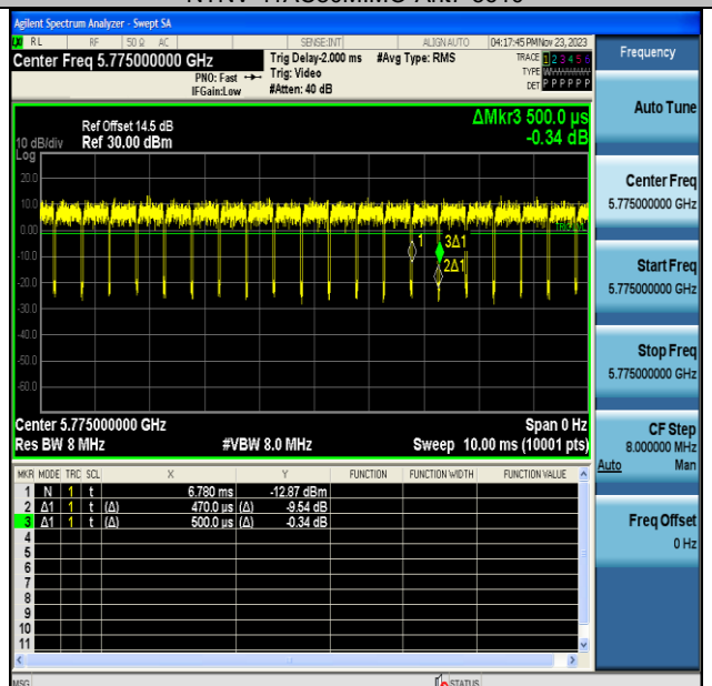
NTNV-11AC80MIMO-Ant7-5775
