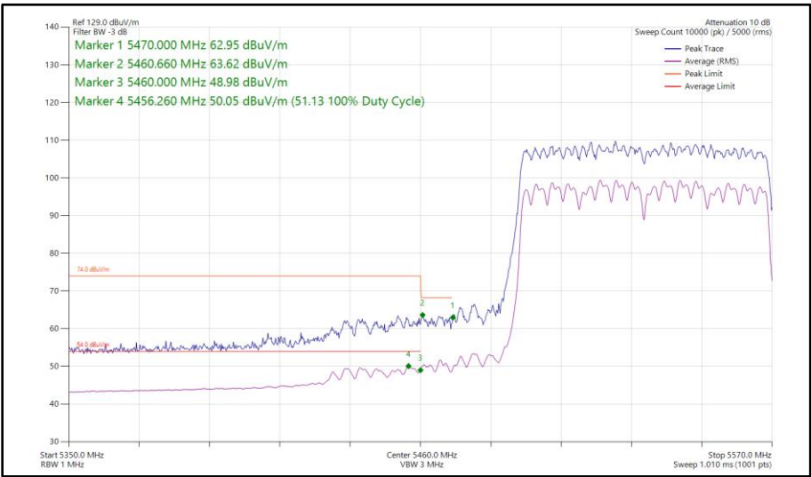
Figure 614 - 802.11ac VHT80, CDD, Core 0 - Core 1 - 5530 MHz Band Edge Frequency 5470 MHz
