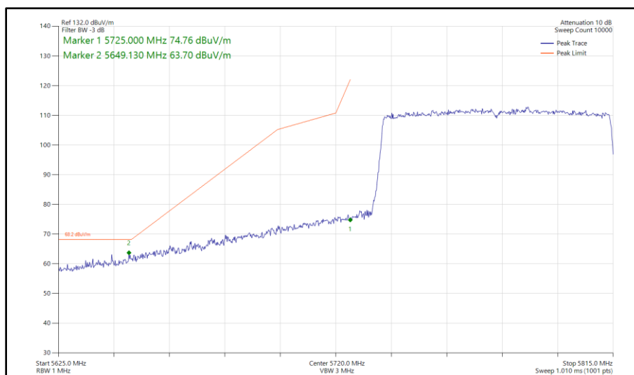
Figure 588 - 802.11ax HE80, SU, SISO, Core 0 - 5775 MHz Band Edge Frequency 5725 MHz
