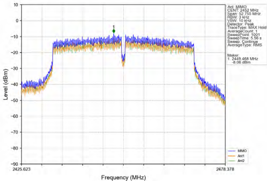
802.11ac(VHT40)_HCH_2452MHz_MIMO_NTNV
