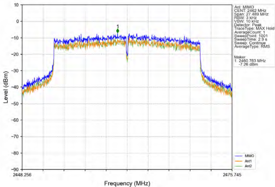
802.11ax(HEW20)_HCH_2462MHz_RU242_Left_MIMO_NTNV
