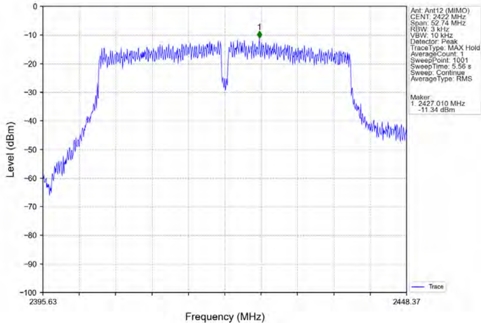
802.11ac(VHT40)_LCH_2422MHz_MIMO_NTNV
