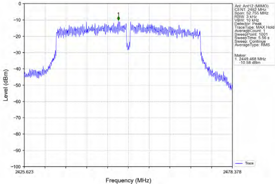
802.11ac(VHT40)_HCH_2452MHz_MIMO_NTNV
