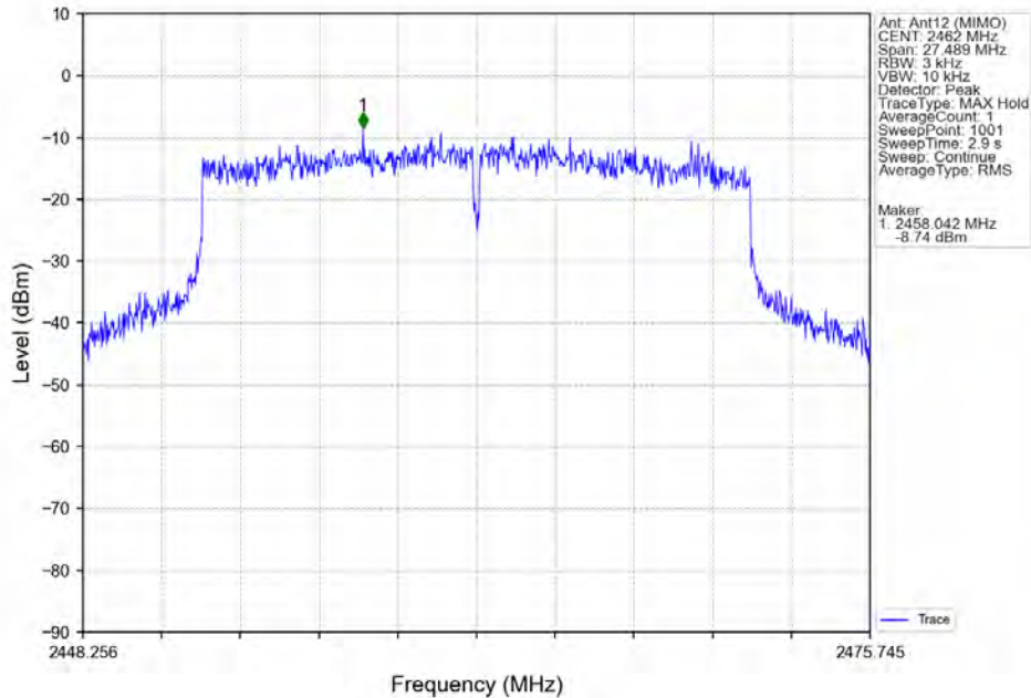
802.11ax(HEW20)_HCH_2462MHz_RU242_Left_MIMO_NTNV
