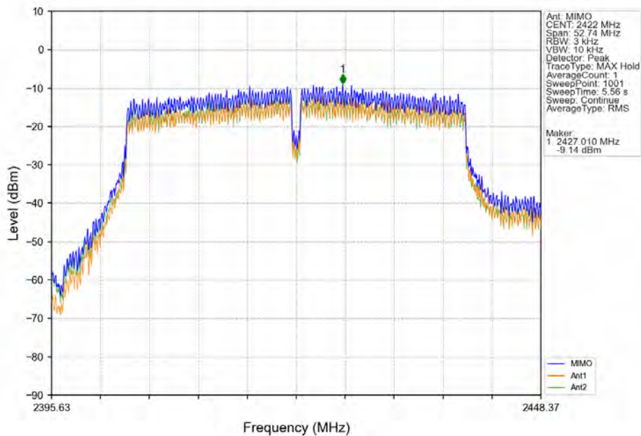
802.11ac(VHT40)_LCH_2422MHz_MIMO_NTNV
