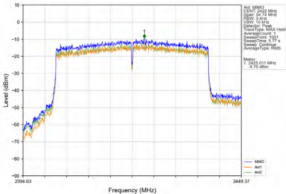
802.11ax(HEW40)_LCH_2422MHz_RU484_Left_MIMO_NTNV
