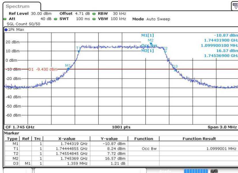
Band66-1.4MHz-QPSK-132322-6RB#0
