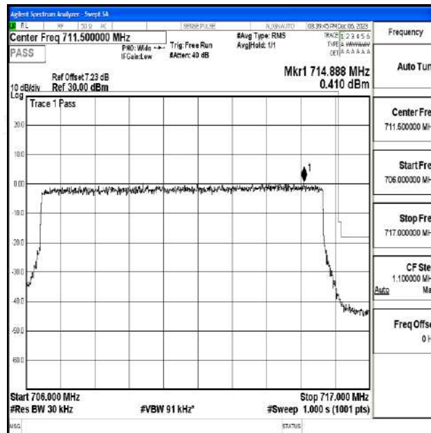
Band12_10MHz_QPSK_23130_50RB#0
