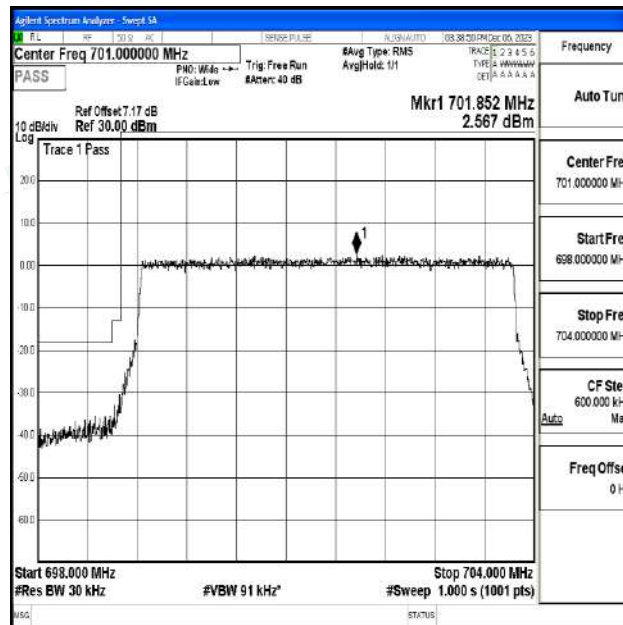
Band12_5MHz_QPSK_23035_25RB#0
