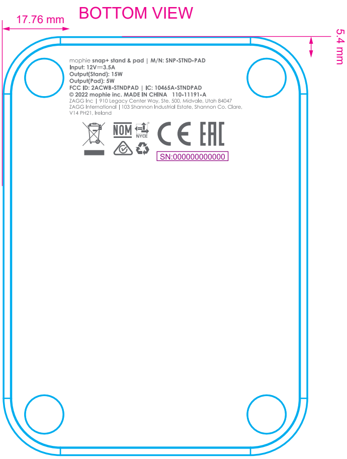
BOTTOM VIEW
