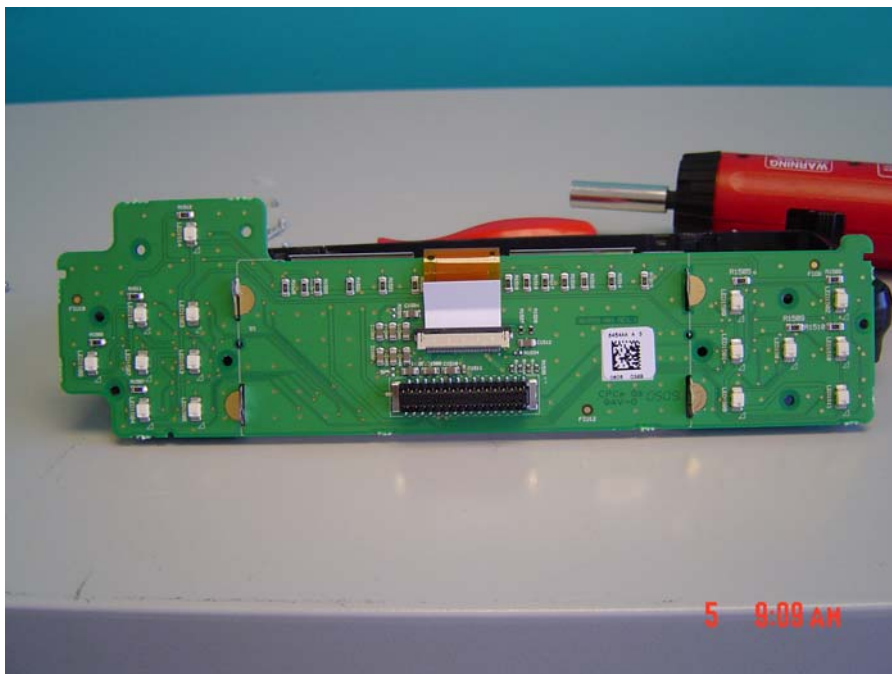
Head Unit – Faceplate PCB Rear View
