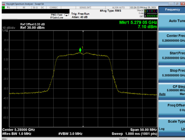
Plot 7-536. PSD SDM Antenna 3b (20MHz BW 802.11n – Ch. 56, MCS11)
