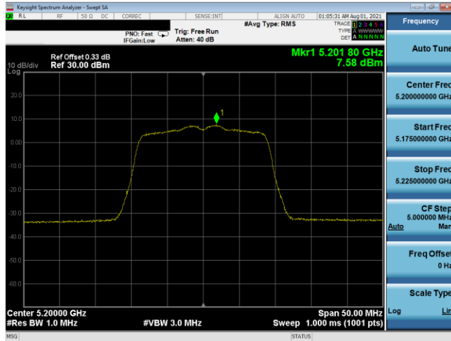
Plot 7-523. PSD SDM Antenna 5T (20MHz BW 802.11n - Ch. 40, MCS11)
