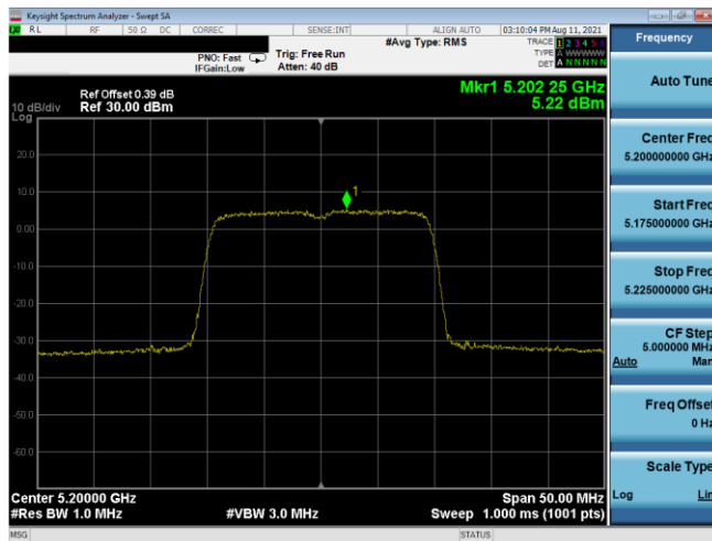
Plot 7-561. PSD SDM Antenna 5T (20MHz BW 802.11ax(SU) – Ch. 40, MCS5)
