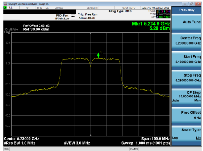
Plot 7-564. PSD SDM Antenna 3b (40MHz BW 802.11n – Ch. 46, MCS13)
