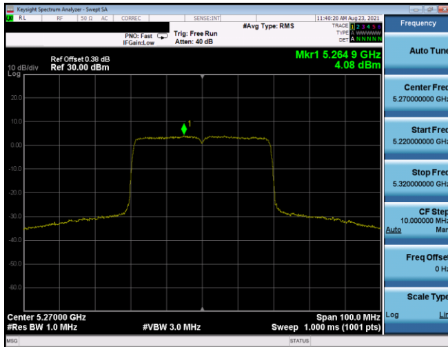
Plot 7-541. PSD SDM Antenna 5T (40MHz BW 802.11ax(SU) – Ch. 54, MCS3)
