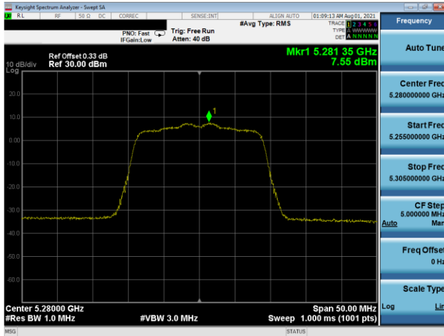
Plot 7-535. PSD SDM Antenna 5T (20MHz BW 802.11n – Ch. 56, MCS11)
