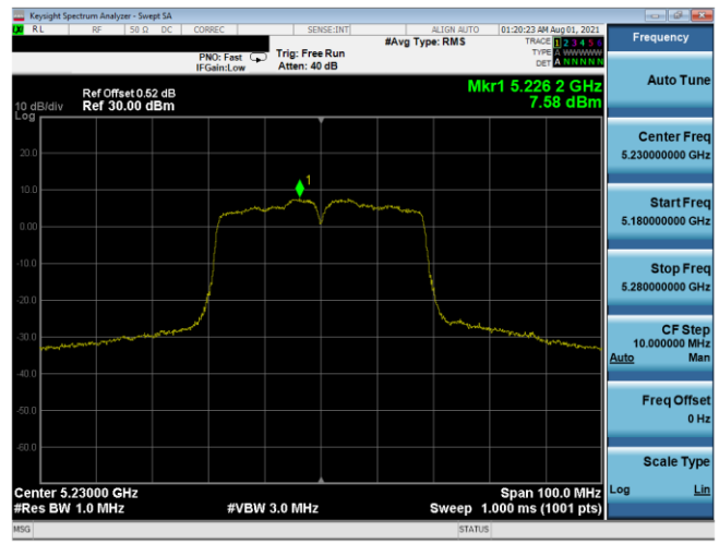
Plot 7-527. PSD SDM Antenna 5T (40MHz BW 802.11n - Ch. 46, MCS11)
