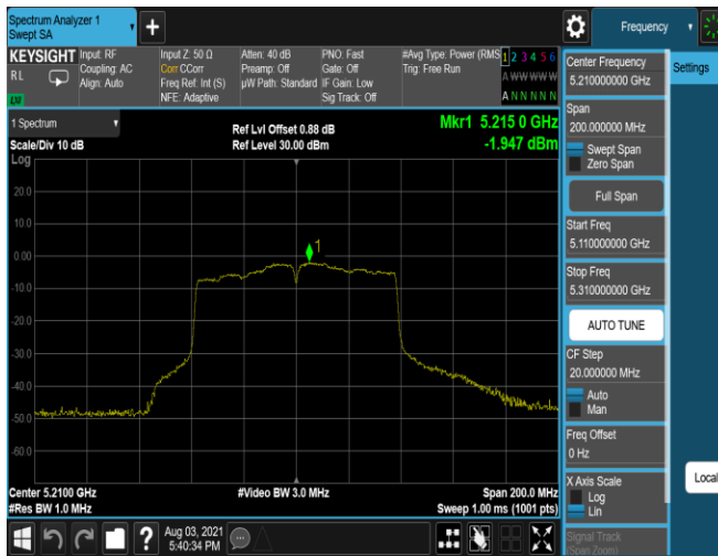
Plot 7-495. PSD CDD Antenna 5T (80MHz BW 802.11ac – Ch. 42, MCS2)
