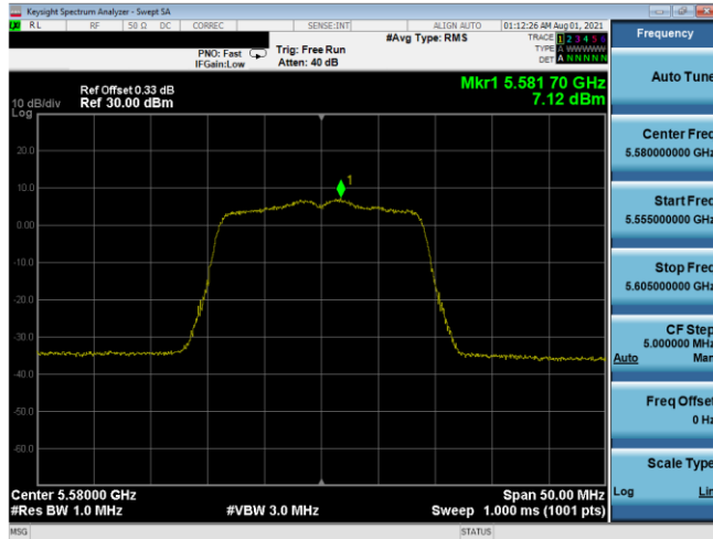
Plot 7-547. PSD CDD Antenna 5T (20MHz BW 802.11n – Ch. 116, MCS11)
