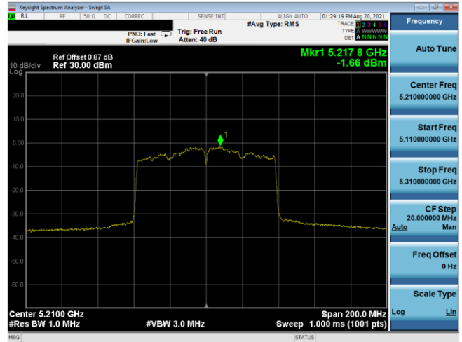
Plot 7-532. PSD CDD Antenna 3b (80MHz BW 802.11ac – Ch. 42, MCS3)
