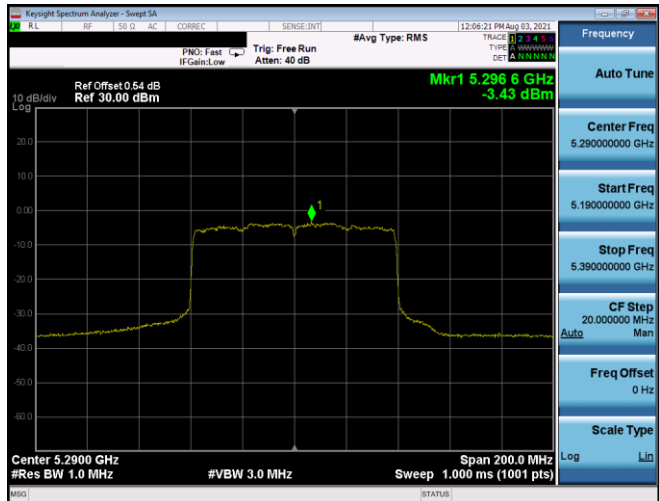
Plot 7-510. PSD CDD Antenna 3b (80MHz BW 802.11ax(SU) - Ch. 58, MCS2)
