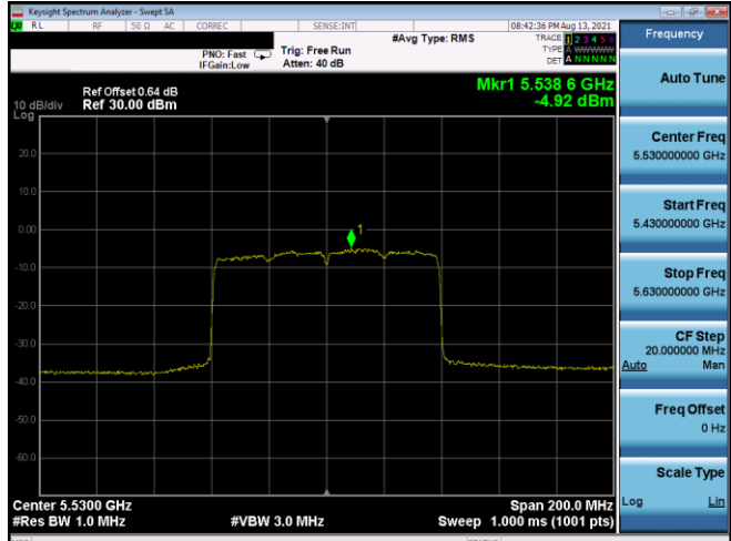
Plot 7-557. PSD CDD Antenna 5T (80MHz BW 802.11ax(SU) – Ch. 106, MCS3)
