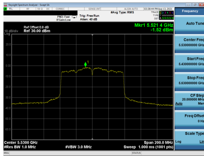
Plot 7-519. PSD CDD Antenna 5T (80MHz BW 802.11ac – Ch. 106, MCS2)
