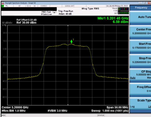
Plot 7-524. PSD SDM Antenna 3b (20MHz BW 802.11n - Ch. 40, MCS11)
