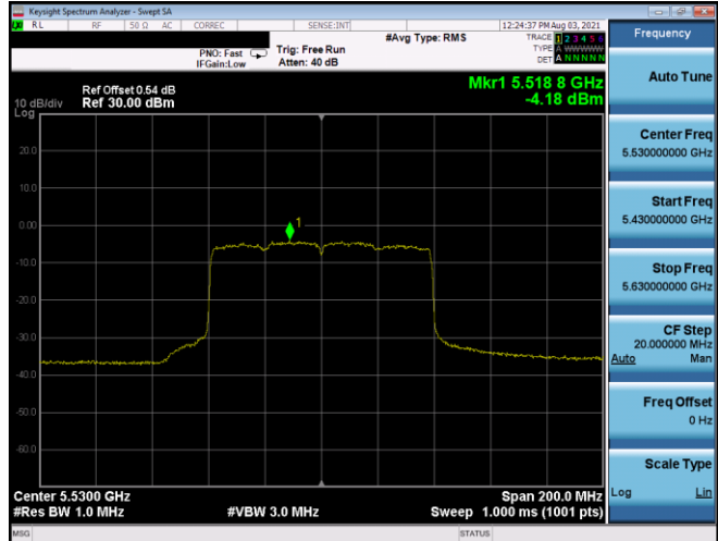
Plot 7-521. PSD CDD Antenna 5T (80MHz BW 802.11ax(SU) – Ch. 106, MCS2)
