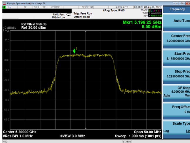
Plot 7-560. PSD SDM Antenna 3b (20MHz BW 802.11n – Ch. 40, MCS13)
