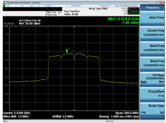
Plot 7-556. PSD CDD Antenna 3b (80MHz BW 802.11ac – Ch. 106, MCS3)
