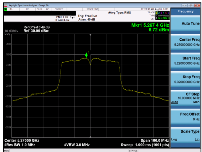
Plot 7-504. PSD SDM Antenna 3b (40MHz BW 802.11n – Ch. 54, MCS10)
