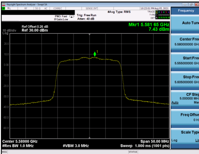
Plot 7-549. PSD CDD Antenna 5T (20MHz BW 802.11ax(SU) – Ch. 116, MCS3)
