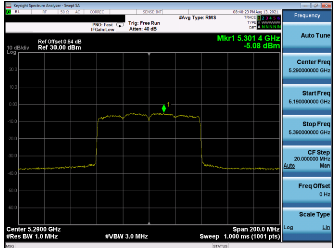
Plot 7-545. PSD CDD Antenna 5T (80MHz BW 802.11ax(SU) – Ch. 58, MCS3)
