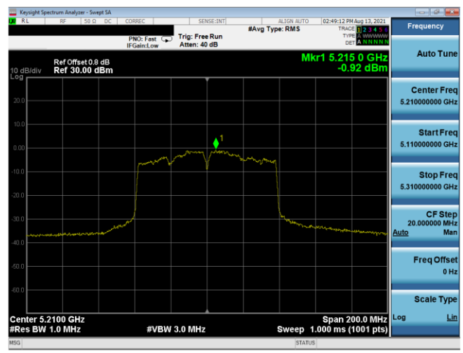
Plot 7-496. PSD CDD Antenna 3b (80MHz BW 802.11ac – Ch. 42, MCS2)
