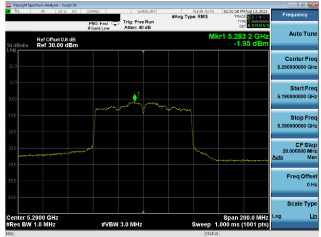
Plot 7-508. PSD CDD Antenna 3b (80MHz BW 802.11ac - Ch. 58, MCS2)
