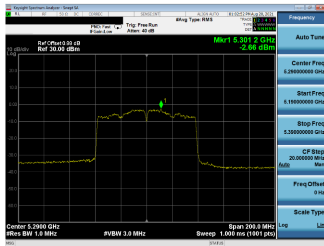
Plot 7-543. PSD CDD Antenna 5T (80MHz BW 802.11ac – Ch. 58, MCS3)
