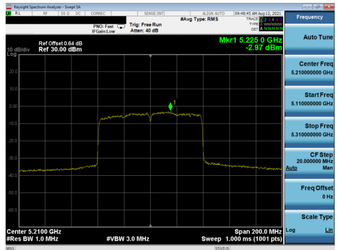
Plot 7-533. PSD CDD Antenna 5T (80MHz BW 802.11ax(SU) – Ch. 42, MCS3)
