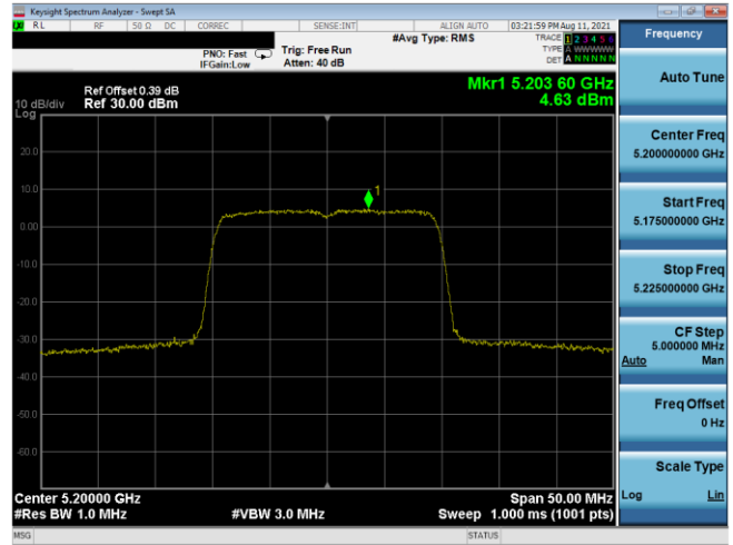
Plot 7-562. PSD SDM Antenna 3b (20MHz BW 802.11ax(SU) – Ch. 40, MCS5)
