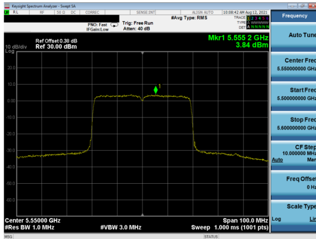
Plot 7-554. PSD CDD Antenna 3b (40MHz BW 802.11ax(SU) – Ch. 110, MCS3)
