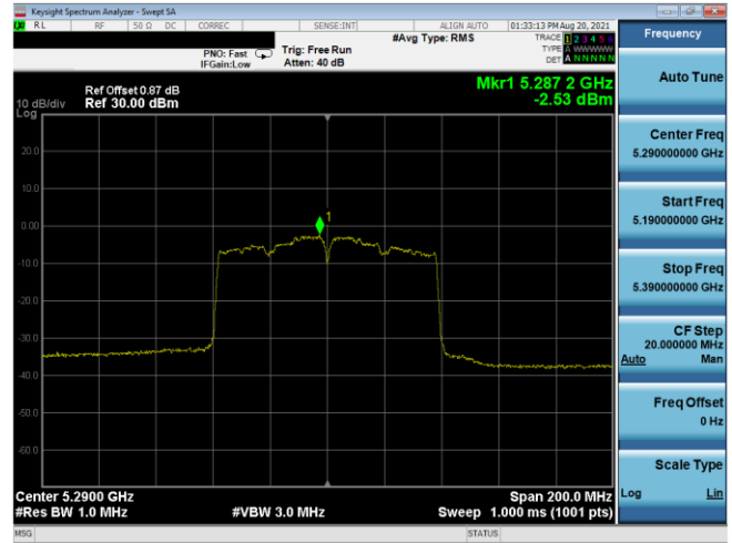
Plot 7-544. PSD CDD Antenna 3b (80MHz BW 802.11ac – Ch. 58, MCS3)
