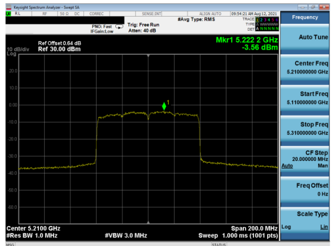
Plot 7-534. PSD CDD Antenna 3b (80MHz BW 802.11ax(SU) – Ch. 42, MCS3)
