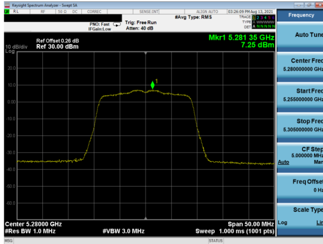
Plot 7-499. PSD SDM Antenna 5T (20MHz BW 802.11n – Ch. 56, MCS10)
