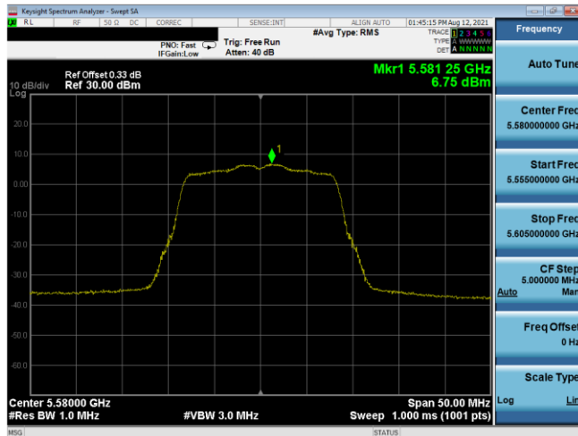
Plot 7-548. PSD CDD Antenna 3b (20MHz BW 802.11n – Ch. 116, MCS11)
