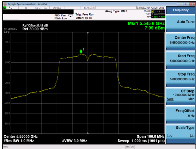
Plot 7-515. PSD CDD Antenna 5T (40MHz BW 802.11n – Ch. 110, MCS10)
