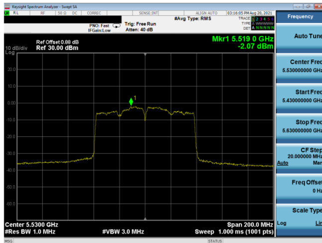
Plot 7-555. PSD CDD Antenna 5T (80MHz BW 802.11ac – Ch. 106, MCS3)
