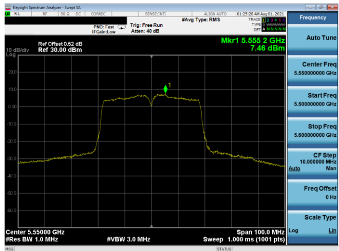
Plot 7-551. PSD CDD Antenna 5T (40MHz BW 802.11n – Ch. 110, MCS11)
