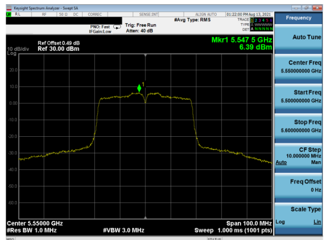
Plot 7-516. PSD CDD Antenna 3b (40MHz BW 802.11n – Ch. 110, MCS10)
