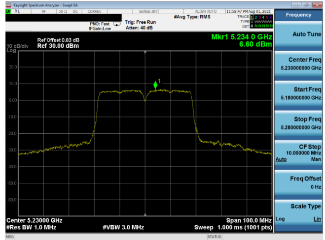
Plot 7-563. PSD SDM Antenna 5T (40MHz BW 802.11n – Ch. 46, MCS13)
