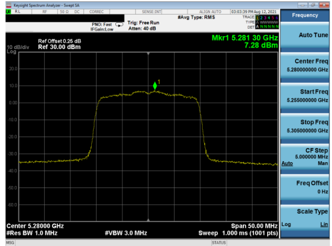
Plot 7-538. PSD SDM Antenna 3b (20MHz BW 802.11ax(SU) – Ch. 56, MCS3)
