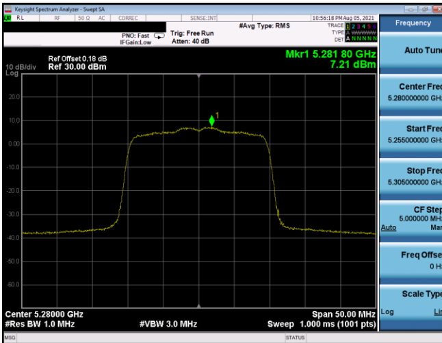
Plot 7-501. PSD SDM Antenna 5T (20MHz BW 802.11ax(SU) – Ch. 56, MCS2)
