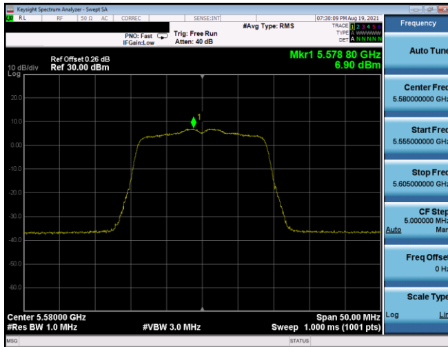
Plot 7-511. PSD CDD Antenna 5T (20MHz BW 802.11n – Ch. 116, MCS10)
