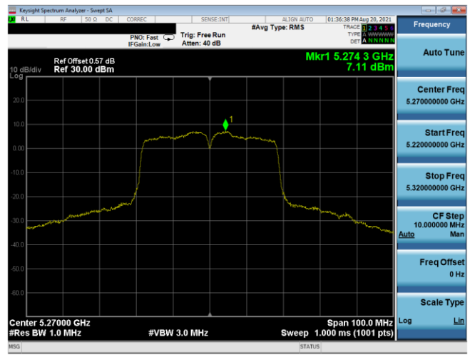
Plot 7-540. PSD SDM Antenna 3b (40MHz BW 802.11n – Ch. 54, MCS11)
