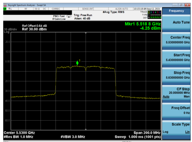
Plot 7-558. PSD CDD Antenna 3b (80MHz BW 802.11ax(SU) – Ch. 106, MCS3)
