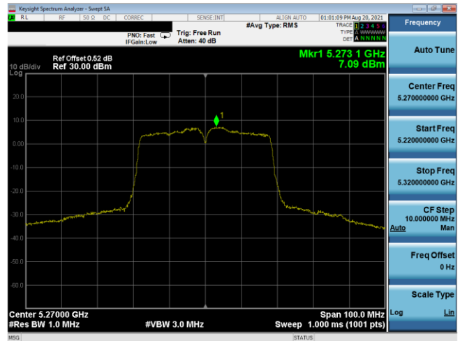
Plot 7-539. PSD SDM Antenna 5T (40MHz BW 802.11n – Ch. 54, MCS11)
