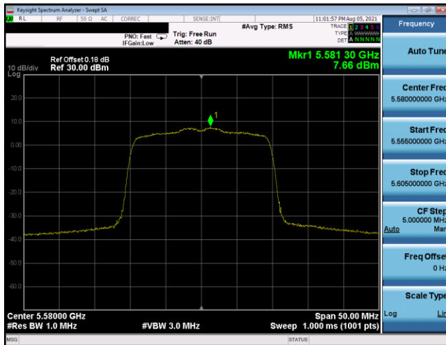
Plot 7-513. PSD CDD Antenna 5T (20MHz BW 802.11ax(SU) – Ch. 116, MCS2)
