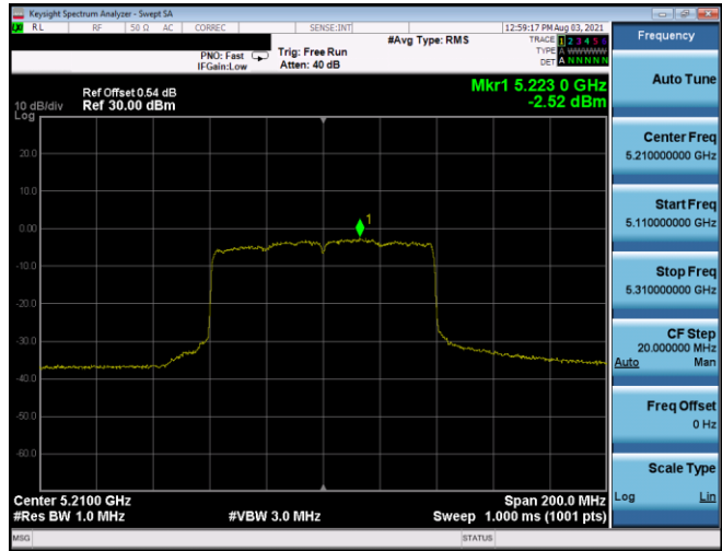
Plot 7-497. PSD CDD Antenna 5T (80MHz BW 802.11ax(SU) – Ch. 42, MCS2)
