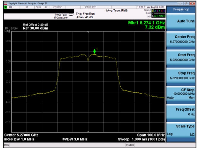
Plot 7-503. PSD SDM Antenna 5T (40MHz BW 802.11n – Ch. 54, MCS10)
