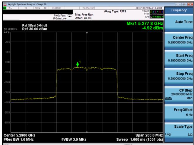
Plot 7-546. PSD CDD Antenna 3b (80MHz BW 802.11ax(SU) – Ch. 58, MCS3)
