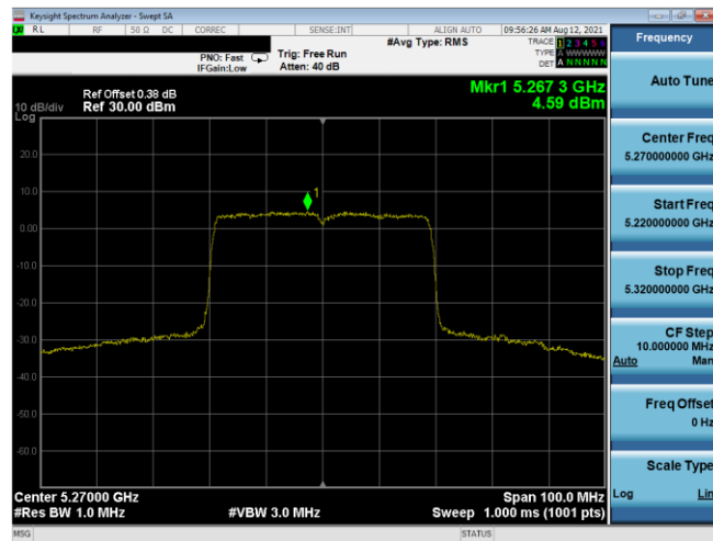
Plot 7-542. PSD SDM Antenna 3b (40MHz BW 802.11ax(SU) – Ch. 54, MCS3)
