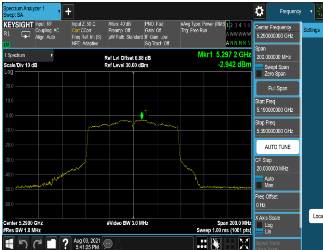
Plot 7-507. PSD CDD Antenna 5T (80MHz BW 802.11ac - Ch. 58, MCS2)
