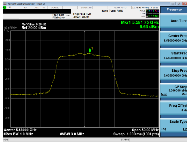
Plot 7-512. PSD CDD Antenna 3b (20MHz BW 802.11n – Ch. 116, MCS10)
