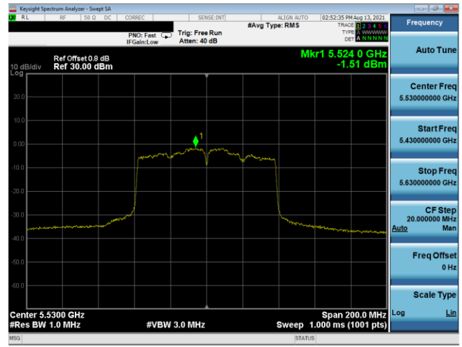
Plot 7-520. PSD CDD Antenna 3b (80MHz BW 802.11ac – Ch. 106, MCS2)
