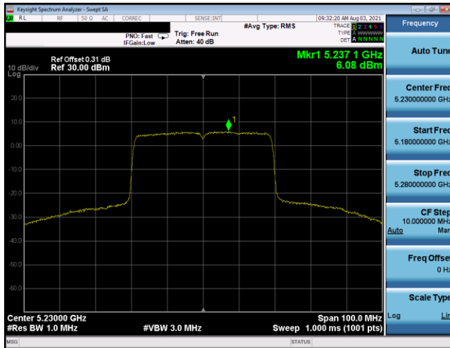
Plot 7-493. PSD SDM Antenna 5T (40MHz BW 802.11ax(SU) – Ch. 46, MCS2)
