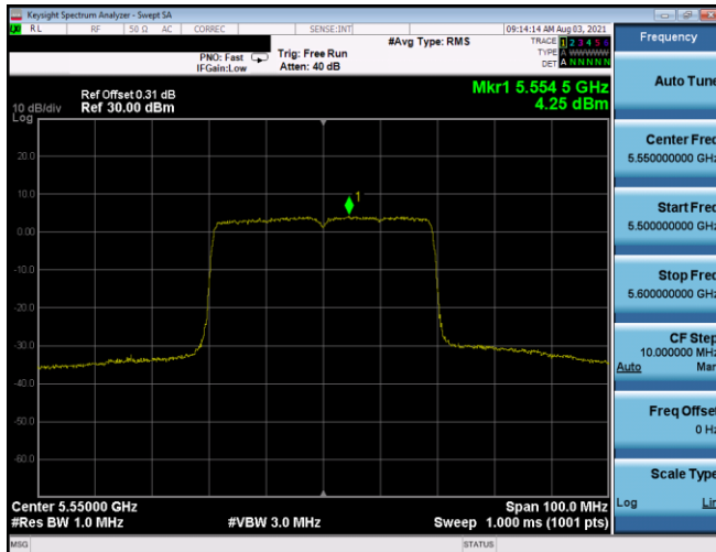
Plot 7-517. PSD CDD Antenna 5T (40MHz BW 802.11ax(SU) – Ch. 110, MCS2)
