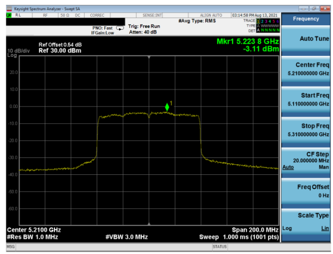
Plot 7-498. PSD CDD Antenna 3b (80MHz BW 802.11ax(SU) – Ch. 42, MCS2)
