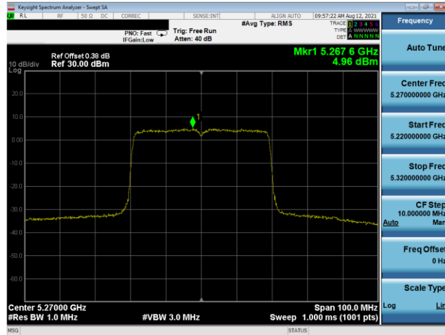
Plot 7-505. PSD SDM Antenna 5T (40MHz BW 802.11ax(SU) - Ch. 54, MCS2)
