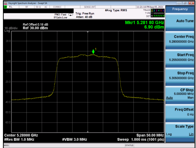
Plot 7-502. PSD SDM Antenna 3b (20MHz BW 802.11ax(SU) – Ch. 56, MCS2)
