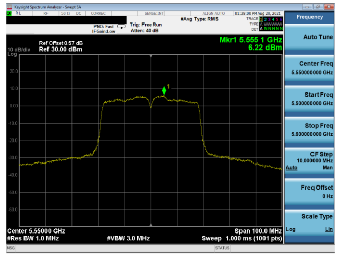
Plot 7-552. PSD CDD Antenna 3b (40MHz BW 802.11n – Ch. 110, MCS11)
