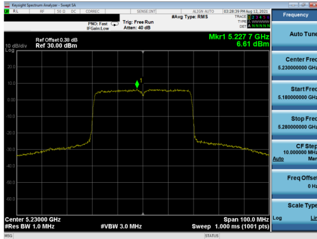
Plot 7-529. PSD SDM Antenna 5T (40MHz BW 802.11ax(SU) – Ch. 46, MCS3)
