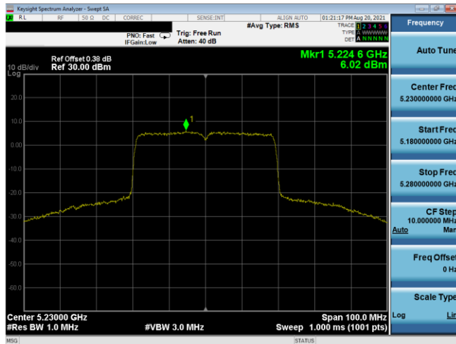
Plot 7-530. PSD SDM Antenna 3b (40MHz BW 802.11ax(SU) – Ch. 46, MCS3)
