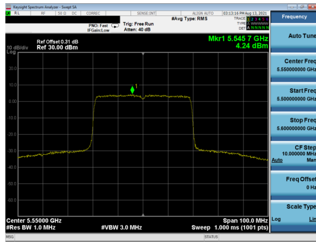
Plot 7-518. PSD CDD Antenna 3b (40MHz BW 802.11ax(SU) – Ch. 110, MCS2)
