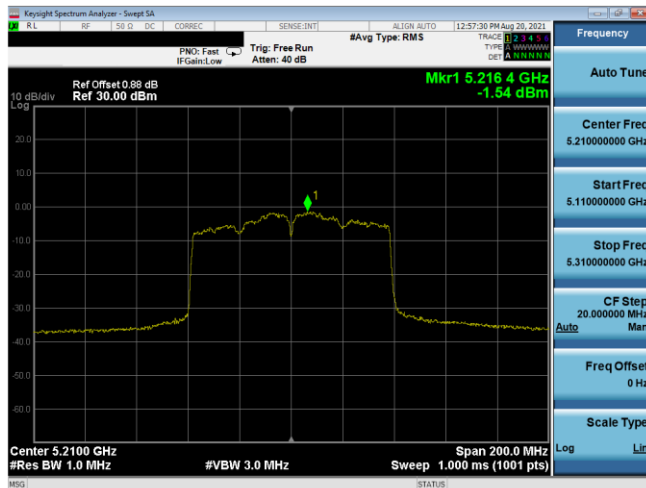
Plot 7-531. PSD CDD Antenna 5T (80MHz BW 802.11ac – Ch. 42, MCS3)
