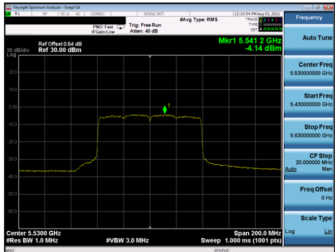
Plot 7-522. PSD CDD Antenna 3b (80MHz BW 802.11ax(SU) – Ch. 106, MCS2)
