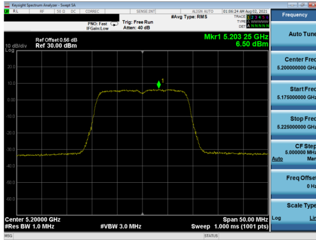
Plot 7-559. PSD SDM Antenna 5T (20MHz BW 802.11n – Ch. 40, MCS13)
