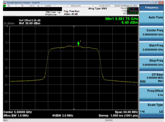
Plot 7-550. PSD CDD Antenna 3b (20MHz BW 802.11ax(SU) – Ch. 116, MCS3)
