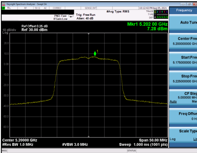
Plot 7-525. PSD SDM Antenna 5T (20MHz BW 802.11ax(SU) - Ch. 40, MCS3)
