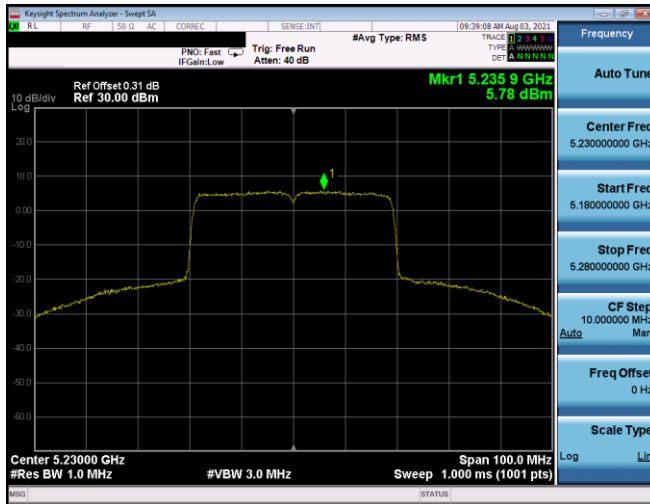
Plot 7-494. PSD SDM Antenna 3b (40MHz BW 802.11ax(SU) – Ch. 46, MCS2)
