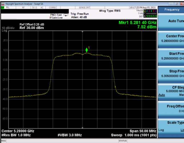
Plot 7-537. PSD SDM Antenna 5T (20MHz BW 802.11ax(SU) – Ch. 56, MCS3)
