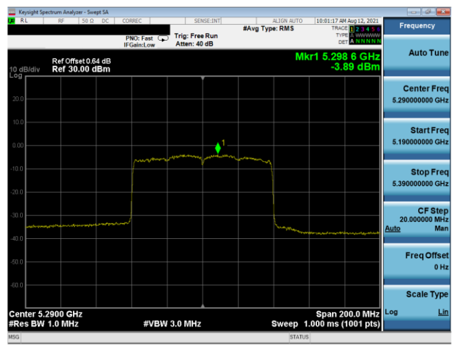
Plot 7-509. PSD CDD Antenna 5T (80MHz BW 802.11ax(SU) - Ch. 58, MCS2)
