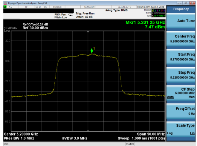
Plot 7-526. PSD SDM Antenna 3b (20MHz BW 802.11ax(SU) - Ch. 40, MCS3)
