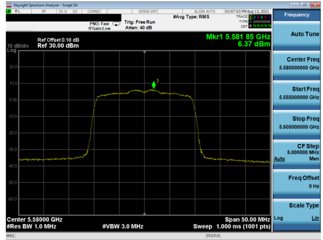
Plot 7-514. PSD CDD Antenna 3b (20MHz BW 802.11ax(SU) – Ch. 116, MCS2)
