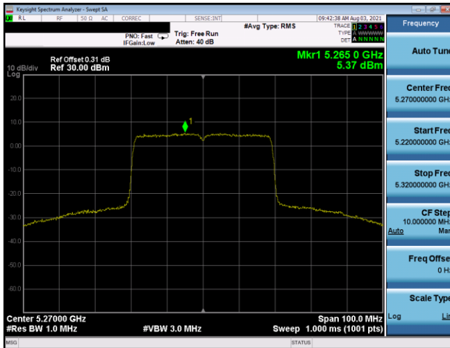
Plot 7-506. PSD SDM Antenna 3b (40MHz BW 802.11ax(SU) - Ch. 54, MCS2)
