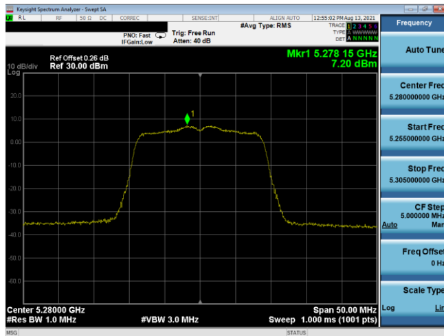
Plot 7-500. PSD SDM Antenna 3b (20MHz BW 802.11n – Ch. 56, MCS10)
