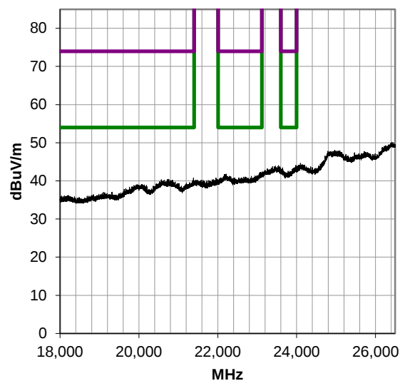
18000-26500 MHz, Run 32
