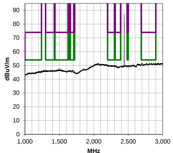
1000-3000 MHz, Run 5
