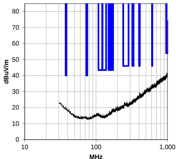
30-1000 MHz, Run 25
