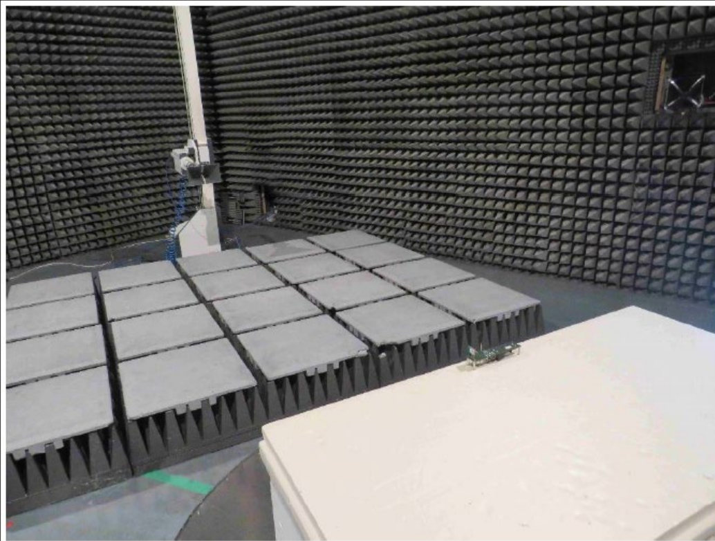
TEST SETUP – 1 GHz to 6 GHz - CONFIGURATION 1
