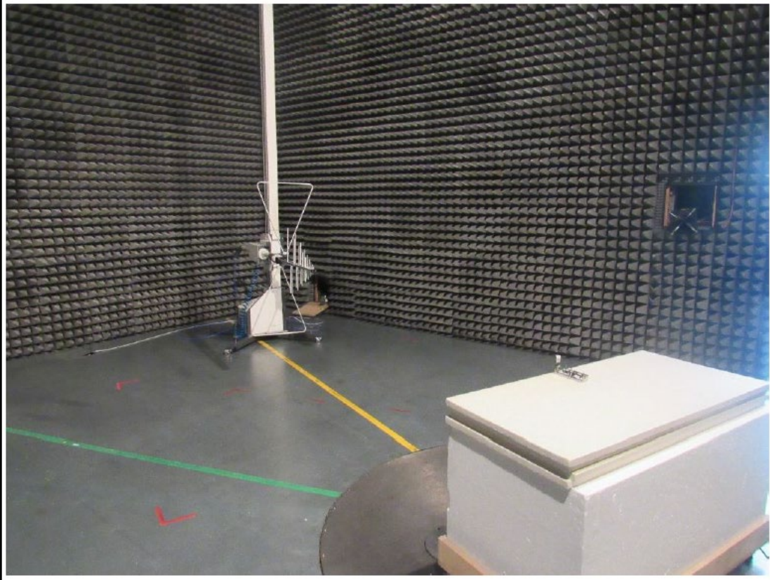
Setup for measurements below 1 GHz
