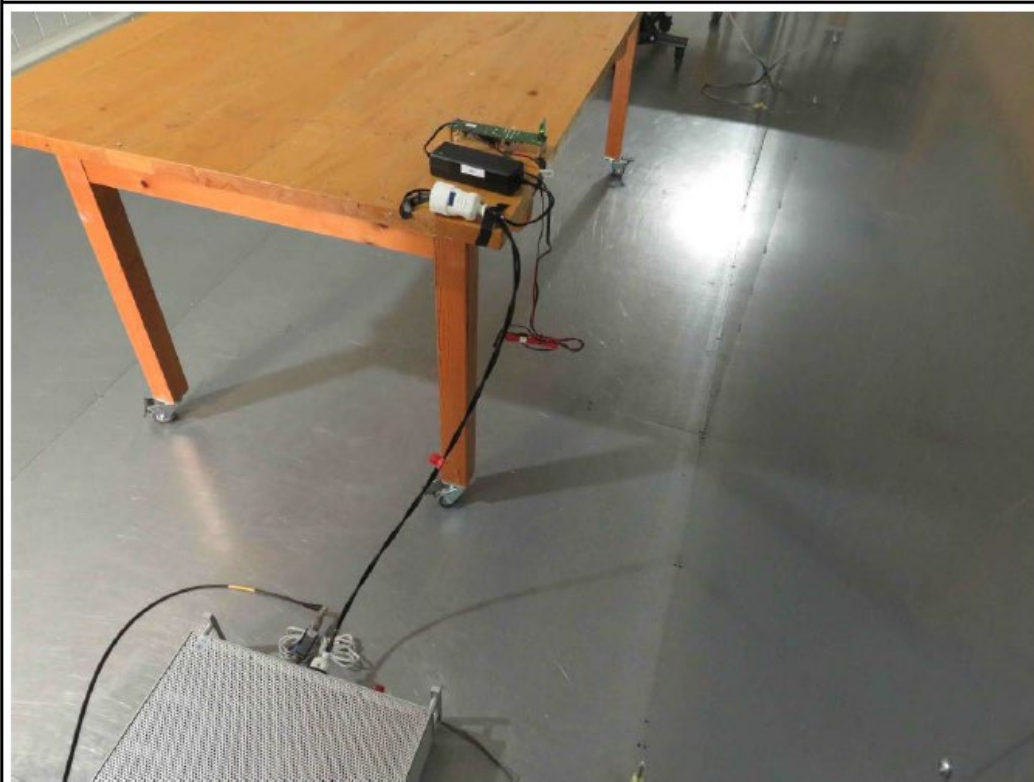
TEST SETUP – POWER – CONFIGURATION 2
