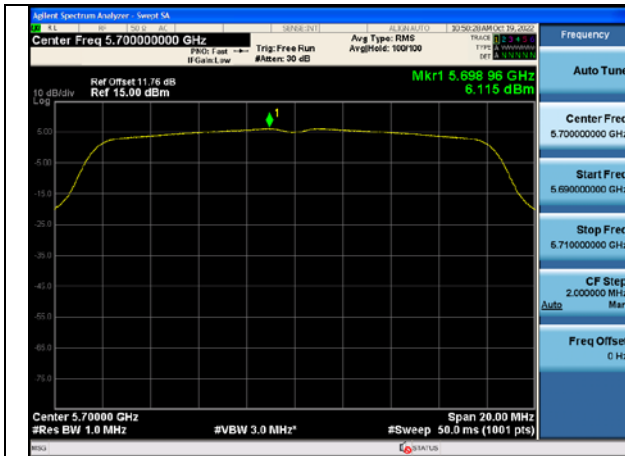
Test Mode:802.11a 5700MHz Chain0
