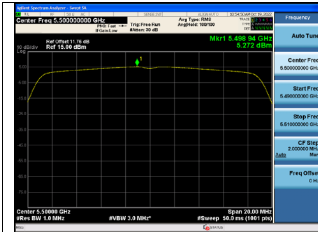
Test Mode:802.11n HT20 5500MHz Chain0
