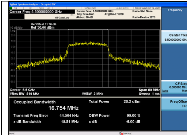
Test Mode:802.11a 5500MHz Chain0
